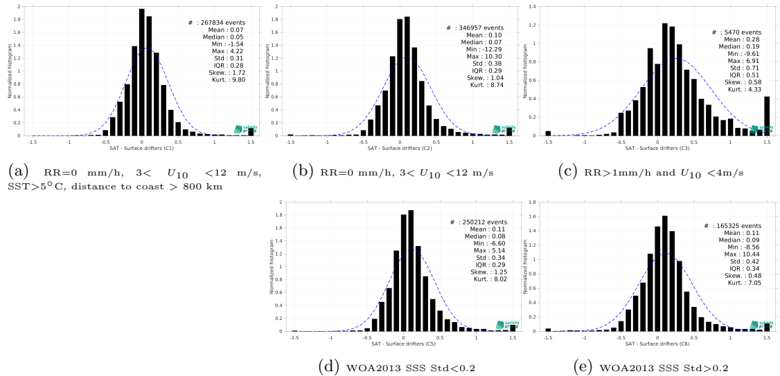
Figure 14: Normalized histogram of \Delta SSS (SMAP SSS L3 v5.0 - Monthly (JPL) - Surface drifters) for 5 different subdatasets corresponding to: RR=0 mm/h, 3 < U_{10} < 12 m/s, SST >5^\circ\text{C} , distance to coast > 800 km (a), RR=0 mm/h, 3 < U_{10} < 12 m/s (b), RR >1 mm/h and U_{10} < 4 m/s (c), WOA2013 SSS Std <0.2 (d), WOA2013 SSS Std >0.2 (e).
