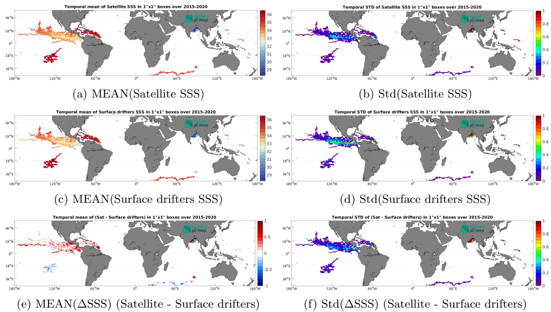
Figure 6: Temporal mean (left) and Std (right) of SSS from SMAP SSS L3 v5.0 - Monthly (JPL) (top), Surface drifters (middle), and of \Delta SSS (Satellite - Surface drifters). Only match-up pairs are used to generate these maps.
