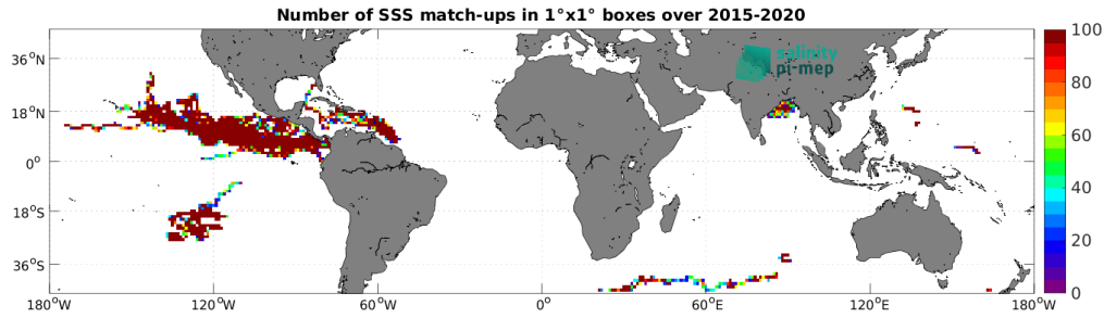
Figure 4: Number of SSS match-ups between Surface drifters SSS and the SMAP SSS L3 v5.0 - Monthly (JPL) SSS product for the Mid-Low Latitudes 45N-45S Pi-MEP region over 1^\circ \times 1^\circ boxes and for the full satellite product period.
