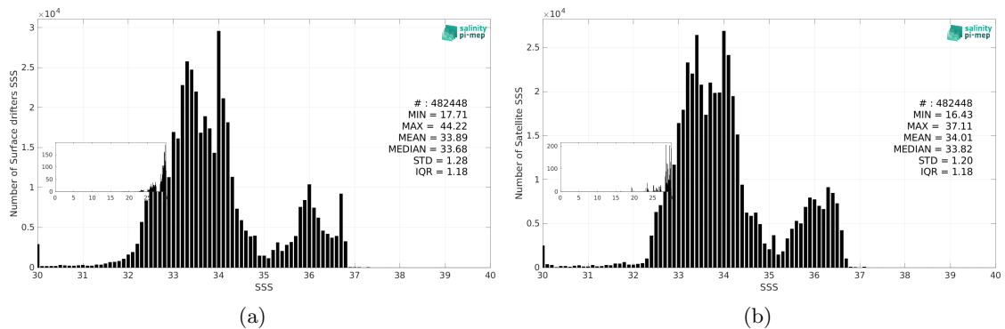
Figure 3: Histograms of SSS from Surface drifters (a) and SMAP SSS L3 v5.0 - Monthly (JPL) (b) considering all match-up pairs per bins of 0.1 over the Mid-Low Latitudes 45N-45S Pi-MEP region and for the full satellite product period.
