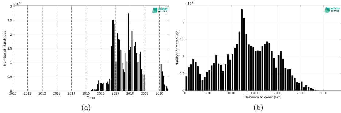
Figure 2: Number of match-ups between Surface drifters and SMAP SSS L3 v5.0 - Monthly (JPL) SSS as a function of time (a) and as function of the distance to coast (b) over the Mid-Low Latitudes 45N-45S Pi-MEP region and for the full satellite product period.
