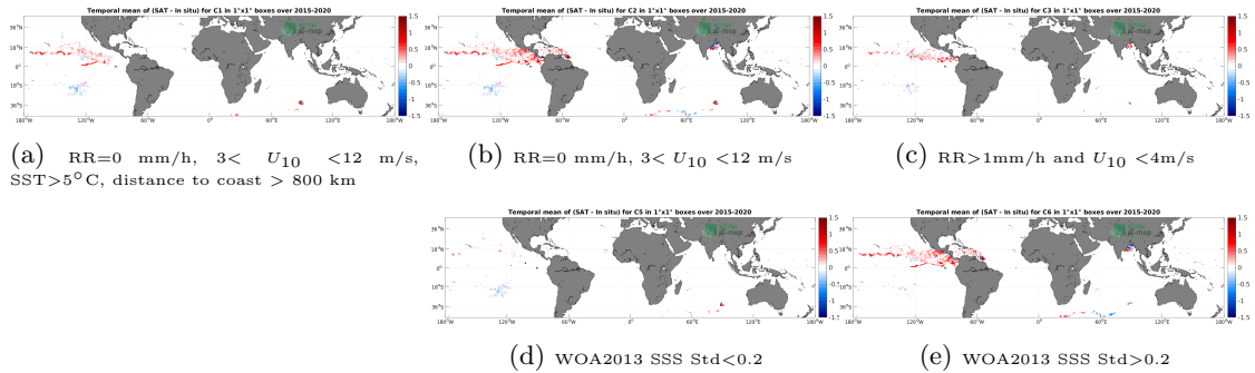
Figure 11: Temporal mean gridded over spatial boxes of size 1^\circ \times 1^\circ of \Delta SSS (SMAP SSS L3 v5.0 - Monthly (JPL) - Surface drifters) for 5 different subdatasets corresponding to:RR=0 mm/h, 3 < U_{10} < 12 m/s, SST > 5^\circ C , distance to coast > 800 km (a), RR=0 mm/h, 3 < U_{10} < 12 m/s (b), RR>1mm/h and U_{10} < 4 m/s (c), WOA2013 SSS Std<0.2 (d), WOA2013 SSS Std>0.2 (e).
