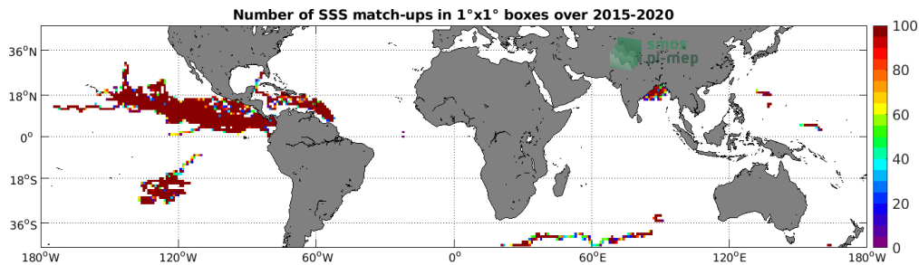
Figure 3: Number of SSS match-ups between Surface drifters SSS and the SMAP SSS L3 v5.0 - Monthly (JPL) SSS product for the Mid-Low Latitudes 45N-45S Pi-MEP region over 1^\circ \times 1^\circ boxes and for the full satellite product period.
