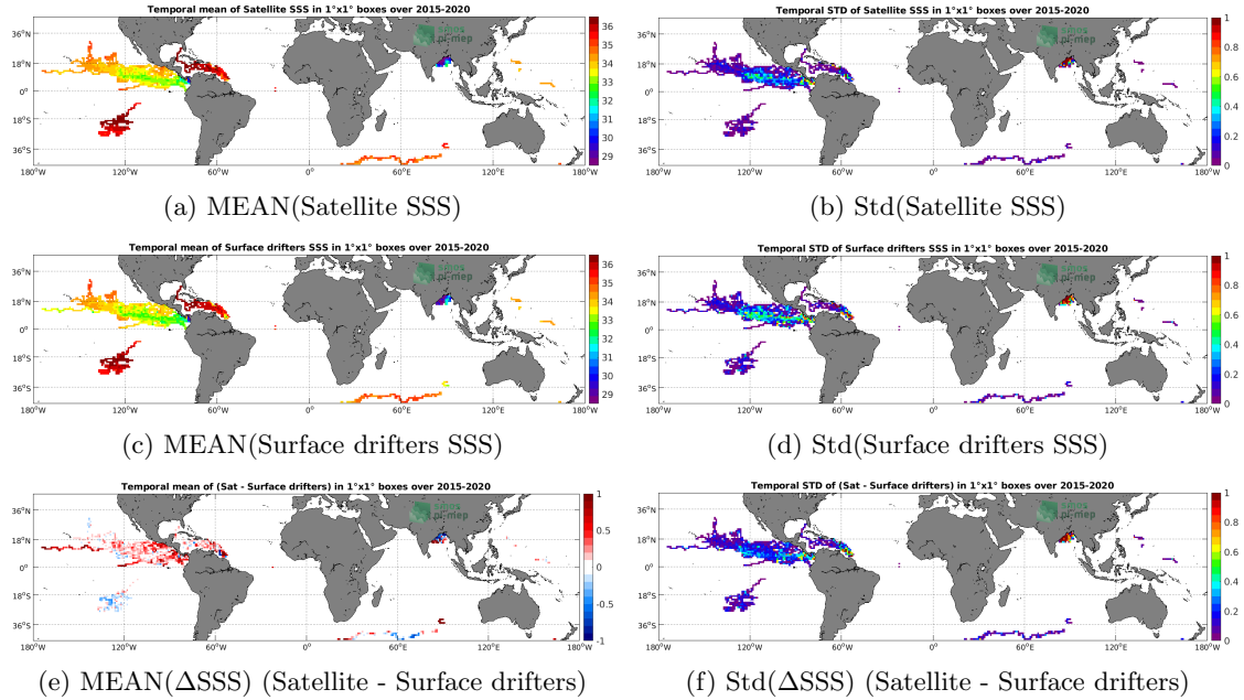
Figure 5: Temporal mean (left) and Std (right) of SSS from SMAP SSS L3 v5.0 - Monthly (JPL) (top), Surface drifters (middle), and of \Delta SSS (Satellite - Surface drifters). Only match-up pairs are used to generate these maps.
