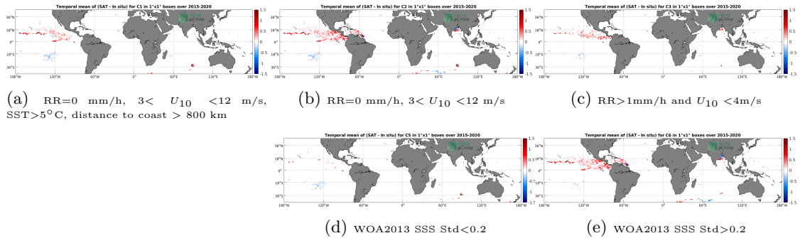
Figure 11: Temporal mean gridded over spatial boxes of size 1^\circ \times 1^\circ of \Delta SSS (SMAP SSS L3 v5.0 - Monthly (JPL) - Surface drifters) for 5 different subdatasets corresponding to: RR=0 mm/h, 3 < U_{10} < 12 m/s, SST>5°C, distance to coast > 800 km (a), RR=0 mm/h, 3 < U_{10} < 12 m/s (b), RR>1mm/h and U_{10} < 4 m/s (c), WOA2013 SSS Std<0.2 (d), WOA2013 SSS Std>0.2 (e).
