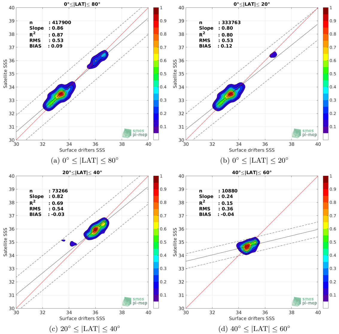
Figure 8: Contour maps of the concentration of SMAP-L3-JPL-V4.3-MONTHLY-60KM SSS (y-axis) versus Surface drifters SSS (x-axis) at match-up pairs for different latitudinal bands. For each plot, the red line shows x=y . The black thin and dashed lines indicate a linear fit through the data cloud and the \pm 95\% confidence levels, respectively. The number match-up pairs n , the slope and R^2 coefficient of the linear fit, the root mean square (RMS) and the mean bias between satellite and in situ data are indicated for each latitude band in each plots.
