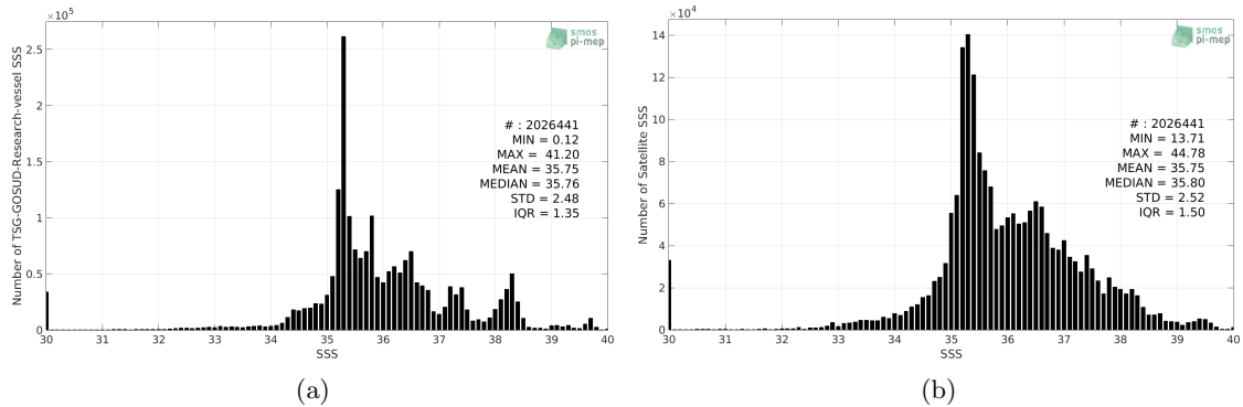
Figure 2: Histograms of SSS from TSG-GOSUD-Research-vessel (a) and SMAP-L3-JPL-V4.2-8DAY-RUNNING-60KM (b) considering all match-up pairs per bins of 0.1 over the Mid-Low Latitudes 45N-45S Pi-MEP region and for the full satellite product period.
