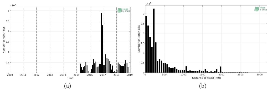
Figure 1: Number of match-ups between TSG-GOSUD-Research-vessel and SMAP-L3-JPL-V4.2-8DAY-RUNNING-60KM SSS as a function of time (a) and as function of the distance to coast (b) over the Mid-Low Latitudes 45N-45S Pi-MEP region and for the full satellite product period.
