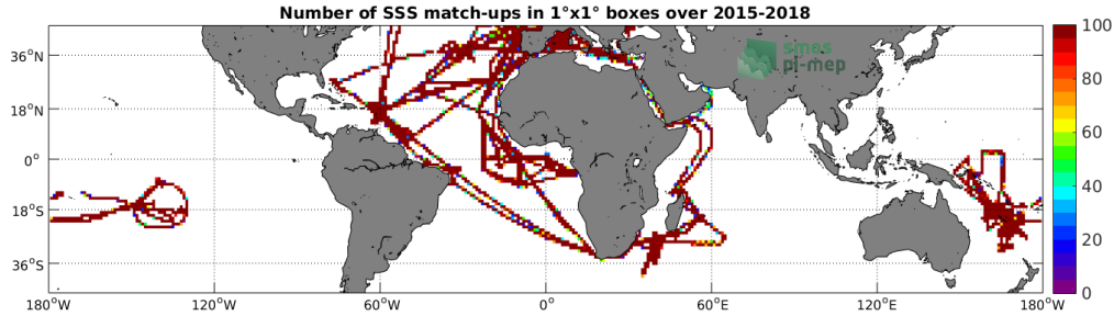
Figure 4: Number of SSS match-ups between TSG-GOSUD-Research-vessel SSS and the SMAP-L3-JPL-V4.2-8DAY-RUNNING-60KM SSS product for the Mid-Low Latitudes 45N-45S Pi-MEP region over 1^\circ \times 1^\circ boxes and for the full satellite product period.
