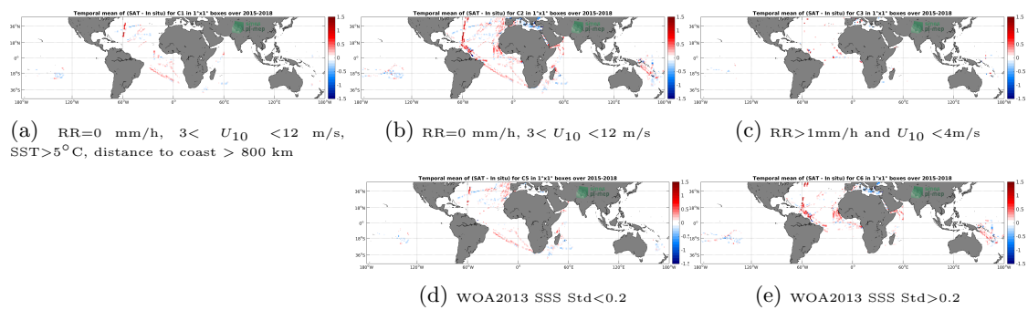
Figure 12: Temporal mean gridded over spatial boxes of size 1^\circ \times 1^\circ of \Delta SSS (SMAP-L3-JPL-V4.2-8DAY-RUNNING-60KM - TSG-GOSUD-Research-vessel) for 5 different subdatasets corresponding to:RR=0 mm/h, 3 < U_{10} < 12 m/s, SST >5^\circ\text{C} , distance to coast > 800 km (a), RR=0 mm/h, 3 < U_{10} < 12 m/s (b), RR >1 mm/h and U_{10} < 4 m/s (c), WOA2013 SSS Std <0.2 (d), WOA2013 SSS Std >0.2 (e).
