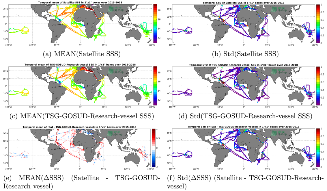
Figure 6: Temporal mean (left) and Std (right) of SSS from SMAP-L3-JPL-V4.2-8DAY-RUNNING-60KM (top), TSG-GOSUD-Research-vessel (middle), and of \Delta SSS (Satellite - TSG-GOSUD-Research-vessel). Only match-up pairs are used to generate these maps.
