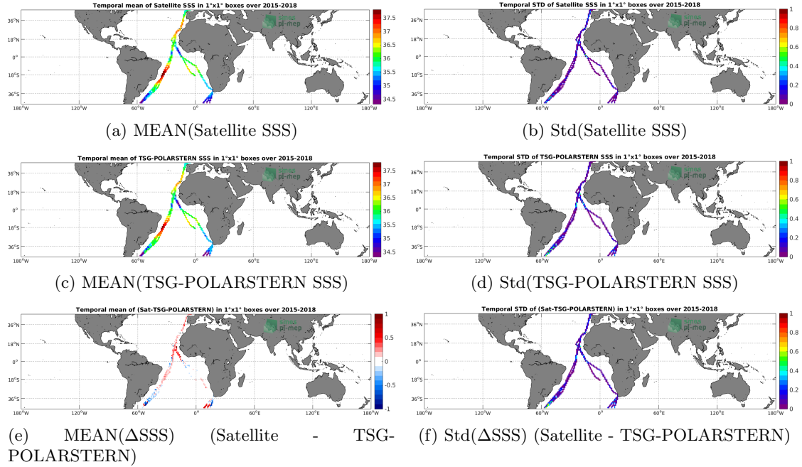
Figure 6: Temporal mean (left) and Std (right) of SSS from SMAP-L3-JPL-V4.2-MONTHLY-60KM (top), TSG-POLARSTERN (middle), and of \Delta SSS (Satellite - TSG-POLARSTERN). Only match-up pairs are used to generate these maps.
