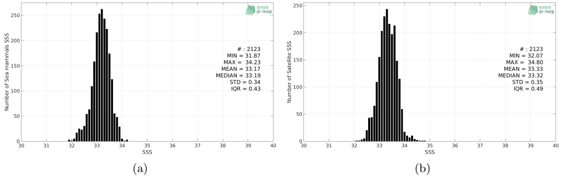
Figure 2: Histograms of SSS from Sea mammals (a) and SMAP-L3-JPL-V4.2-MONTHLY-60KM (b) considering all match-up pairs per bins of 0.1 over the Mid-Low Latitudes 45N-45S Pi-MEP region and for the full satellite product period.
