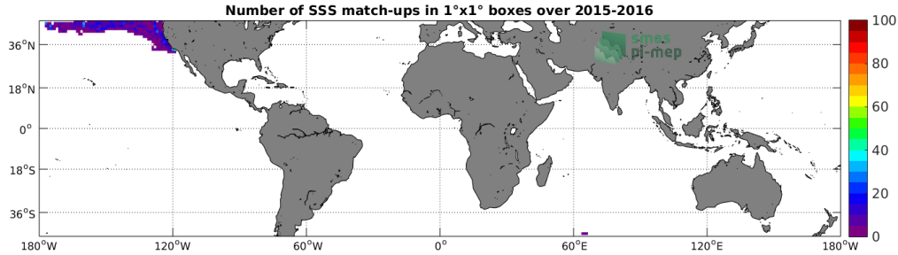
Figure 4: Number of SSS match-ups between Sea mammals SSS and the SMAP-L3-JPL-V4.2-MONTHLY-60KM SSS product for the Mid-Low Latitudes 45N-45S Pi-MEP region over 1^\circ \times 1^\circ boxes and for the full satellite product period.
