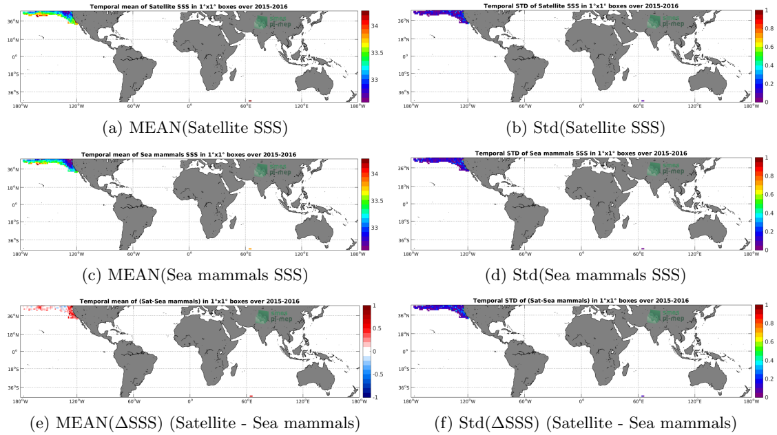
Figure 6: Temporal mean (left) and Std (right) of SSS from SMAP-L3-JPL-V4.2-MONTHLY-60KM (top), Sea mammals (middle), and of \Delta SSS (Satellite - Sea mammals). Only match-up pairs are used to generate these maps.
