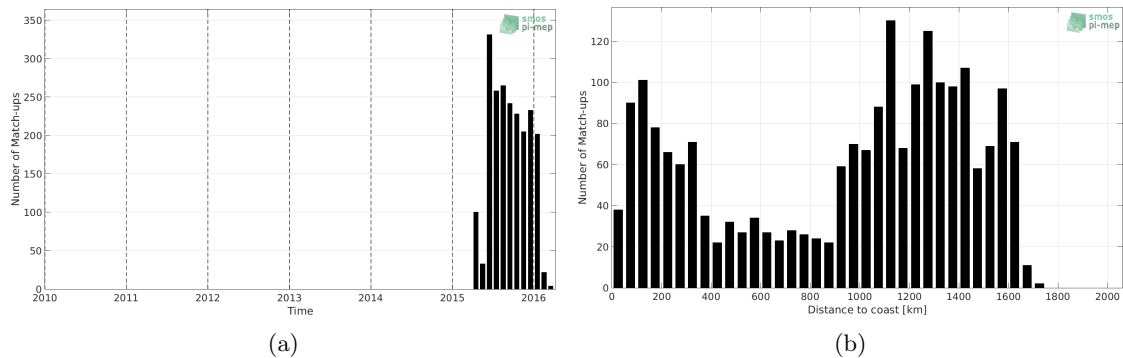
Figure 1: Number of match-ups between Sea mammals and SMAP-L3-JPL-V4.2-MONTHLY-60KM SSS as a function of time (a) and as function of the distance to coast (b) over the Mid-Low Latitudes 45N-45S Pi-MEP region and for the full satellite product period.
