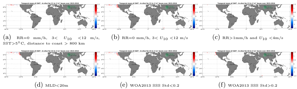
Figure 12: Temporal mean gridded over spatial boxes of size 1^\circ \times 1^\circ of \Delta SSS (SMAP-L3-JPL-V4.2-MONTHLY-60KM - Sea mammals) for 6 different subdatasets corresponding to:RR=0 mm/h, 3 < U_{10} < 12 m/s, SST >5^\circ C, distance to coast > 800 km (a), RR=0 mm/h, 3 < U_{10} < 12 m/s (b), RR >1 mm/h and U_{10} < 4 m/s (c),MLD <20 m (d),WOA2013 SSS Std <0.2 (e),WOA2013 SSS Std >0.2 (f).
