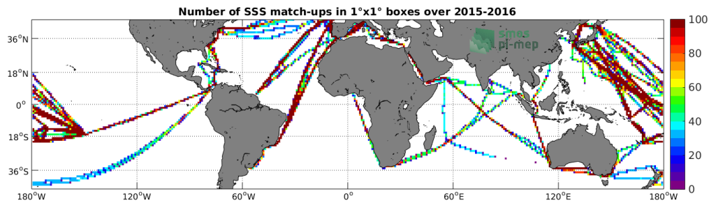
Figure 4: Number of SSS match-ups between TSG-LEGOS-DM SSS and the SMAP-L3-JPL-V4-8DAY-RUNNING-60KM SSS product for the Mid-Low Latitudes 45N-45S Pi-MEP region over 1^\circ \times 1^\circ boxes and for the full satellite product period.
