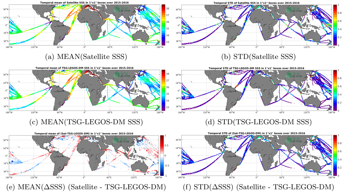
Figure 6: Temporal mean (left) and STD (right) of SSS from SMAP-L3-JPL-V4-8DAY-RUNNING-60KM (top), TSG-LEGOS-DM (middle), and of \Delta SSS (Satellite - TSG-LEGOS-DM). Only match-up pairs are used to generate these maps.
