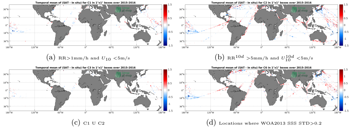
Figure 12: Temporal mean gridded over spatial boxes of size 1^\circ \times 1^\circ of \Delta SSS (SMAP-L3-JPL-V4-8DAY-RUNNING-60KM - TSG-LEGOS-DM) for 4 different subdatasets corresponding to: RR > 1\text{mm/h} and U_{10} < 5\text{m/s} (a), RR^{10d} > 5\text{mm/h} and U_{10}^{10d} < 5\text{m/s} (b), C1 U C2 (c), Locations where WOA2013 SSS STD > 0.2 (d).
