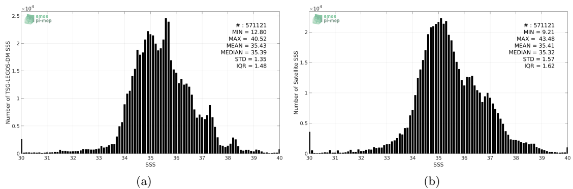
Figure 2: Histograms of SSS from TSG-LEGOS-DM (a) and SMAP-L3-JPL-V4-8DAY-RUNNING-60KM (b) considering all match-up pairs per bins of 0.1 over the Mid-Low Latitudes 45N-45S Pi-MEP region and for the full satellite product period.
