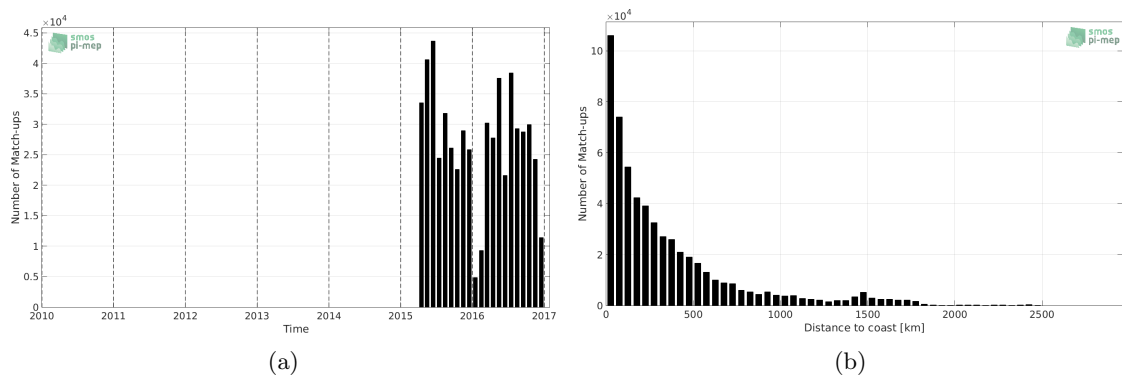
Figure 1: Number of match-ups between TSG-LEGOS-DM and SMAP-L3-JPL-V4-8DAY-RUNNING-60KM SSS as a function of time (a) and as function of the distance to coast (b) over the Mid-Low Latitudes 45N-45S Pi-MEP region and for the full satellite product period.
