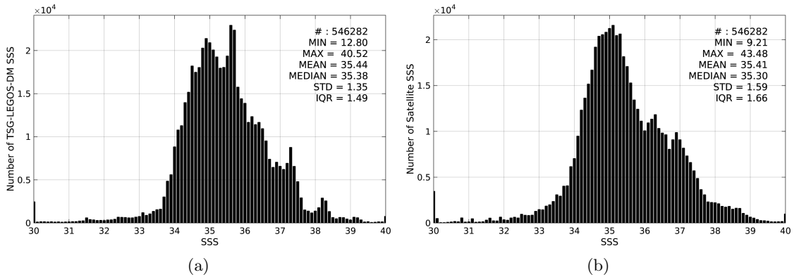
Figure 2: Histograms of SSS from TSG-LEGOS-DM (a) and SMAP-L3-JPL-V4-8DAY-RUNNING-60KM (b) considering all match-up pairs per bins of 0.1 over the Mid-Low Latitudes 45N-45S Pi-MEP region and for the full satellite product period.
