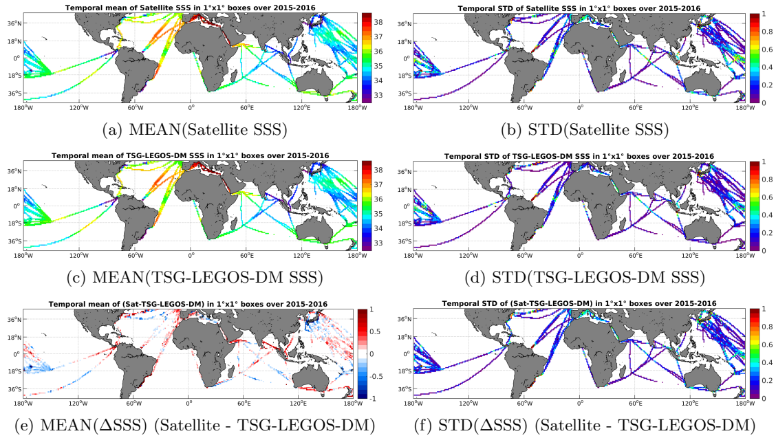
Figure 6: Temporal mean (left) and STD (right) of SSS from SMAP-L3-JPL-V4-8DAY-RUNNING-60KM (top), TSG-LEGOS-DM (middle), and of \Delta SSS (Satellite - TSG-LEGOS-DM). Only match-up pairs are used to generate these maps.
