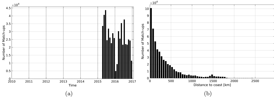
Figure 1: Number of match-ups between TSG-LEGOS-DM and SMAP-L3-JPL-V4-8DAY-RUNNING-60KM SSS as a function of time (a) and as function of the distance to coast (b) over the Mid-Low Latitudes 45N-45S Pi-MEP region and for the full satellite product period.
