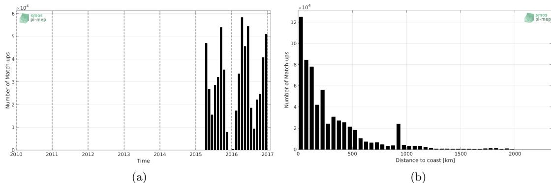
Figure 1: Number of match-ups between TSG-GOSUD-Research-vessel and SMAP-L3-JPL-V4-8DAY-RUNNING-60KM SSS as a function of time (a) and as function of the distance to coast (b) over the Mid-Low Latitudes 45N-45S Pi-MEP region and for the full satellite product period.
