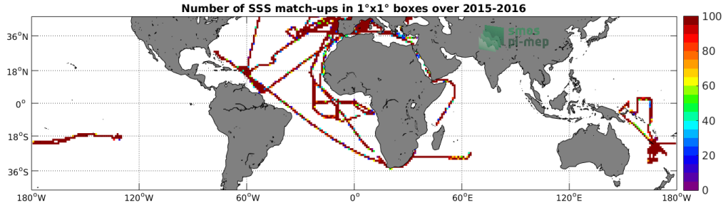
Figure 4: Number of SSS match-ups between TSG-GOSUD-Research-vessel SSS and the SMAP-L3-JPL-V4-8DAY-RUNNING-60KM SSS product for the Mid-Low Latitudes 45N-45S Pi-MEP region over 1^\circ \times 1^\circ boxes and for the full satellite product period.
