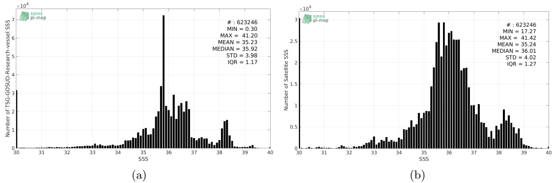
Figure 2: Histograms of SSS from TSG-GOSUD-Research-vessel (a) and SMAP-L3-JPL-V4-8DAY-RUNNING-60KM (b) considering all match-up pairs per bins of 0.1 over the Mid-Low Latitudes 45N-45S Pi-MEP region and for the full satellite product period.
