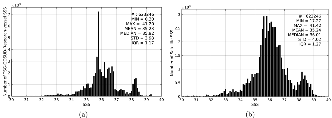
Figure 2: Histograms of SSS from TSG-GOSUD-Research-vessel (a) and SMAP-L3-JPL-V4-8DAY-RUNNING-60KM (b) considering all match-up pairs per bins of 0.1 over the Mid-Low Latitudes 45N-45S Pi-MEP region and for the full satellite product period.
