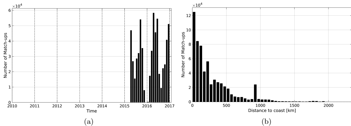
Figure 1: Number of match-ups between TSG-GOSUD-Research-vessel and SMAP-L3-JPL-V4-8DAY-RUNNING-60KM SSS as a function of time (a) and as function of the distance to coast (b) over the Mid-Low Latitudes 45N-45S Pi-MEP region and for the full satellite product period.
