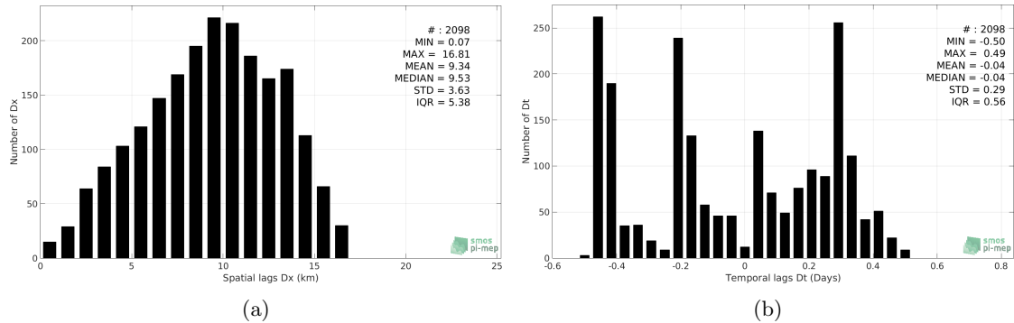
Figure 5: Histograms of the spatial (a) and temporal (b) lags between the time of the Sea mammals measurements and the date of the corresponding SMAP-L3-JPL-V4-8DAY-RUNNING-60KM SSS product.
