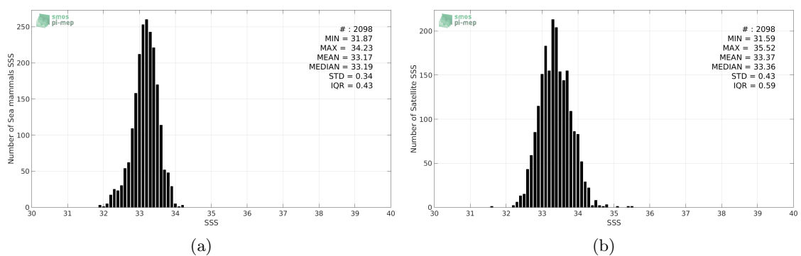
Figure 2: Histograms of SSS from Sea mammals (a) and SMAP-L3-JPL-V4-8DAY-RUNNING-60KM (b) considering all match-up pairs per bins of 0.1 over the Mid-Low Latitudes 45N-45S Pi-MEP region and for the full satellite product period.
