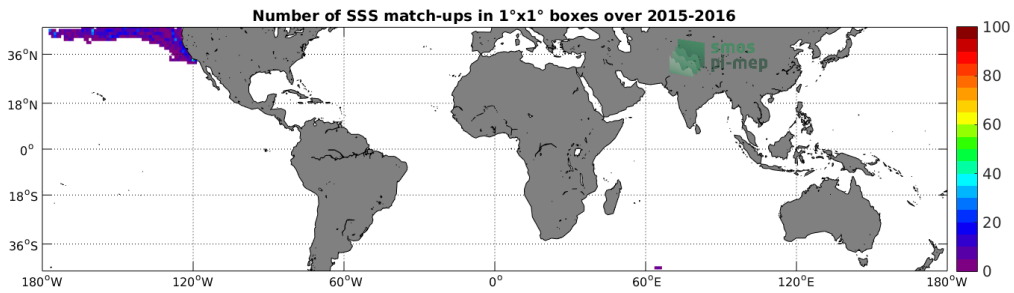
Figure 4: Number of SSS match-ups between Sea mammals SSS and the SMAP-L3-JPL-V4-8DAY-RUNNING-60KM SSS product for the Mid-Low Latitudes 45N-45S Pi-MEP region over 1^\circ \times 1^\circ boxes and for the full satellite product period.
