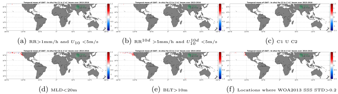
Figure 12: Temporal mean gridded over spatial boxes of size 1°x1° of \Delta SSS (SMAP-L3-JPL-V4-8DAY-RUNNING-60KM - Sea mammals) for 6 different subdatasets corresponding to:RR>1mm/h and U_{10} < 5m/s (a), RR^{10d} > 5mm/h and U_{10}^{10d} < 5m/s (b), C1 U C2 (c),MLD<20m (d),BLT>10m (e),Locations where WOA2013 SSS STD>0.2 (f).
