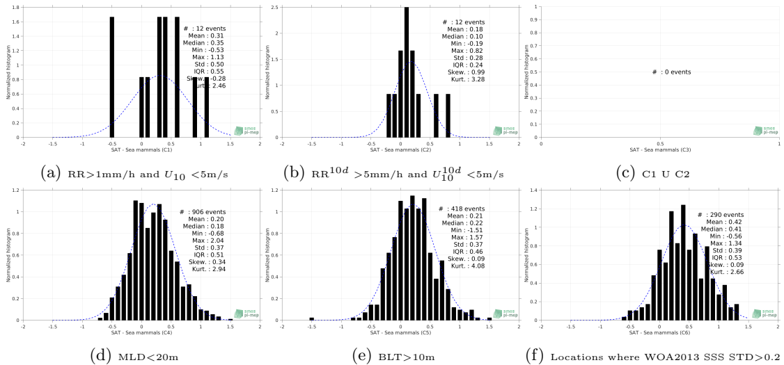
Figure 13: Normalized histogram of \Delta SSS (SMAP-L3-JPL-V4-8DAY-RUNNING-60KM - Sea mammals) for 6 different subdatasets corresponding to: RR>1mm/h and U_{10} < 5m/s (a), RR^{10d} > 5mm/h and U_{10}^{10d} < 5m/s (b), C1 U C2 (c),MLD<20m (d),BLT>10m (e),Locations where WOA2013 SSS STD>0.2 (f).
