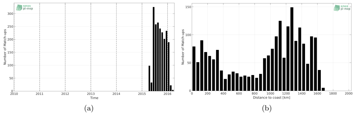
Figure 1: Number of match-ups between Sea mammals and SMAP-L3-JPL-V4-8DAY-RUNNING-60KM SSS as a function of time (a) and as function of the distance to coast (b) over the Mid-Low Latitudes 45N-45S Pi-MEP region and for the full satellite product period.
