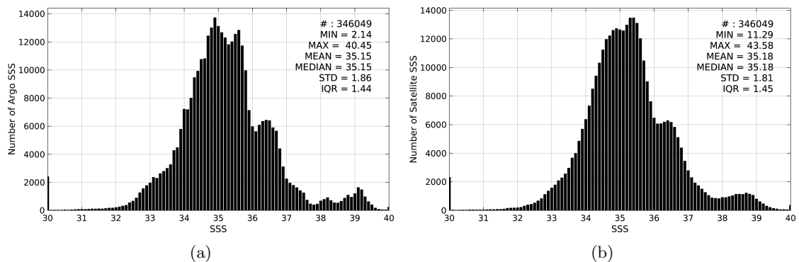
Figure 2: Histograms of SSS from Argo (a) and SMAP-L3-JPL-V4-8DAY-RUNNING-60KM (b) considering all match-up pairs per bins of 0.1 over the Mid-Low Latitudes 45N-45S Pi-MEP region and for the full satellite product period.
