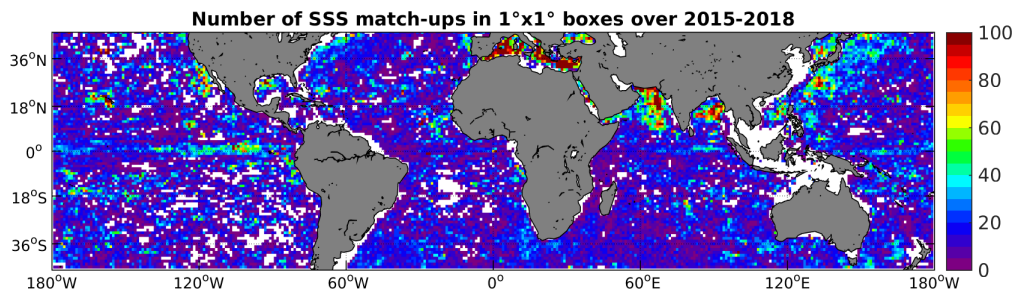
Figure 4: Number of SSS match-ups between Argo SSS and the SMAP-L3-JPL-V4-8DAY-RUNNING-60KM SSS product for the Mid-Low Latitudes 45N-45S Pi-MEP region over 1^\circ \times 1^\circ boxes and for the full satellite product period.
