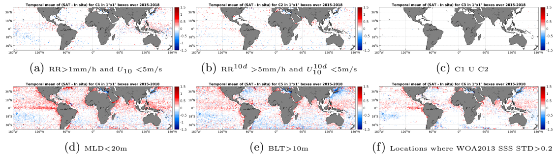
Figure 12: Temporal mean gridded over spatial boxes of size 1^\circ \times 1^\circ of \Delta SSS (SMAP-L3-JPL-V4-8DAY-RUNNING-60KM - Argo) for 6 different subdatasets corresponding to: RR>1mm/h and U_{10} < 5\text{m/s} (a), RR^{10d} > 5\text{mm/h} and U_{10}^{10d} < 5\text{m/s} (b), C1 U C2 (c),MLD<20m (d),BLT>10m (e),Locations where WOA2013 SSS STD>0.2 (f).
