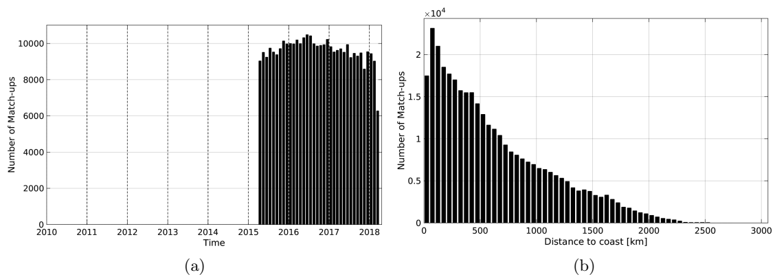
Figure 1: Number of match-ups between Argo and SMAP-L3-JPL-V4-8DAY-RUNNING-60KM SSS as a function of time (a) and as function of the distance to coast (b) over the Mid-Low Latitudes 45N-45S Pi-MEP region and for the full satellite product period.
