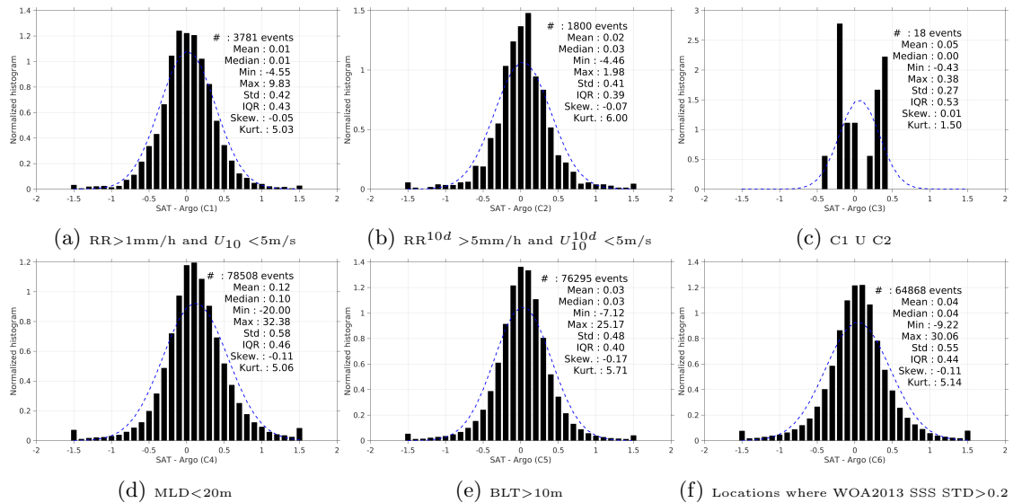
Figure 13: Normalized histogram of \Delta SSS (SMAP-L3-JPL-V4-8DAY-RUNNING-60KM - Argo) for 6 different subdatasets corresponding to: RR>1mm/h and U_{10} < 5\text{m/s} (a), RR^{10d} > 5\text{mm/h} and U_{10}^{10d} < 5\text{m/s} (b), C1 U C2 (c),MLD<20m (d),BLT>10m (e),Locations where WOA2013 SSS STD>0.2 (f).
