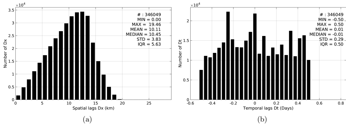
Figure 5: Histograms of the spatial (a) and temporal (b) lags between the time of the Argo measurements and the date of the corresponding SMAP-L3-JPL-V4-8DAY-RUNNING-60KM SSS product.
