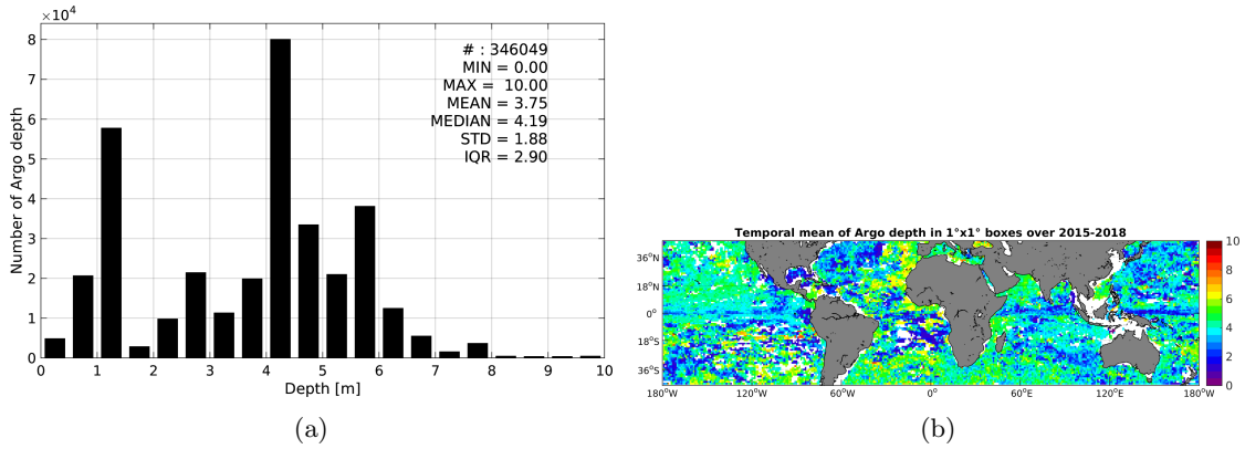
Figure 3: Histograms of the depth of the upper level SSS measurements from Argo in the Match-up DataBase for the Mid-Low Latitudes 45N-45S Pi-MEP region (a) and temporal mean spatial distribution of pressure of the in situ SSS data over 1^\circ \times 1^\circ boxes and for the full satellite product period (b).
