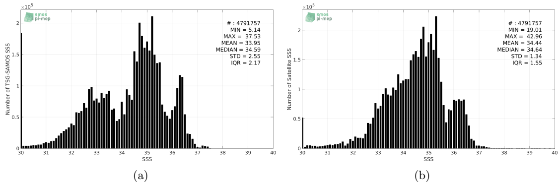
Figure 2: Histograms of SSS from TSG-SAMOS (a) and SMAP-L3-JPL-V4-MONTHLY-60KM (b) considering all match-up pairs per bins of 0.1 over the Mid-Low Latitudes 45N-45S Pi-MEP region and for the full satellite product period.
