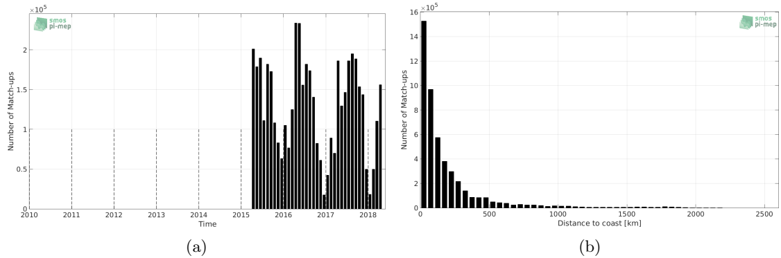
Figure 1: Number of match-ups between TSG-SAMOS and SMAP-L3-JPL-V4-MONTHLY-60KM SSS as a function of time (a) and as function of the distance to coast (b) over the Mid-Low Latitudes 45N-45S Pi-MEP region and for the full satellite product period.
