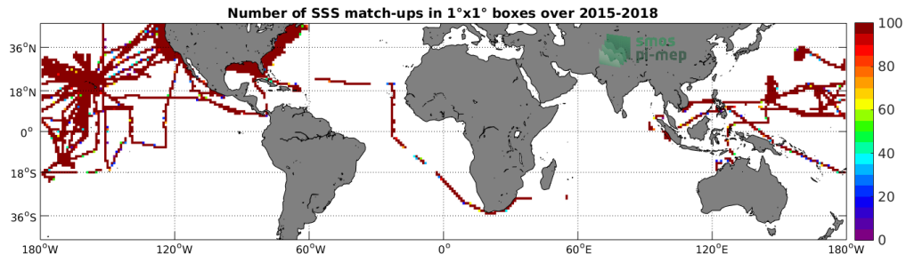
Figure 4: Number of SSS match-ups between TSG-SAMOS SSS and the SMAP-L3-JPL-V4-MONTHLY-60KM SSS product for the Mid-Low Latitudes 45N-45S Pi-MEP region over 1^\circ \times 1^\circ boxes and for the full satellite product period.
