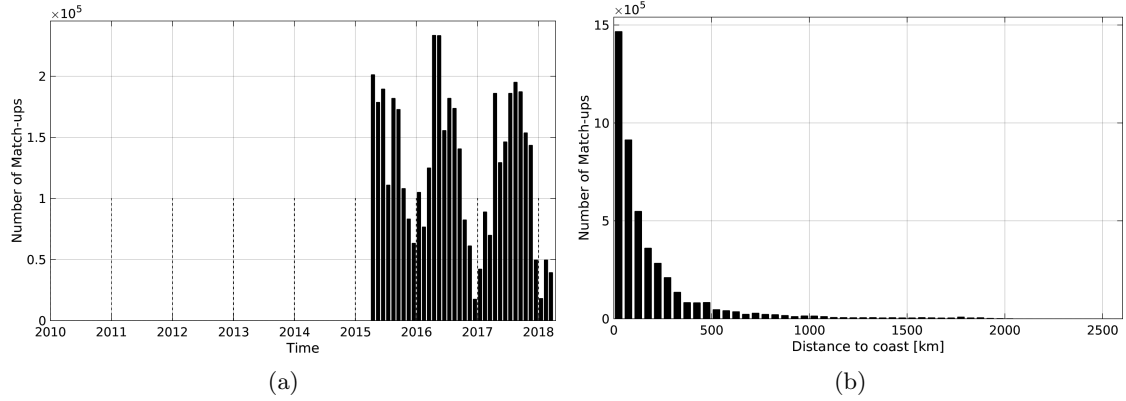
Figure 1: Number of match-ups between TSG-SAMOS and SMAP-L3-JPL-V4-MONTHLY-60KM SSS as a function of time (a) and as function of the distance to coast (b) over the Mid-Low Latitudes 45N-45S Pi-MEP region and for the full satellite product period.
