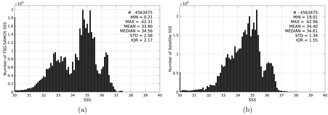
Figure 2: Histograms of SSS from TSG-SAMOS (a) and SMAP-L3-JPL-V4-MONTHLY-60KM (b) considering all match-up pairs per bins of 0.1 over the Mid-Low Latitudes 45N-45S Pi-MEP region and for the full satellite product period.
