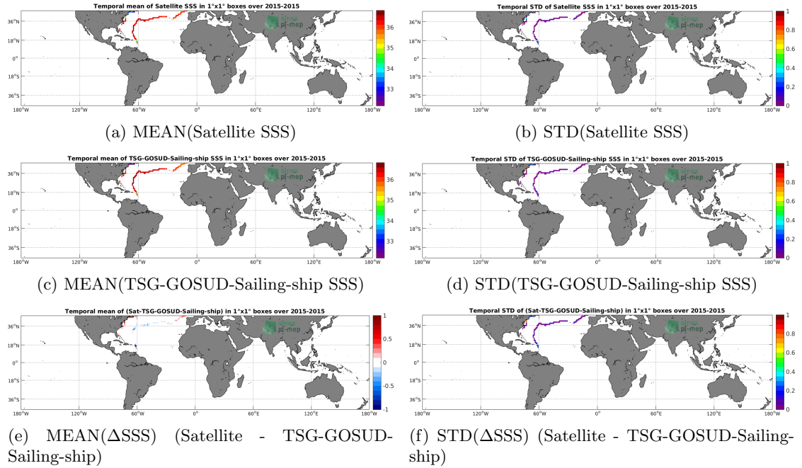
Figure 6: Temporal mean (left) and STD (right) of SSS from SMAP-L3-JPL-V4-MONTHLY-60KM (top), TSG-GOSUD-Sailing-ship (middle), and of \Delta SSS (Satellite - TSG-GOSUD-Sailing-ship). Only match-up pairs are used to generate these maps.
