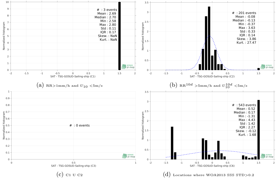
Figure 13: Normalized histogram of \Delta\text{SSS} (SMAP-L3-JPL-V4-MONTHLY-60KM - TSG-GOSUD-Sailing-ship) for 6 different subdatasets corresponding to: RR > 1\text{mm/h} and U_{10} < 5\text{m/s} (a), RR^{10d} > 5\text{mm/h} and U_{10}^{10d} < 5\text{m/s} (b), C1 U C2 (c), Locations where WOA2013 SSS STD > 0.2 (d).
