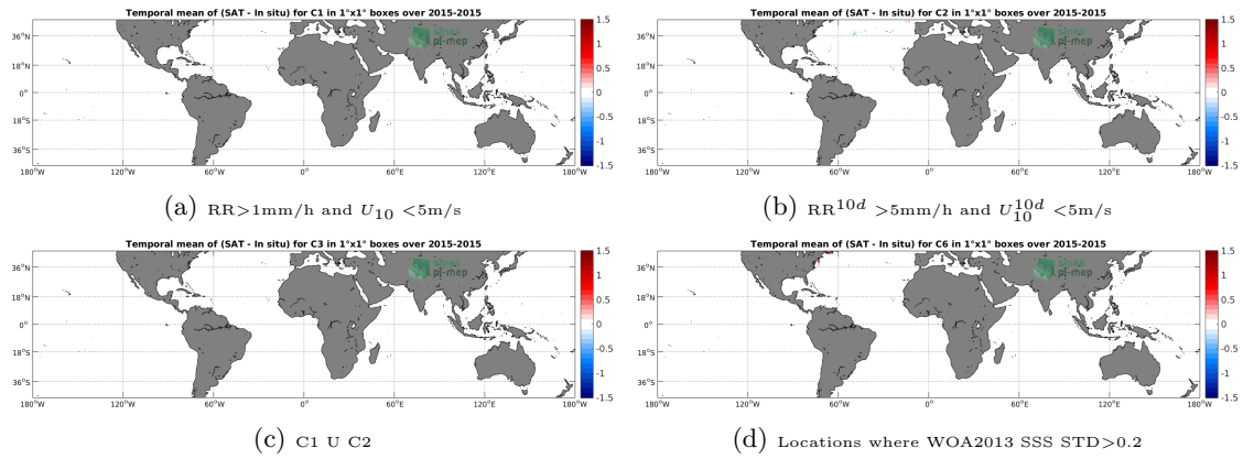
Figure 12: Temporal mean gridded over spatial boxes of size 1^\circ \times 1^\circ of \Delta SSS (SMAP-L3-JPL-V4-MONTHLY-60KM - TSG-GOSUD-Sailing-ship) for 4 different subdatasets corresponding to: RR > 1\text{mm/h} and U_{10} < 5\text{m/s} (a), RR^{10d} > 5\text{mm/h} and U_{10}^{10d} < 5\text{m/s} (b), C1 U C2 (c), Locations where WOA2013 SSS STD > 0.2 (d).
