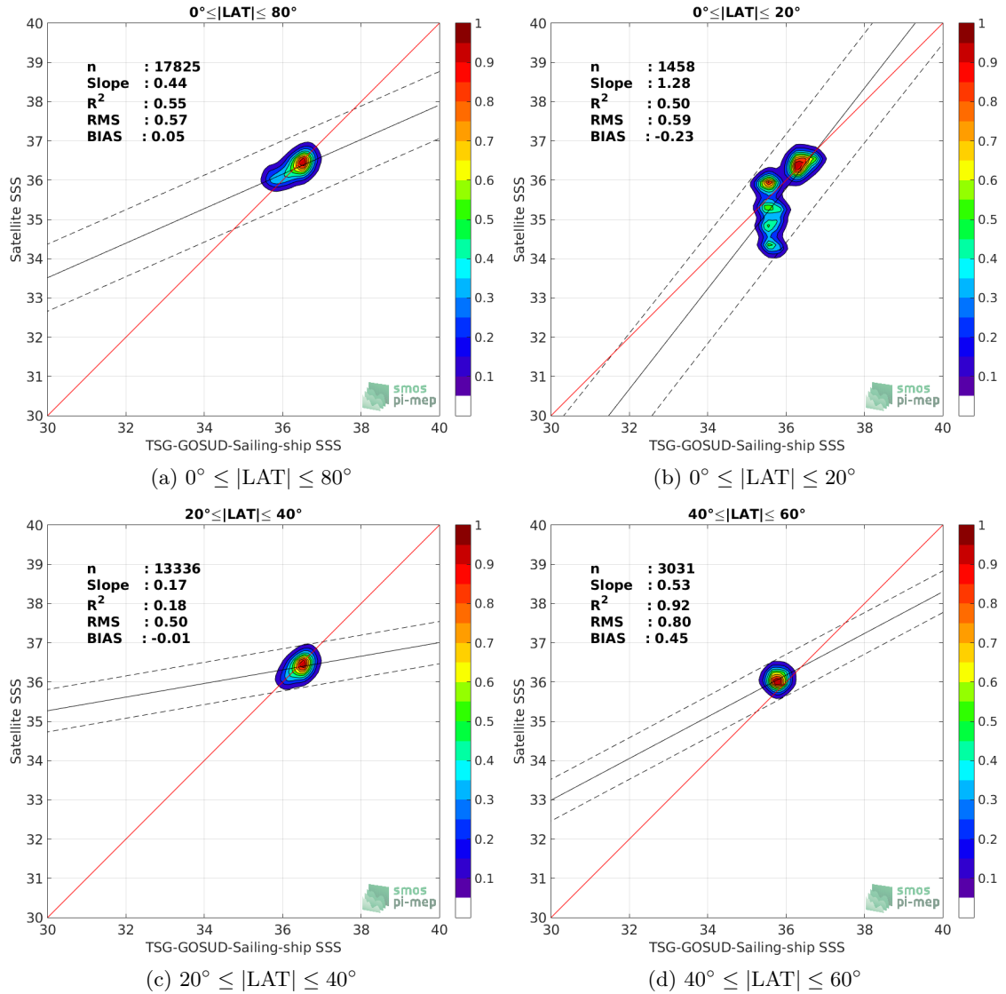
Figure 9: Contour maps of the concentration of SMAP-L3-JPL-V4-MONTHLY-60KM SSS (y-axis) versus TSG-GOSUD-Sailing-ship SSS (x-axis) at match-up pairs for different latitude bands. For each plot, the red line shows x=y . The black thin and dashed lines indicate a linear fit through the data cloud and the \pm 95\% confidence levels, respectively. The number match-up pairs n , the slope and R^2 coefficient of the linear fit, the root mean square (RMS) and the mean bias between satellite and in situ data are indicated for each latitude band in each plots.
