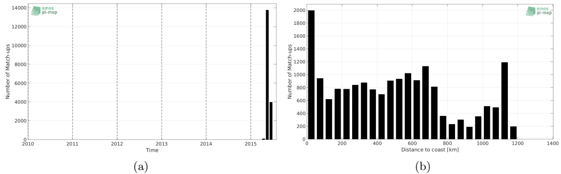
Figure 1: Number of match-ups between TSG-GOSUD-Sailing-ship and SMAP-L3-JPL-V4-MONTHLY-60KM SSS as a function of time (a) and as function of the distance to coast (b) over the Mid-Low Latitudes 45N-45S Pi-MEP region and for the full satellite product period.
