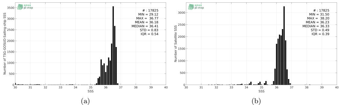
Figure 2: Histograms of SSS from TSG-GOSUD-Sailing-ship (a) and SMAP-L3-JPL-V4-MONTHLY-60KM (b) considering all match-up pairs per bins of 0.1 over the Mid-Low Latitudes 45N-45S Pi-MEP region and for the full satellite product period.
