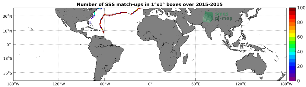
Figure 4: Number of SSS match-ups between TSG-GOSUD-Sailing-ship SSS and the SMAP-L3-JPL-V4-MONTHLY-60KM SSS product for the Mid-Low Latitudes 45N-45S Pi-MEP region over 1°x1° boxes and for the full satellite product period.
