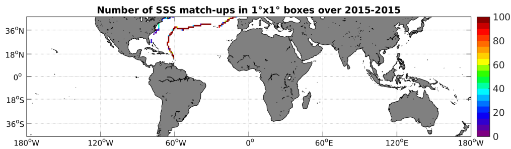
Figure 4: Number of SSS match-ups between TSG-GOSUD-Sailing-ship SSS and the SMAP-L3-JPL-V4-MONTHLY-60KM SSS product for the Mid-Low Latitudes 45N-45S Pi-MEP region over 1^{\circ} \times 1^{\circ} boxes and for the full satellite product period.
