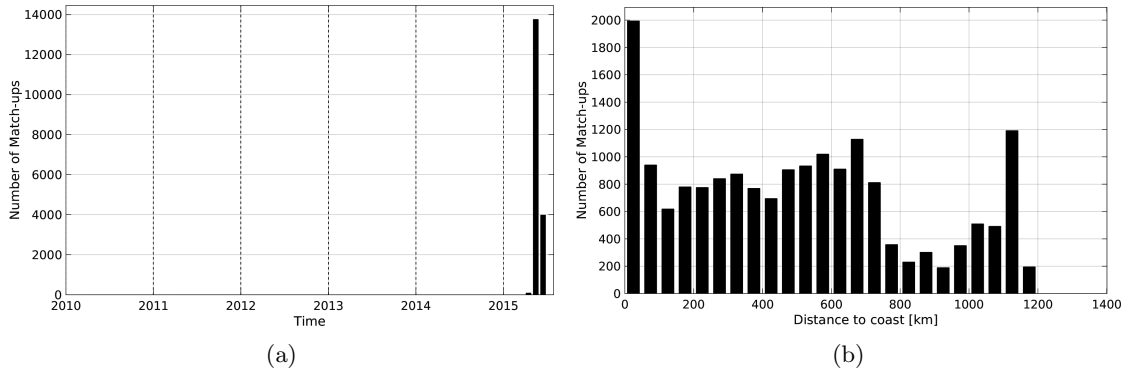
Figure 1: Number of match-ups between TSG-GOSUD-Sailing-ship and SMAP-L3-JPL-V4-MONTHLY-60KM SSS as a function of time (a) and as function of the distance to coast (b) over the Mid-Low Latitudes 45N-45S Pi-MEP region and for the full satellite product period.
