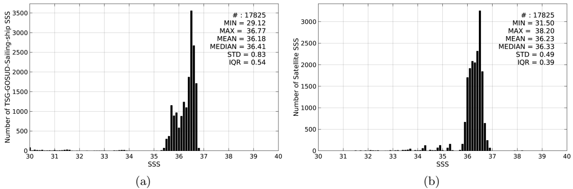
Figure 2: Histograms of SSS from TSG-GOSUD-Sailing-ship (a) and SMAP-L3-JPL-V4-MONTHLY-60KM (b) considering all match-up pairs per bins of 0.1 over the Mid-Low Latitudes 45N-45S Pi-MEP region and for the full satellite product period.
