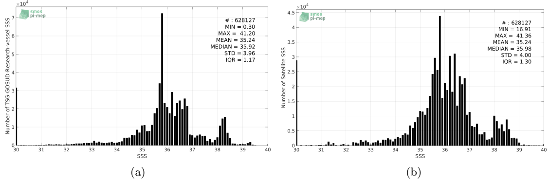
Figure 2: Histograms of SSS from TSG-GOSUD-Research-vessel (a) and SMAP-L3-JPL-V4-MONTHLY-60KM (b) considering all match-up pairs per bins of 0.1 over the Mid-Low Latitudes 45N-45S Pi-MEP region and for the full satellite product period.
