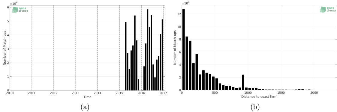
Figure 1: Number of match-ups between TSG-GOSUD-Research-vessel and SMAP-L3-JPL-V4-MONTHLY-60KM SSS as a function of time (a) and as function of the distance to coast (b) over the Mid-Low Latitudes 45N-45S Pi-MEP region and for the full satellite product period.
