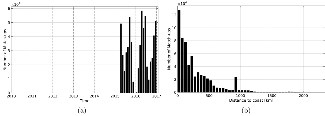
Figure 1: Number of match-ups between TSG-GOSUD-Research-vessel and SMAP-L3-JPL-V4-MONTHLY-60KM SSS as a function of time (a) and as function of the distance to coast (b) over the Mid-Low Latitudes 45N-45S Pi-MEP region and for the full satellite product period.
