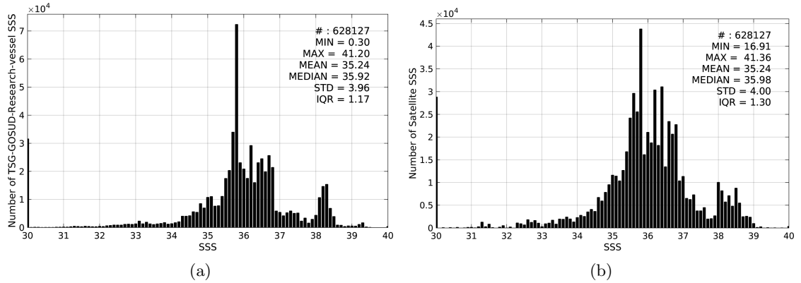
Figure 2: Histograms of SSS from TSG-GOSUD-Research-vessel (a) and SMAP-L3-JPL-V4-MONTHLY-60KM (b) considering all match-up pairs per bins of 0.1 over the Mid-Low Latitudes 45N-45S Pi-MEP region and for the full satellite product period.
