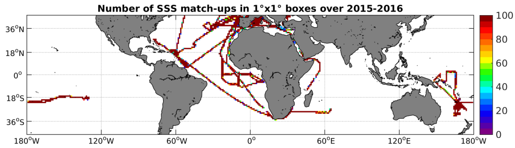
Figure 4: Number of SSS match-ups between TSG-GOSUD-Research-vessel SSS and the SMAP-L3-JPL-V4-MONTHLY-60KM SSS product for the Mid-Low Latitudes 45N-45S Pi-MEP region over 1^\circ \times 1^\circ boxes and for the full satellite product period.
