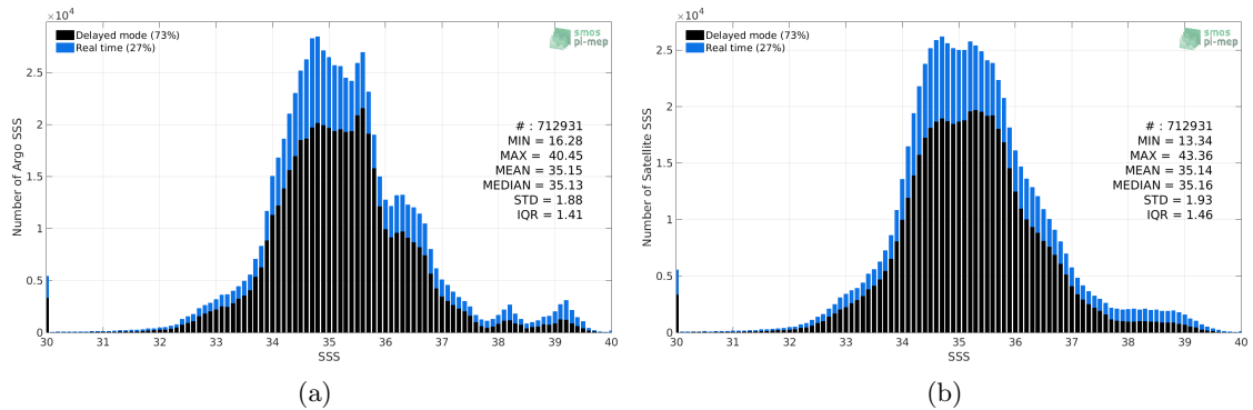
Figure 2: Histograms of SSS from Argo (a) and SMAP SSS L2-AVERAGED v5 (RSS) (b) considering all match-up pairs per bins of 0.1 over the Mid-Low Latitudes 45N-45S Pi-MEP region and for the full satellite product period.
