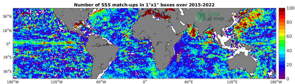
Figure 4: Number of SSS match-ups between Argo SSS and the SMAP SSS L2-AVERAGED v5 (RSS) SSS product for the Mid-Low Latitudes 45N-45S Pi-MEP region over 1^\circ \times 1^\circ boxes and for the full satellite product period.
