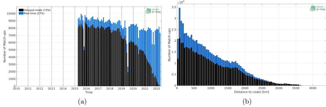
Figure 1: Number of match-ups between Argo and SMAP SSS L2-AVERAGED v5 (RSS) SSS as a function of time (a) and as function of the distance to coast (b) over the Mid-Low Latitudes 45N-45S Pi-MEP region and for the full satellite product period.
