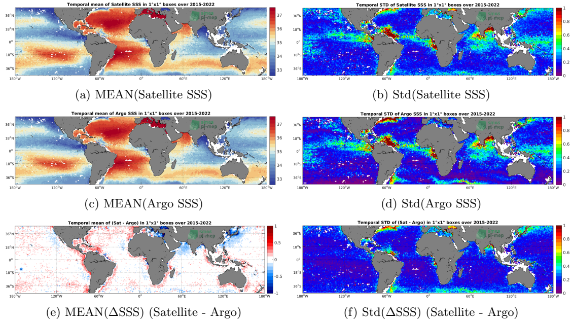
Figure 6: Temporal mean (left) and Std (right) of SSS from SMAP SSS L2-AVERAGED v5 (RSS) (top), Argo (middle), and of \Delta SSS (Satellite - Argo). Only match-up pairs are used to generate these maps.
