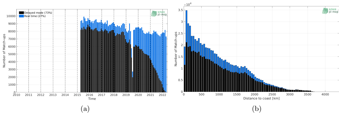
Figure 1: Number of match-ups between Argo and SMAP SSS L2-AVERAGED v5.0 (JPL) SSS as a function of time (a) and as function of the distance to coast (b) over the Mid-Low Latitudes 45N-45S Pi-MEP region and for the full satellite product period.
