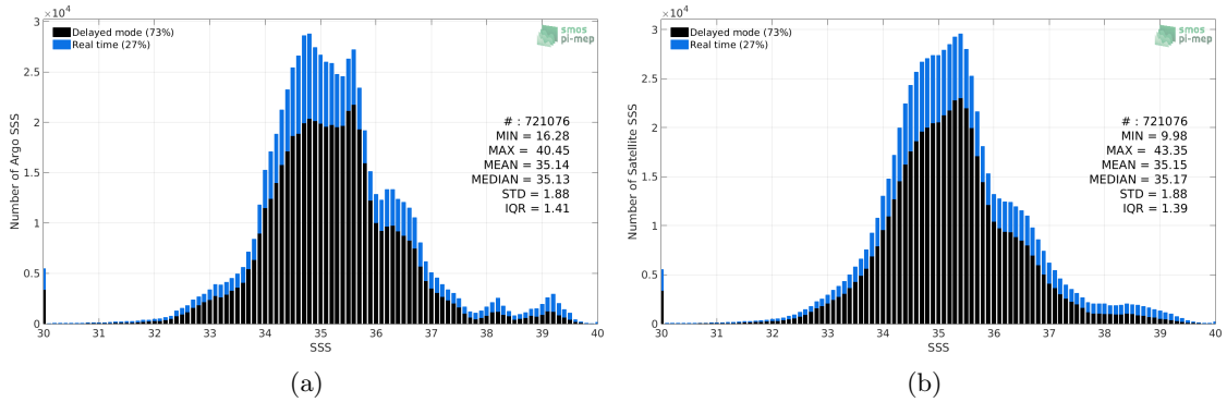
Figure 2: Histograms of SSS from Argo (a) and SMAP SSS L2-AVERAGED v5.0 (JPL) (b) considering all match-up pairs per bins of 0.1 over the Mid-Low Latitudes 45N-45S Pi-MEP region and for the full satellite product period.
