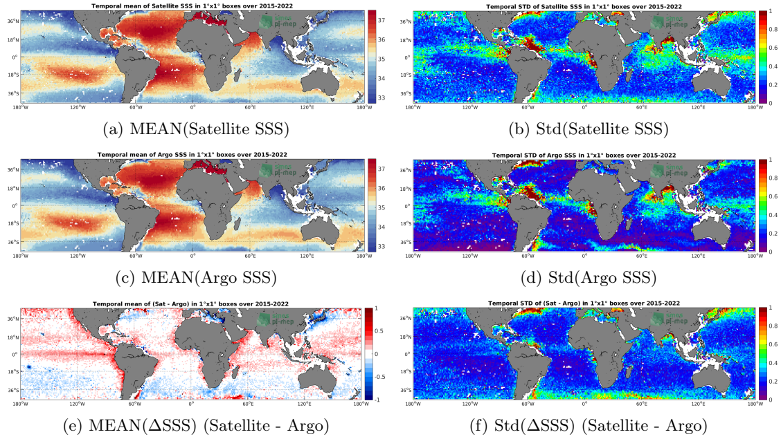
Figure 6: Temporal mean (left) and Std (right) of SSS from SMAP SSS L2-AVERAGED v5.0 (JPL) (top), Argo (middle), and of \Delta SSS (Satellite - Argo). Only match-up pairs are used to generate these maps.
