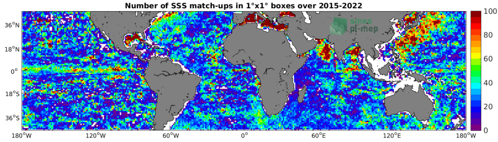
Figure 4: Number of SSS match-ups between Argo SSS and the SMAP SSS L2-AVERAGED v5.0 (JPL) SSS product for the Mid-Low Latitudes 45N-45S Pi-MEP region over 1^\circ \times 1^\circ boxes and for the full satellite product period.
