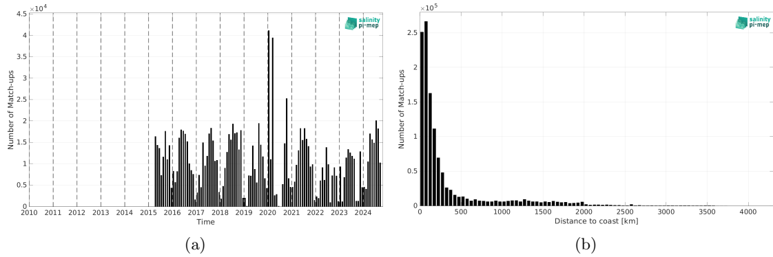
Figure 2: Number of match-ups between TSG (SAMOS) and SMAP SSS L2 v6 (RSS) SSS as a function of time (a) and as function of the distance to coast (b) over the Mid-Low Latitudes 45N-45S Pi-MEP region and for the full satellite product period.
