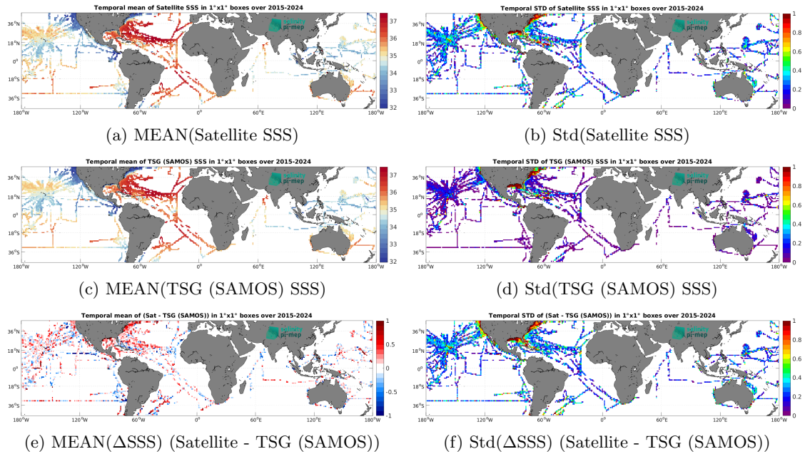
Figure 7: Temporal mean (left) and Std (right) of SSS from SMAP SSS L2 v6 (RSS) (top), TSG (SAMOS) (middle), and of \Delta SSS (Satellite - TSG (SAMOS)). Only match-up pairs are used to generate these maps.
