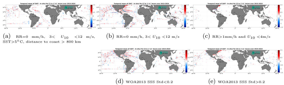
Figure 14: Temporal mean gridded over spatial boxes of size 1^\circ \times 1^\circ of \Delta SSS (SMAP SSS L2 v6 (RSS) - TSG (SAMOS)) for 5 different subdatasets corresponding to: RR=0 mm/h, 3 < U_{10} < 12 m/s, SST > 5°C, distance to coast > 800 km (a), RR=0 mm/h, 3 < U_{10} < 12 m/s (b), RR > 1mm/h and U_{10} < 4 m/s (c), WOA2013 SSS Std < 0.2 (d), WOA2013 SSS Std > 0.2 (e).
