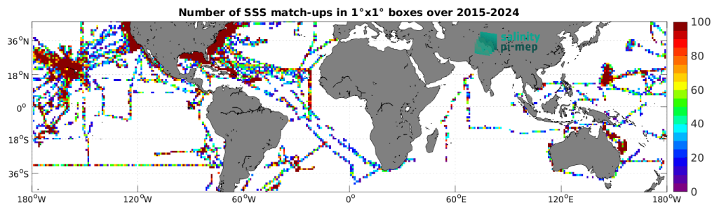
Figure 5: Number of SSS match-ups between TSG (SAMOS) SSS and the SMAP SSS L2 v6 (RSS) SSS product for the Mid-Low Latitudes 45N-45S Pi-MEP region over 1^\circ \times 1^\circ boxes and for the full satellite product period.
