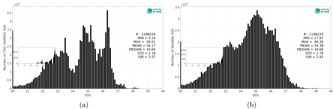
Figure 3: Histograms of SSS from TSG (SAMOS) (a) and SMAP SSS L2 v6 (RSS) (b) considering all match-up pairs per bins of 0.1 over the Mid-Low Latitudes 45N-45S Pi-MEP region and for the full satellite product period.
