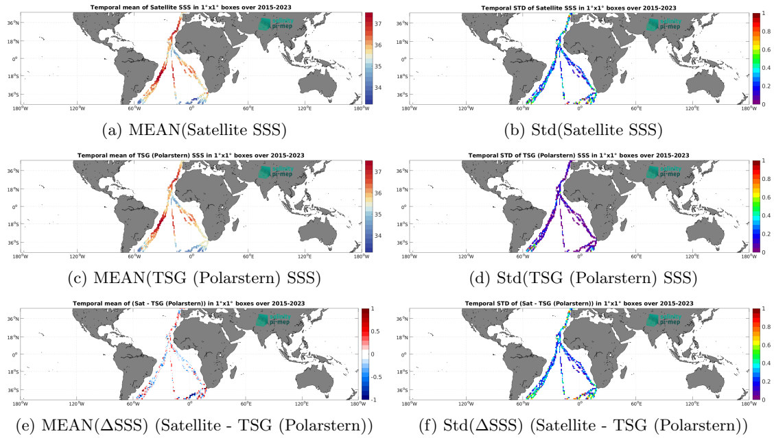
Figure 7: Temporal mean (left) and Std (right) of SSS from SMAP SSS L2 v6 (RSS) (top), TSG (Polarstern) (middle), and of \Delta SSS (Satellite - TSG (Polarstern)). Only match-up pairs are used to generate these maps.
