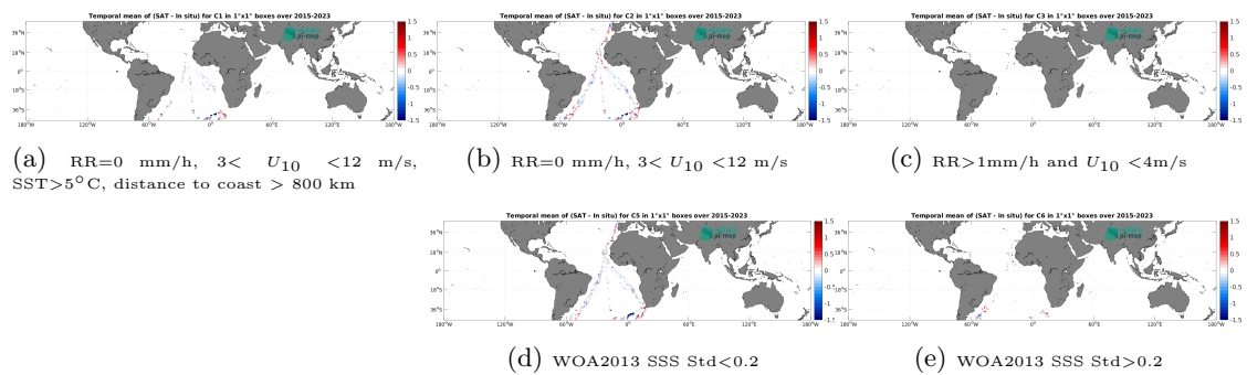
Figure 14: Temporal mean gridded over spatial boxes of size 1^\circ \times 1^\circ of \Delta SSS (SMAP SSS L2 v6 (RSS) - TSG (Polarstern)) for 5 different subdatasets corresponding to: RR=0 mm/h, 3 < U_{10} < 12 m/s, SST > 5°C, distance to coast > 800 km (a), RR=0 mm/h, 3 < U_{10} < 12 m/s (b), RR > 1mm/h and U_{10} < 4 m/s (c), WOA2013 SSS Std < 0.2 (d), WOA2013 SSS Std > 0.2 (e).
