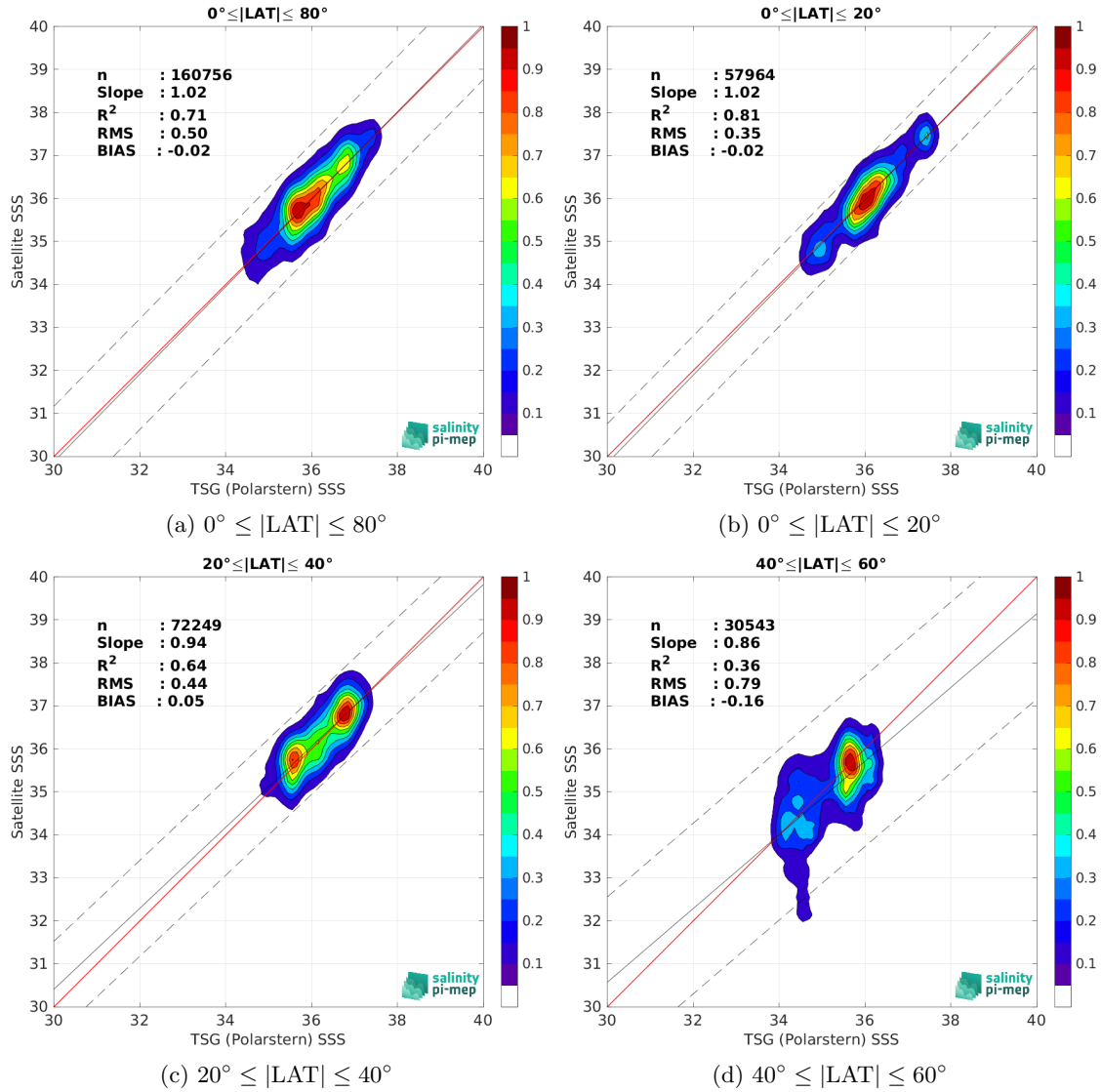
Figure 10: Contour maps of the concentration of SMAP SSS L2 v6 (RSS) SSS (y-axis) versus TSG (Polarstern) SSS (x-axis) at match-up pairs for different latitude bands. For each plot, the red line shows x=y . The black thin and dashed lines indicate a linear fit through the data cloud and the \pm 95\% confidence levels, respectively. The number match-up pairs n , the slope and R^2 coefficient of the linear fit, the root mean square (RMS) and the mean bias between satellite and in situ data are indicated for each latitude band in each plots.
