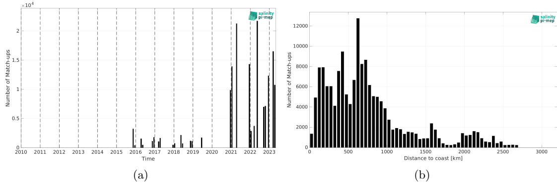
Figure 2: Number of match-ups between TSG (Polarstern) and SMAP SSS L2 v6 (RSS) SSS as a function of time (a) and as function of the distance to coast (b) over the Mid-Low Latitudes 45N-45S Pi-MEP region and for the full satellite product period.
