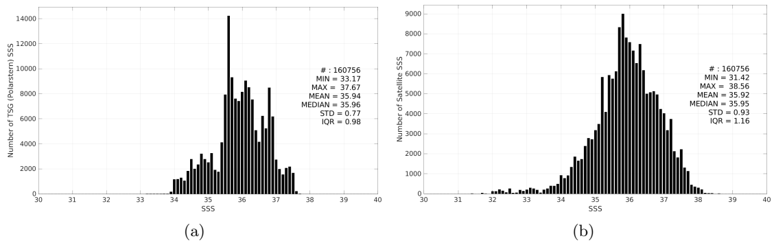
Figure 3: Histograms of SSS from TSG (Polarstern) (a) and SMAP SSS L2 v6 (RSS) (b) considering all match-up pairs per bins of 0.1 over the Mid-Low Latitudes 45N-45S Pi-MEP region and for the full satellite product period.
