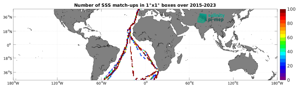
Figure 5: Number of SSS match-ups between TSG (Polarstern) SSS and the SMAP SSS L2 v6 (RSS) SSS product for the Mid-Low Latitudes 45N-45S Pi-MEP region over 1^\circ \times 1^\circ boxes and for the full satellite product period.
