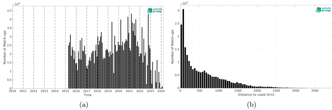
Figure 2: Number of match-ups between TSG (LEGOS-DM) and SMAP SSS L2 v6 (RSS) SSS as a function of time (a) and as function of the distance to coast (b) over the Mid-Low Latitudes 45N-45S Pi-MEP region and for the full satellite product period.
