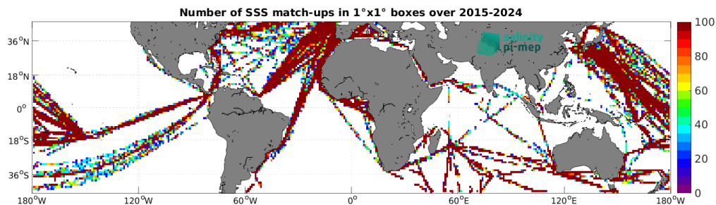
Figure 5: Number of SSS match-ups between TSG (LEGOS-DM) SSS and the SMAP SSS L2 v6 (RSS) SSS product for the Mid-Low Latitudes 45N-45S Pi-MEP region over 1^\circ \times 1^\circ boxes and for the full satellite product period.
