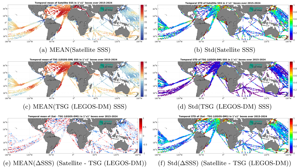
Figure 7: Temporal mean (left) and Std (right) of SSS from SMAP SSS L2 v6 (RSS) (top), TSG (LEGOS-DM) (middle), and of \Delta SSS (Satellite - TSG (LEGOS-DM)). Only match-up pairs are used to generate these maps.
