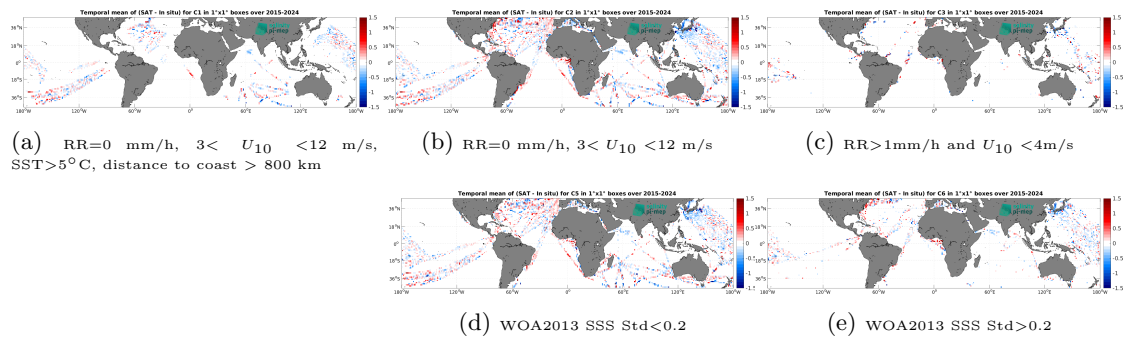
Figure 14: Temporal mean gridded over spatial boxes of size 1^\circ \times 1^\circ of \Delta\text{SSS} (SMAP SSS L2 v6 (RSS) - TSG (LEGOS-DM)) for 5 different subdatasets corresponding to:RR=0 mm/h, 3 < U_{10} < 12 m/s, SST>5°C, distance to coast > 800 km (a), RR=0 mm/h, 3 < U_{10} < 12 m/s (b), RR>1mm/h and U_{10} < 4 m/s (c), WOA2013 SSS Std<0.2 (d), WOA2013 SSS Std>0.2 (e).
