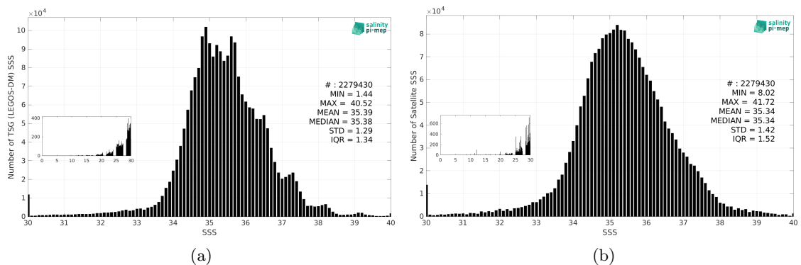
Figure 3: Histograms of SSS from TSG (LEGOS-DM) (a) and SMAP SSS L2 v6 (RSS) (b) considering all match-up pairs per bins of 0.1 over the Mid-Low Latitudes 45N-45S Pi-MEP region and for the full satellite product period.
