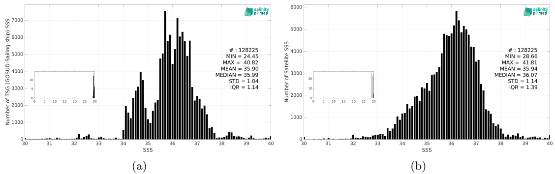
Figure 3: Histograms of SSS from TSG (GOSUD-Sailing-ship) (a) and SMAP SSS L2 v6 (RSS) (b) considering all match-up pairs per bins of 0.1 over the Mid-Low Latitudes 45N-45S Pi-MEP region and for the full satellite product period.
