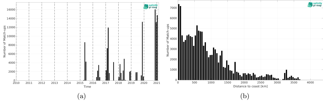
Figure 2: Number of match-ups between TSG (GOSUD-Sailing-ship) and SMAP SSS L2 v6 (RSS) SSS as a function of time (a) and as function of the distance to coast (b) over the Mid-Low Latitudes 45N-45S Pi-MEP region and for the full satellite product period.
