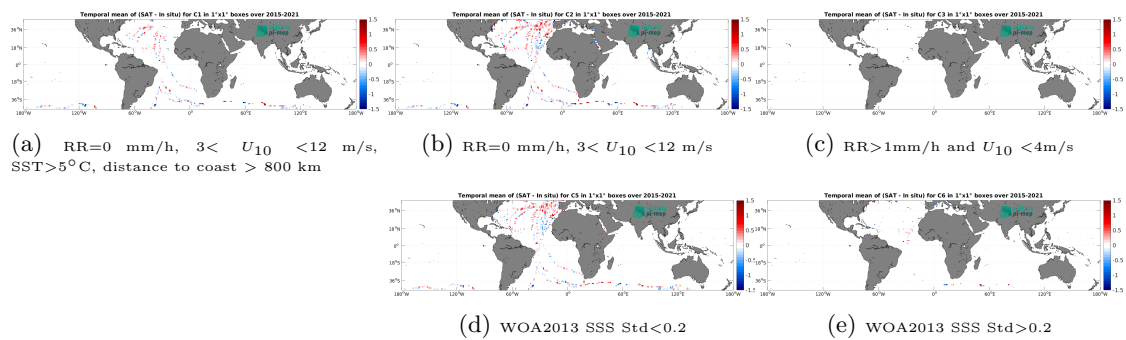
Figure 14: Temporal mean gridded over spatial boxes of size 1^\circ \times 1^\circ of \Delta SSS (SMAP SSS L2 v6 (RSS) - TSG (GOSUD-Sailing-ship)) for 5 different subdatasets corresponding to:RR=0 mm/h, 3 < U_{10} < 12 m/s, SST>5°C, distance to coast > 800 km (a), RR=0 mm/h, 3 < U_{10} < 12 m/s (b), RR>1mm/h and U_{10} < 4 m/s (c), WOA2013 SSS Std<0.2 (d), WOA2013 SSS Std>0.2 (e).
