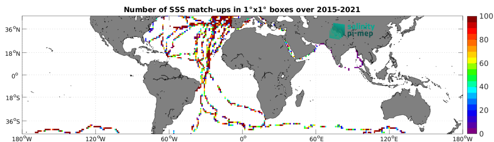
Figure 5: Number of SSS match-ups between TSG (GOSUD-Sailing-ship) SSS and the SMAP SSS L2 v6 (RSS) SSS product for the Mid-Low Latitudes 45N-45S Pi-MEP region over 1^\circ \times 1^\circ boxes and for the full satellite product period.
