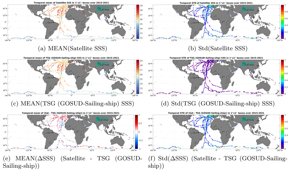
Figure 7: Temporal mean (left) and Std (right) of SSS from SMAP SSS L2 v6 (RSS) (top), TSG (GOSUD-Sailing-ship) (middle), and of \Delta SSS (Satellite - TSG (GOSUD-Sailing-ship)). Only match-up pairs are used to generate these maps.
