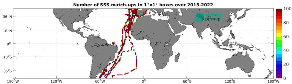
Figure 5: Number of SSS match-ups between TSG (CSIC-UTM) SSS and the SMAP SSS L2 v6 (RSS) SSS product for the Mid-Low Latitudes 45N-45S Pi-MEP region over 1^\circ \times 1^\circ boxes and for the full satellite product period.
