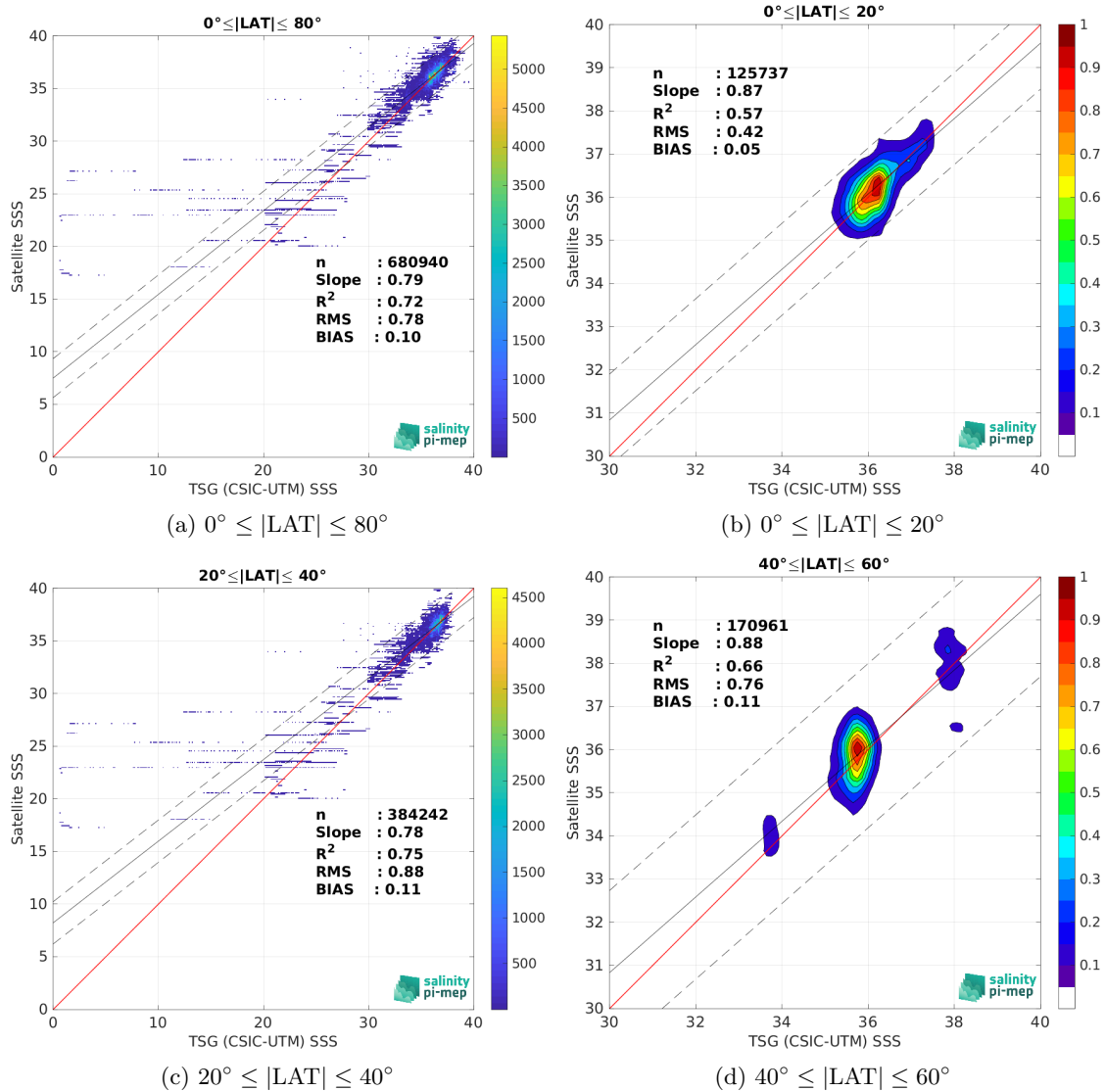
Figure 10: Contour maps of the concentration of SMAP SSS L2 v6 (RSS) SSS (y-axis) versus TSG (CSIC-UTM) SSS (x-axis) at match-up pairs for different latitude bands. For each plot, the red line shows x=y . The black thin and dashed lines indicate a linear fit through the data cloud and the \pm 95\% confidence levels, respectively. The number match-up pairs n , the slope and R^2 coefficient of the linear fit, the root mean square (RMS) and the mean bias between satellite and in situ data are indicated for each latitude band in each plots.
