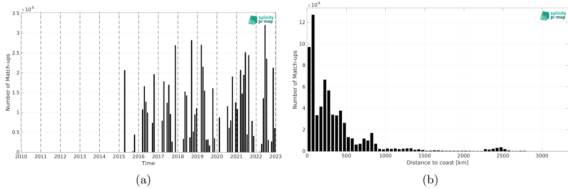
Figure 2: Number of match-ups between TSG (CSIC-UTM) and SMAP SSS L2 v6 (RSS) SSS as a function of time (a) and as function of the distance to coast (b) over the Mid-Low Latitudes 45N-45S Pi-MEP region and for the full satellite product period.
