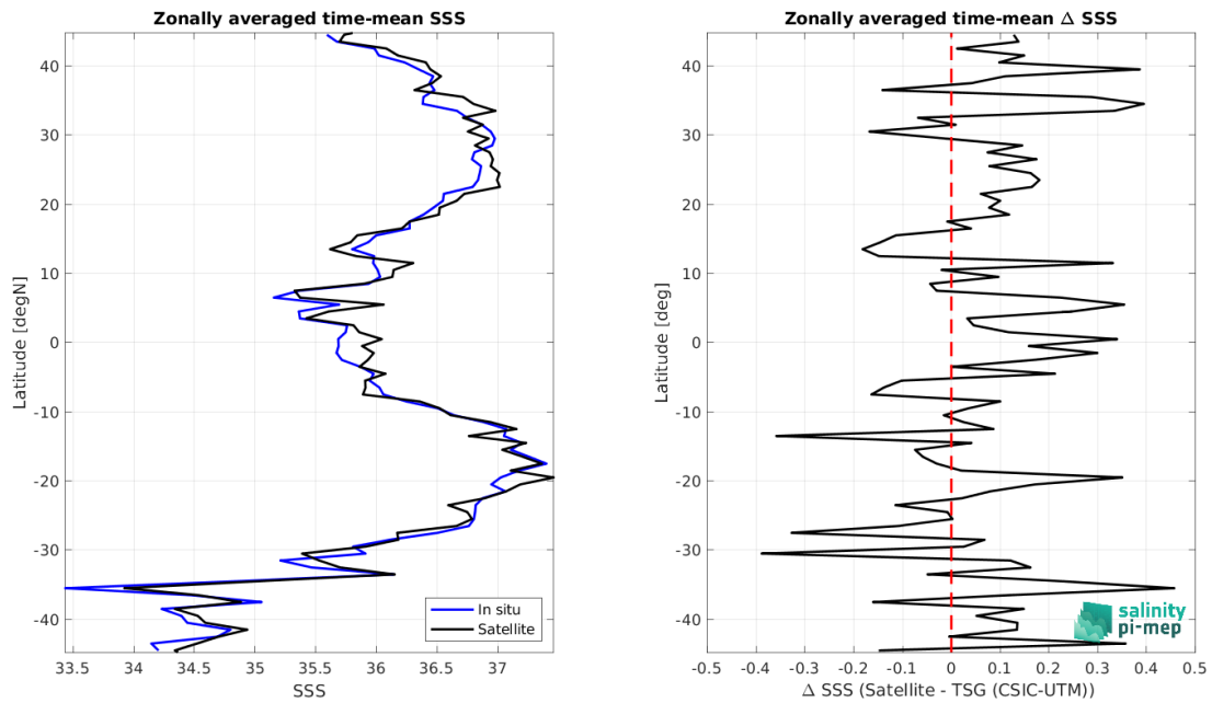
Figure 9: Left panel: Zonal mean SSS from SMAP SSS L2 v6 (RSS) satellite product (black) and from TSG (CSIC-UTM) (blue). Right panel: Zonal mean of \Delta SSS (Satellite - TSG (CSIC-UTM)) for all the collected Pi-MEP match-up pairs estimated over the full satellite product period.
