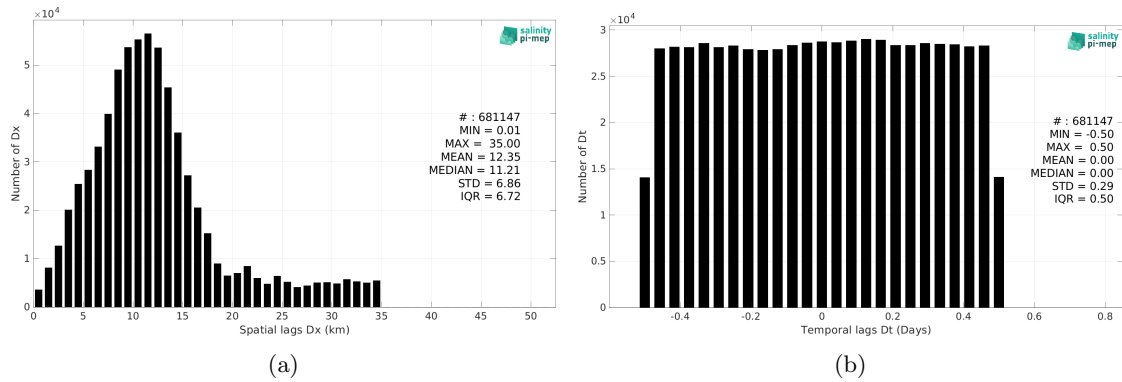
Figure 6: Histograms of the spatial (a) and temporal (b) lags between the location/time of the TSG (CSIC-UTM) measurement and the date of the corresponding SMAP SSS L2 v6 (RSS) SSS pixel.
