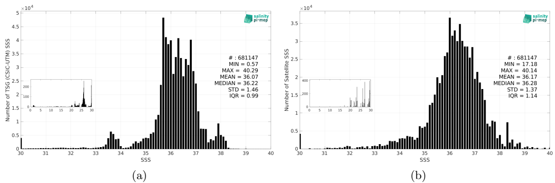
Figure 3: Histograms of SSS from TSG (CSIC-UTM) (a) and SMAP SSS L2 v6 (RSS) (b) considering all match-up pairs per bins of 0.1 over the Mid-Low Latitudes 45N-45S Pi-MEP region and for the full satellite product period.
