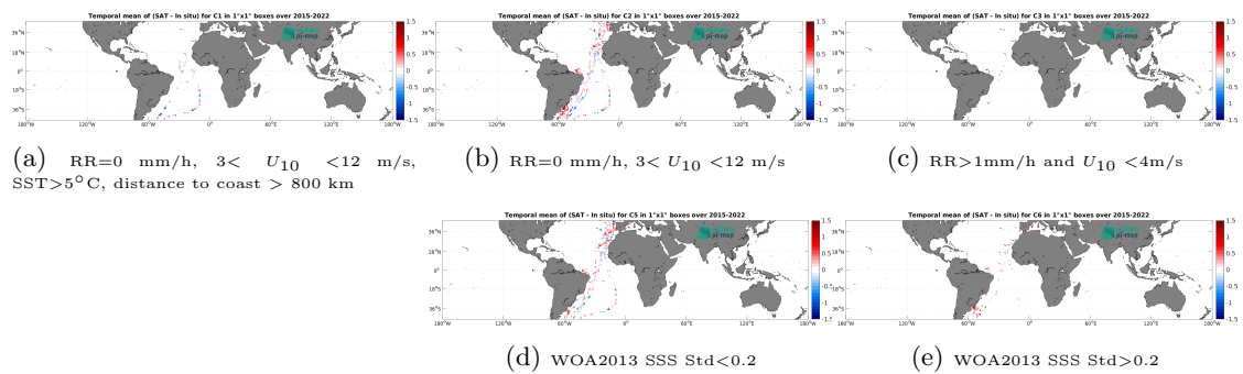
Figure 14: Temporal mean gridded over spatial boxes of size 1^\circ \times 1^\circ of \Delta SSS (SMAP SSS L2 v6 (RSS) - TSG (CSIC-UTM)) for 5 different subdatasets corresponding to:RR=0 mm/h, 3 < U_{10} < 12 m/s, SST >5^\circ C, distance to coast > 800 km (a), RR=0 mm/h, 3 < U_{10} < 12 m/s (b), RR >1 mm/h and U_{10} < 4 m/s (c), WOA2013 SSS Std <0.2 (d), WOA2013 SSS Std >0.2 (e).
