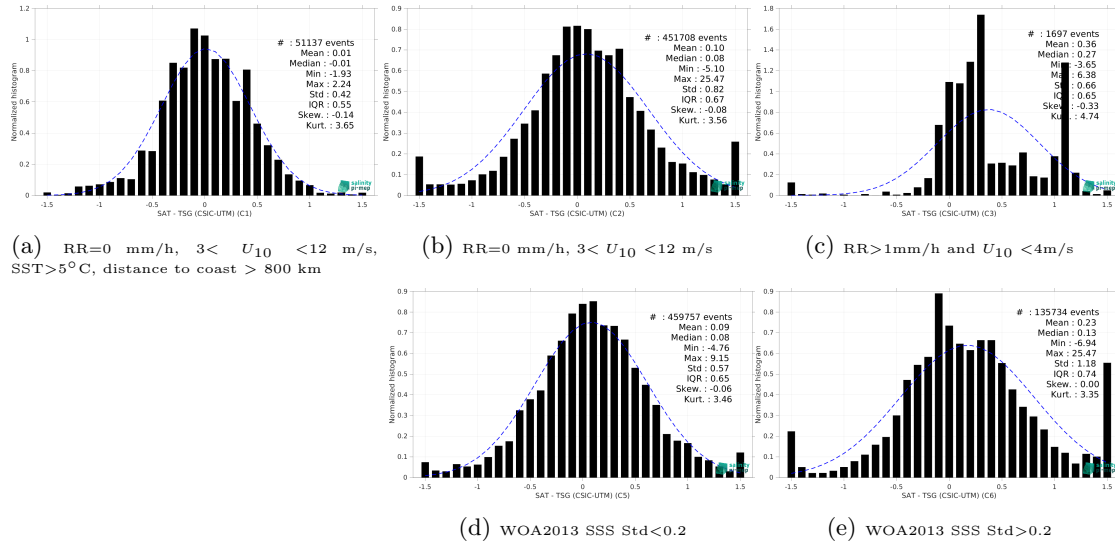
Figure 15: Normalized histogram of \Delta SSS (SMAP SSS L2 v6 (RSS) - TSG (CSIC-UTM)) for 5 different subdatasets corresponding to: RR=0 mm/h, 3 < U_{10} < 12 m/s, SST>5°C, distance to coast > 800 km (a), RR=0 mm/h, 3 < U_{10} < 12 m/s (b), RR>1mm/h and U_{10} < 4 m/s (c), WOA2013 SSS Std<0.2 (d), WOA2013 SSS Std>0.2 (e).
