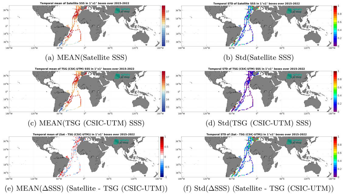
Figure 7: Temporal mean (left) and Std (right) of SSS from SMAP SSS L2 v6 (RSS) (top), TSG (CSIC-UTM) (middle), and of \Delta SSS (Satellite - TSG (CSIC-UTM)). Only match-up pairs are used to generate these maps.
