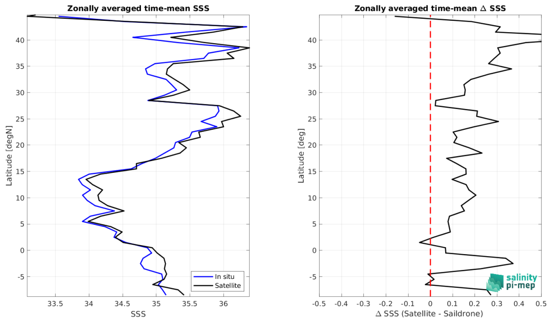
Figure 9: Left panel: Zonal mean SSS from SMAP SSS L2 v6 (RSS) satellite product (black) and from Saildrone (blue). Right panel: Zonal mean of \Delta SSS (Satellite - Saildrone) for all the collected Pi-MEP match-up pairs estimated over the full satellite product period.
