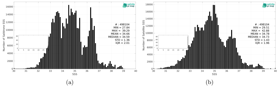
Figure 3: Histograms of SSS from Sairdrone (a) and SMAP SSS L2 v6 (RSS) (b) considering all match-up pairs per bins of 0.1 over the Mid-Low Latitudes 45N-45S Pi-MEP region and for the full satellite product period.
