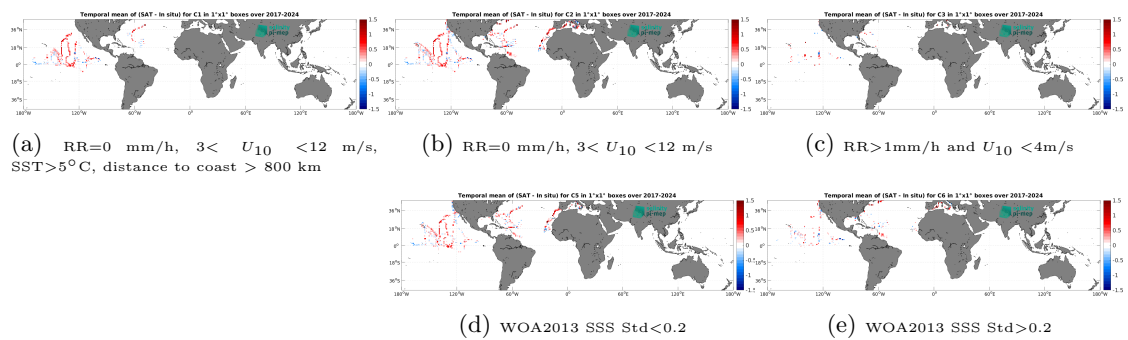
Figure 14: Temporal mean gridded over spatial boxes of size 1^\circ \times 1^\circ of \Delta SSS (SMAP SSS L2 v6 (RSS) - Saldrone) for 5 different subdatasets corresponding to: RR=0 mm/h, 3 < U_{10} < 12 m/s, SST>5°C, distance to coast > 800 km (a), RR=0 mm/h, 3 < U_{10} < 12 m/s (b), RR>1mm/h and U_{10} < 4 m/s (c), WOA2013 SSS Std<0.2 (d), WOA2013 SSS Std>0.2 (e).
