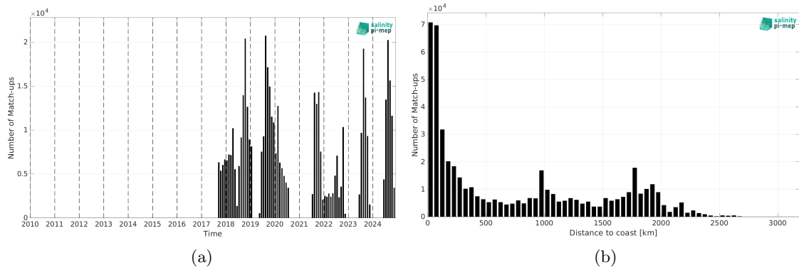
Figure 2: Number of match-ups between Sairdrone and SMAP SSS L2 v6 (RSS) SSS as a function of time (a) and as function of the distance to coast (b) over the Mid-Low Latitudes 45N-45S Pi-MEP region and for the full satellite product period.
