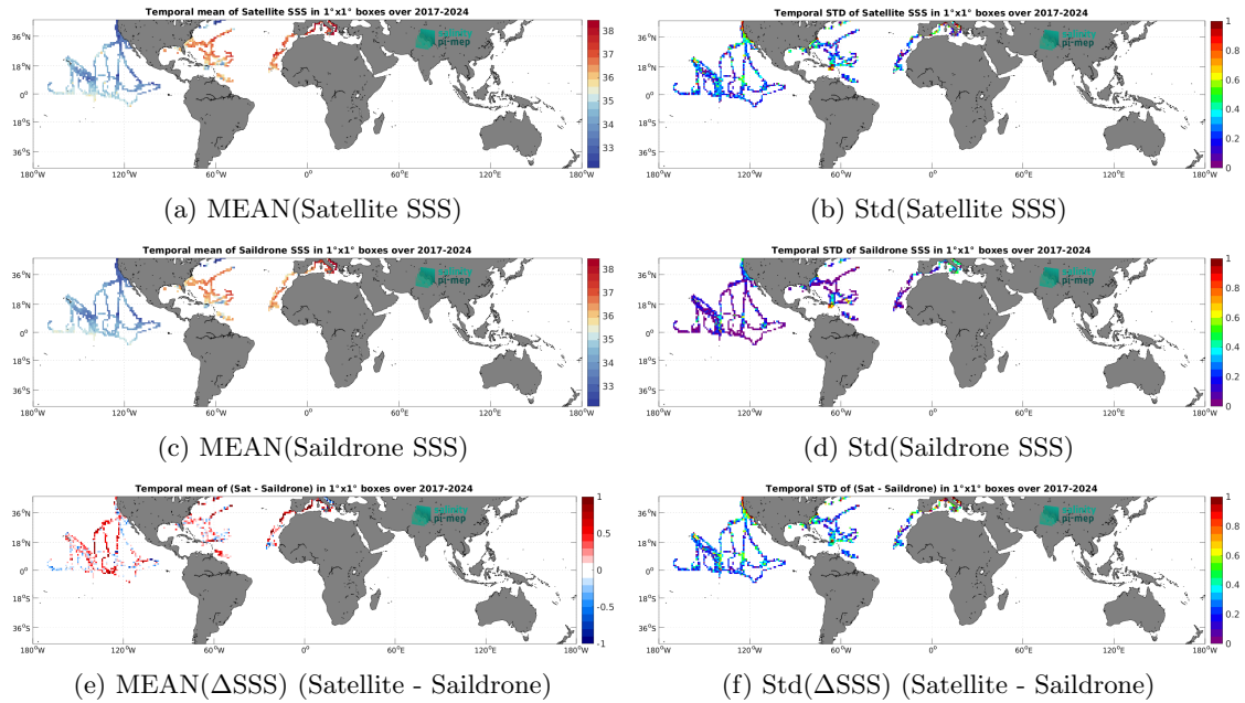
Figure 7: Temporal mean (left) and Std (right) of SSS from SMAP SSS L2 v6 (RSS) (top), Saildrone (middle), and of \Delta SSS (Satellite - Saildrone). Only match-up pairs are used to generate these maps.
