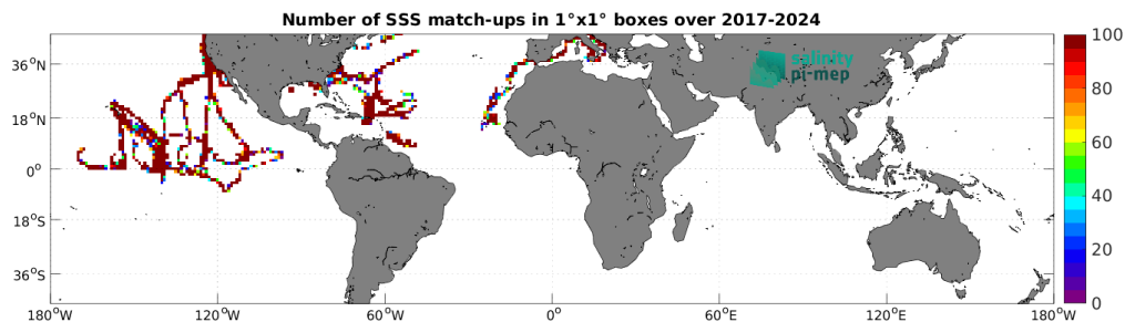
Figure 5: Number of SSS match-ups between Saildrone SSS and the SMAP SSS L2 v6 (RSS) SSS product for the Mid-Low Latitudes 45N-45S Pi-MEP region over 1^\circ \times 1^\circ boxes and for the full satellite product period.
