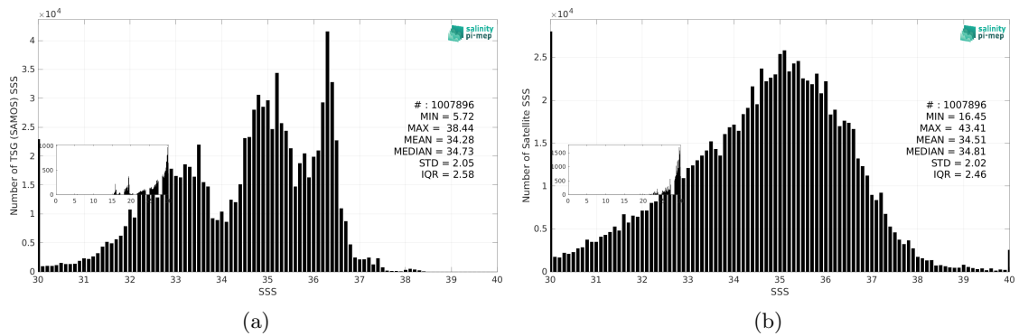
Figure 3: Histograms of SSS from TSG (SAMOS) (a) and SMAP SSS L2 v6 - 40 km (RSS) (b) considering all match-up pairs per bins of 0.1 over the Mid-Low Latitudes 45N-45S Pi-MEP region and for the full satellite product period.
