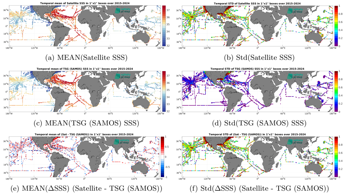
Figure 7: Temporal mean (left) and Std (right) of SSS from SMAP SSS L2 v6 - 40 km (RSS) (top), TSG (SAMOS) (middle), and of \Delta SSS (Satellite - TSG (SAMOS)). Only match-up pairs are used to generate these maps.
