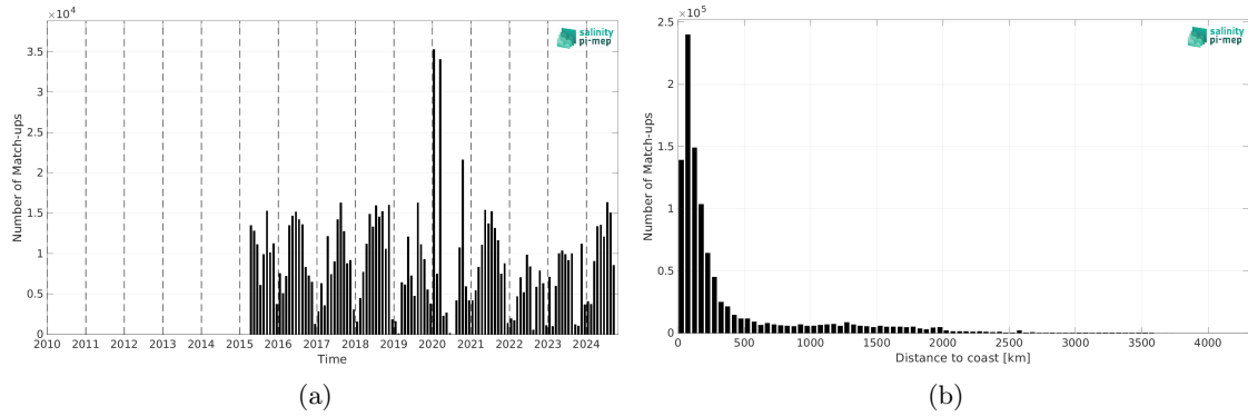
Figure 2: Number of match-ups between TSG (SAMOS) and SMAP SSS L2 v6 - 40 km (RSS) SSS as a function of time (a) and as function of the distance to coast (b) over the Mid-Low Latitudes 45N-45S Pi-MEP region and for the full satellite product period.
