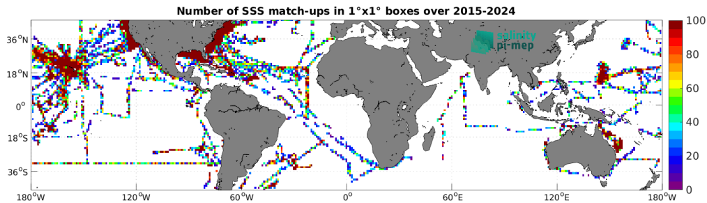
Figure 5: Number of SSS match-ups between TSG (SAMOS) SSS and the SMAP SSS L2 v6 - 40 km (RSS) SSS product for the Mid-Low Latitudes 45N-45S Pi-MEP region over 1^\circ \times 1^\circ boxes and for the full satellite product period.
