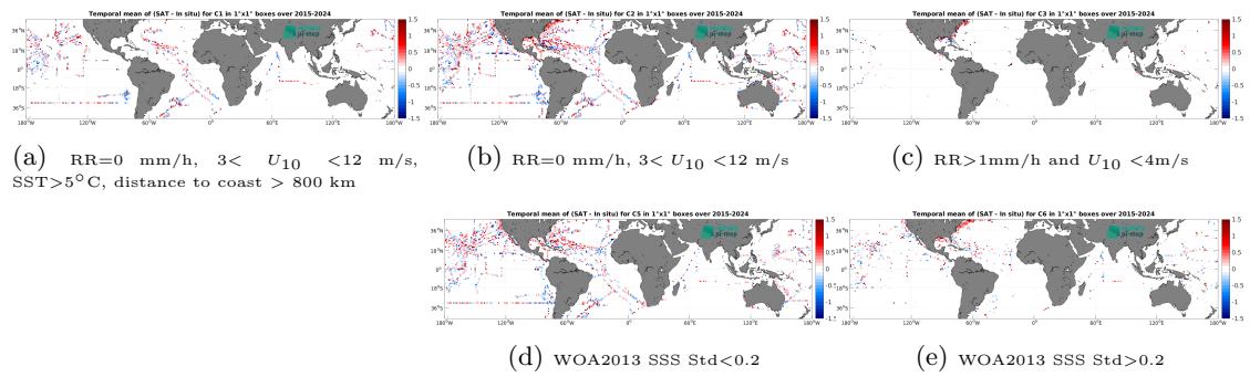
Figure 14: Temporal mean gridded over spatial boxes of size 1^\circ \times 1^\circ of \Delta SSS (SMAP SSS L2 v6 - 40 km (RSS) - TSG (SAMOS)) for 5 different subdatasets corresponding to: RR=0 mm/h, 3 < U_{10} < 12 m/s, SST > 5°C, distance to coast > 800 km (a), RR=0 mm/h, 3 < U_{10} < 12 m/s (b), RR > 1mm/h and U_{10} < 4 m/s (c), WOA2013 SSS Std < 0.2 (d), WOA2013 SSS Std > 0.2 (e).
