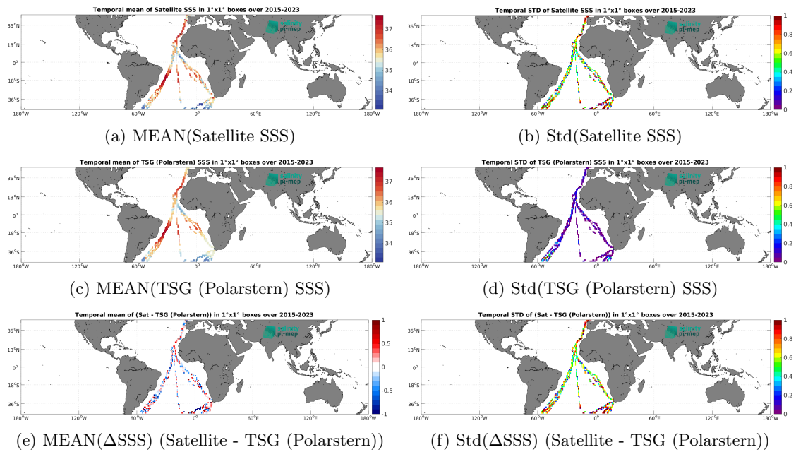
Figure 7: Temporal mean (left) and Std (right) of SSS from SMAP SSS L2 v6 - 40 km (RSS) (top), TSG (Polarstern) (middle), and of \Delta SSS (Satellite - TSG (Polarstern)). Only match-up pairs are used to generate these maps.
