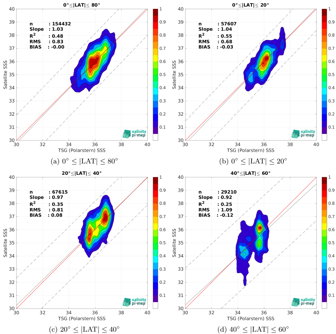
Figure 10: Contour maps of the concentration of SMAP SSS L2 v6 - 40 km (RSS) SSS (y-axis) versus TSG (Polarstern) SSS (x-axis) at match-up pairs for different latitude bands. For each plot, the red line shows x=y . The black thin and dashed lines indicate a linear fit through the data cloud and the \pm 95\% confidence levels, respectively. The number match-up pairs n , the slope and R^2 coefficient of the linear fit, the root mean square (RMS) and the mean bias between satellite and in situ data are indicated for each latitude band in each plots.
