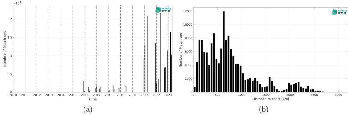
Figure 2: Number of match-ups between TSG (Polarstern) and SMAP SSS L2 v6 - 40 km (RSS) SSS as a function of time (a) and as function of the distance to coast (b) over the Mid-Low Latitudes 45N-45S Pi-MEP region and for the full satellite product period.
