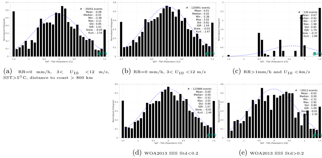
Figure 15: Normalized histogram of \Delta SSS (SMAP SSS L2 v6 - 40 km (RSS) - TSG (Polarstern)) for 5 different subdatasets corresponding to: RR=0 mm/h, 3 < U_{10} < 12 m/s, SST > 5°C, distance to coast > 800 km (a), RR=0 mm/h, 3 < U_{10} < 12 m/s (b), RR > 1mm/h and U_{10} < 4 m/s (c), WOA2013 SSS Std < 0.2 (d), WOA2013 SSS Std > 0.2 (e).
