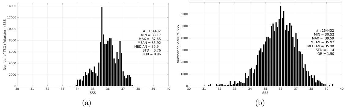
Figure 3: Histograms of SSS from TSG (Polarstern) (a) and SMAP SSS L2 v6 - 40 km (RSS) (b) considering all match-up pairs per bins of 0.1 over the Mid-Low Latitudes 45N-45S Pi-MEP region and for the full satellite product period.
