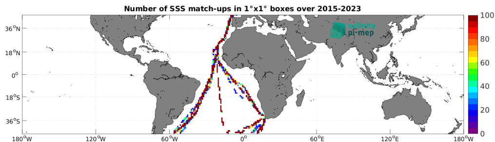
Figure 5: Number of SSS match-ups between TSG (Polarstern) SSS and the SMAP SSS L2 v6 - 40 km (RSS) SSS product for the Mid-Low Latitudes 45N-45S Pi-MEP region over 1^\circ \times 1^\circ boxes and for the full satellite product period.
