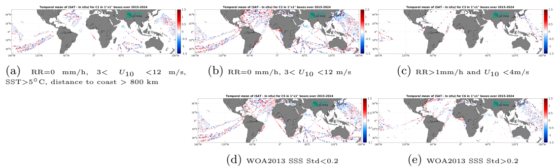
Figure 14: Temporal mean gridded over spatial boxes of size 1^\circ \times 1^\circ of \Delta SSS (SMAP SSS L2 v6 - 40 km (RSS) - TSG (LEGOS-DM)) for 5 different subdatasets corresponding to:RR=0 mm/h, 3 < U_{10} < 12 m/s, SST >5^\circ C, distance to coast > 800 km (a), RR=0 mm/h, 3 < U_{10} < 12 m/s (b), RR >1 mm/h and U_{10} < 4 m/s (c), WOA2013 SSS Std <0.2 (d), WOA2013 SSS Std >0.2 (e).
