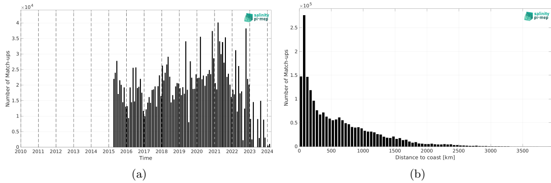
Figure 2: Number of match-ups between TSG (LEGOS-DM) and SMAP SSS L2 v6 - 40 km (RSS) SSS as a function of time (a) and as function of the distance to coast (b) over the Mid-Low Latitudes 45N-45S Pi-MEP region and for the full satellite product period.
