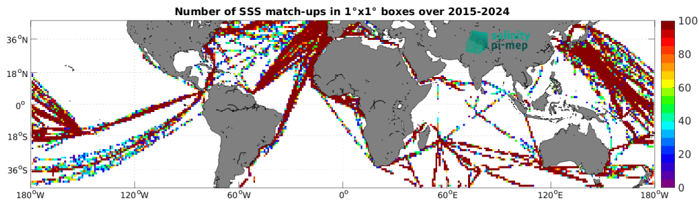
Figure 5: Number of SSS match-ups between TSG (LEGOS-DM) SSS and the SMAP SSS L2 v6 - 40 km (RSS) SSS product for the Mid-Low Latitudes 45N-45S Pi-MEP region over 1^\circ \times 1^\circ boxes and for the full satellite product period.
