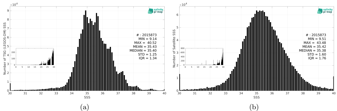
Figure 3: Histograms of SSS from TSG (LEGOS-DM) (a) and SMAP SSS L2 v6 - 40 km (RSS) (b) considering all match-up pairs per bins of 0.1 over the Mid-Low Latitudes 45N-45S Pi-MEP region and for the full satellite product period.
