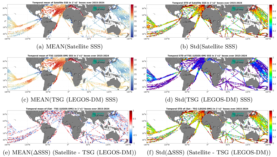
Figure 7: Temporal mean (left) and Std (right) of SSS from SMAP SSS L2 v6 - 40 km (RSS) (top), TSG (LEGOS-DM) (middle), and of \Delta SSS (Satellite - TSG (LEGOS-DM)). Only match-up pairs are used to generate these maps.
