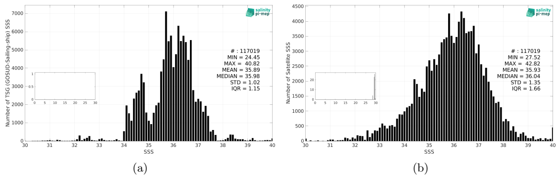
Figure 3: Histograms of SSS from TSG (GOSUD-Sailing-ship) (a) and SMAP SSS L2 v6 - 40 km (RSS) (b) considering all match-up pairs per bins of 0.1 over the Mid-Low Latitudes 45N-45S Pi-MEP region and for the full satellite product period.
