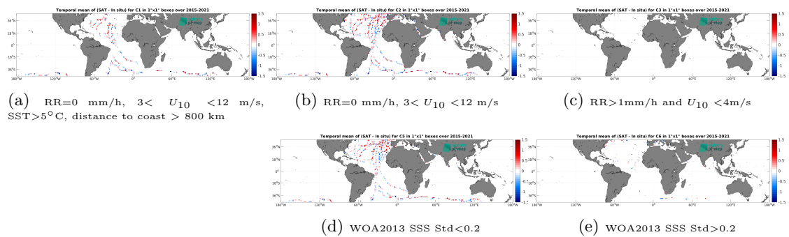
Figure 14: Temporal mean gridded over spatial boxes of size 1^\circ \times 1^\circ of \Delta SSS (SMAP SSS L2 v6 - 40 km (RSS) - TSG (GOSUD-Sailing-ship)) for 5 different subdatasets corresponding to: RR=0 mm/h, 3 < U_{10} < 12 m/s, SST > 5°C, distance to coast > 800 km (a), RR=0 mm/h, 3 < U_{10} < 12 m/s (b), RR > 1mm/h and U_{10} < 4 m/s (c), WOA2013 SSS Std < 0.2 (d), WOA2013 SSS Std > 0.2 (e).
