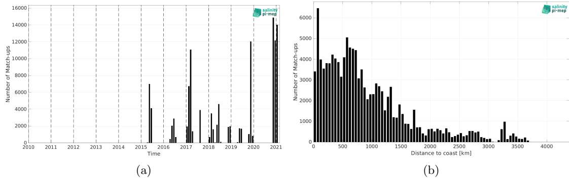
Figure 2: Number of match-ups between TSG (GOSUD-Sailing-ship) and SMAP SSS L2 v6 - 40 km (RSS) SSS as a function of time (a) and as function of the distance to coast (b) over the Mid-Low Latitudes 45N-45S Pi-MEP region and for the full satellite product period.
