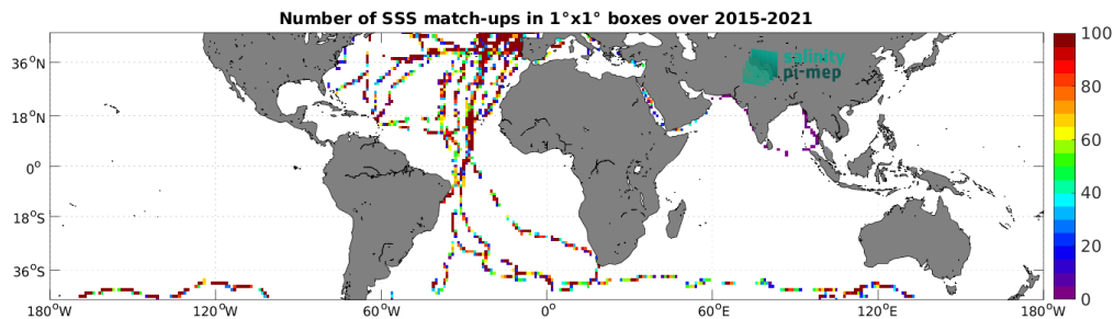
Figure 5: Number of SSS match-ups between TSG (GOSUD-Sailing-ship) SSS and the SMAP SSS L2 v6 - 40 km (RSS) SSS product for the Mid-Low Latitudes 45N-45S Pi-MEP region over 1^\circ \times 1^\circ boxes and for the full satellite product period.
