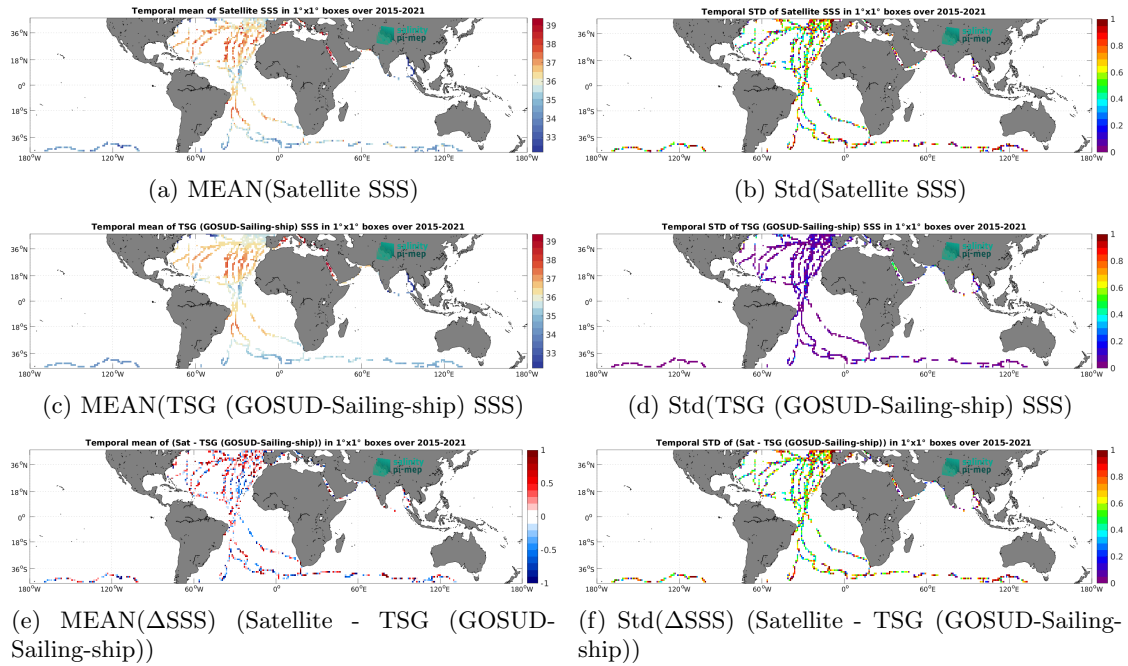
Figure 7: Temporal mean (left) and Std (right) of SSS from SMAP SSS L2 v6 - 40 km (RSS) (top), TSG (GOSUD-Sailing-ship) (middle), and of \Delta SSS (Satellite - TSG (GOSUD-Sailing-ship)). Only match-up pairs are used to generate these maps.
