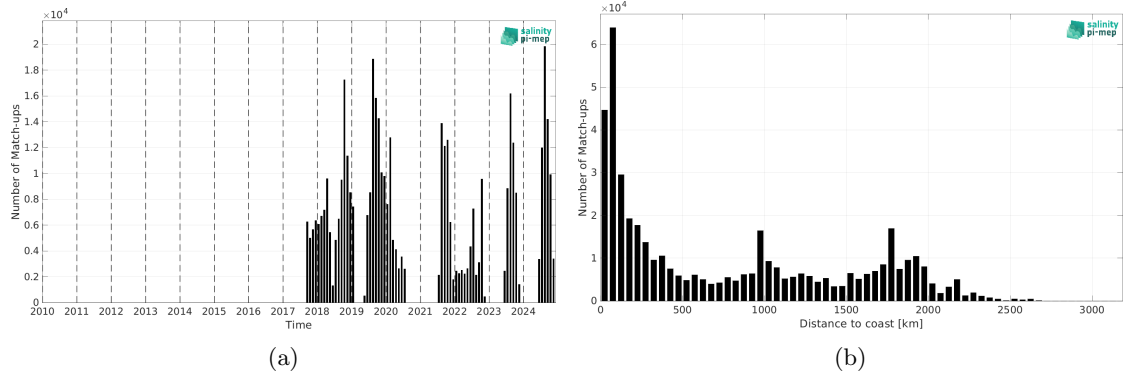
Figure 2: Number of match-ups between Saildrone and SMAP SSS L2 v6 - 40 km (RSS) SSS as a function of time (a) and as function of the distance to coast (b) over the Mid-Low Latitudes 45N-45S Pi-MEP region and for the full satellite product period.
