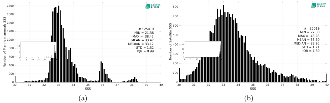
Figure 3: Histograms of SSS from Marine mammals (a) and SMAP SSS L2 v6 - 40 km (RSS) (b) considering all match-up pairs per bins of 0.1 over the Mid-Low Latitudes 45N-45S Pi-MEP region and for the full satellite product period.
