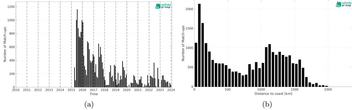
Figure 2: Number of match-ups between Marine mammals and SMAP SSS L2 v6 - 40 km (RSS) SSS as a function of time (a) and as function of the distance to coast (b) over the Mid-Low Latitudes 45N-45S Pi-MEP region and for the full satellite product period.
