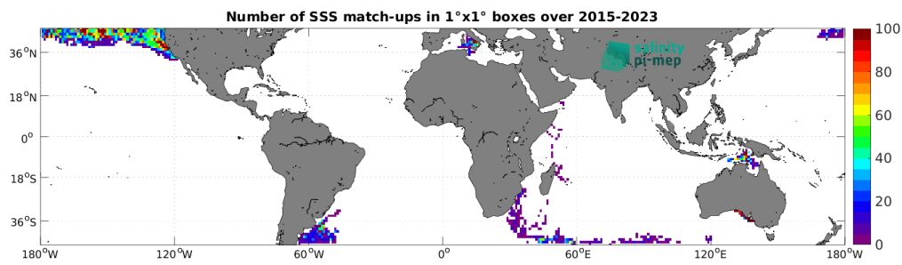
Figure 5: Number of SSS match-ups between Marine mammals SSS and the SMAP SSS L2 v6 - 40 km (RSS) SSS product for the Mid-Low Latitudes 45N-45S Pi-MEP region over 1^\circ \times 1^\circ boxes and for the full satellite product period.
