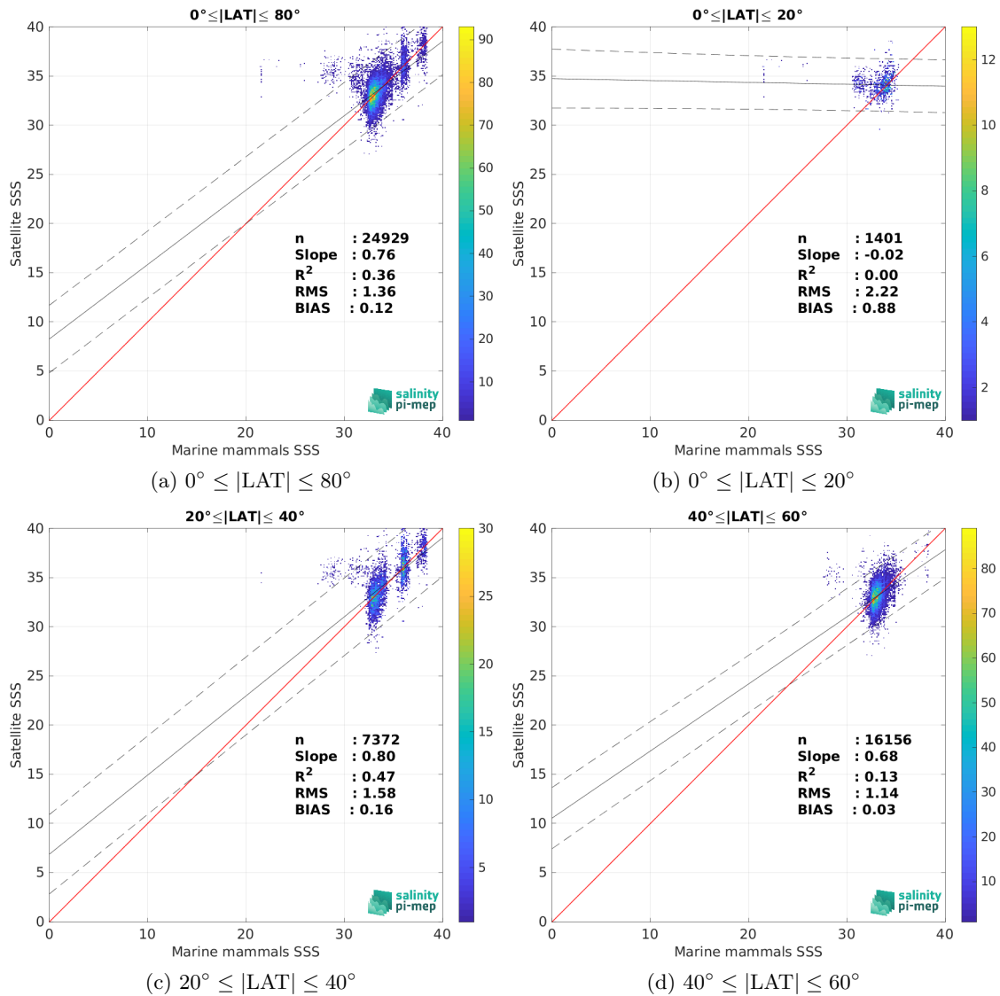
Figure 10: Contour maps of the concentration of SMAP SSS L2 v6 - 40 km (RSS) SSS (y-axis) versus Marine mammals SSS (x-axis) at match-up pairs for different latitude bands. For each plot, the red line shows x=y . The black thin and dashed lines indicate a linear fit through the data cloud and the \pm 95\% confidence levels, respectively. The number match-up pairs n , the slope and R^2 coefficient of the linear fit, the root mean square (RMS) and the mean bias between satellite and in situ data are indicated for each latitude band in each plots.
