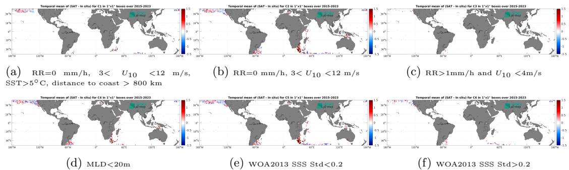
Figure 14: Temporal mean gridded over spatial boxes of size 1^\circ \times 1^\circ of \Delta\text{SSS} (SMAP SSS L2 v6 - 40 km (RSS) - Marine mammals) for 6 different subdatasets corresponding to:RR=0 mm/h, 3 < U_{10} < 12 m/s, SST>5°C, distance to coast > 800 km (a), RR=0 mm/h, 3 < U_{10} < 12 m/s (b), RR>1mm/h and U_{10} < 4 m/s (c),MLD<20m (d),WOA2013 SSS Std<0.2 (e),WOA2013 SSS Std>0.2 (f).
