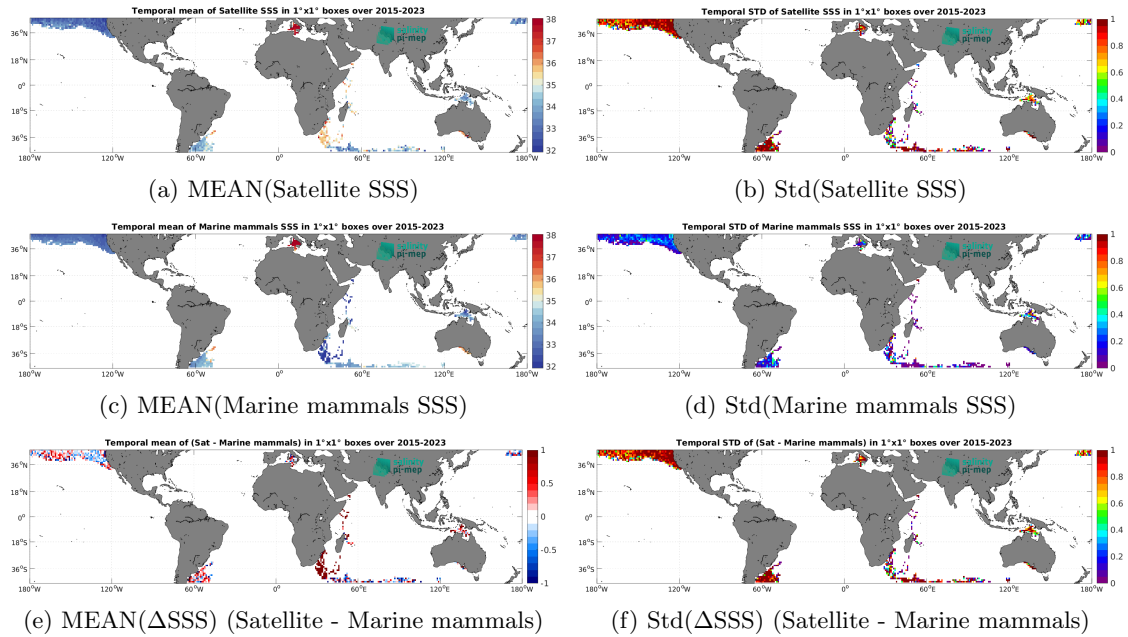
Figure 7: Temporal mean (left) and Std (right) of SSS from SMAP SSS L2 v6 - 40 km (RSS) (top), Marine mammals (middle), and of \Delta SSS (Satellite - Marine mammals). Only match-up pairs are used to generate these maps.
