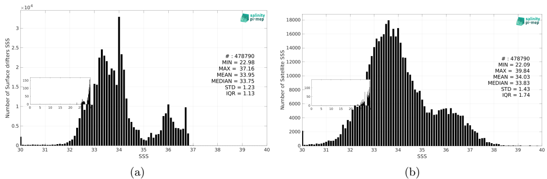
Figure 3: Histograms of SSS from Surface drifters (a) and SMAP SSS L2 v6 - 40 km (RSS) (b) considering all match-up pairs per bins of 0.1 over the Mid-Low Latitudes 45N-45S Pi-MEP region and for the full satellite product period.
