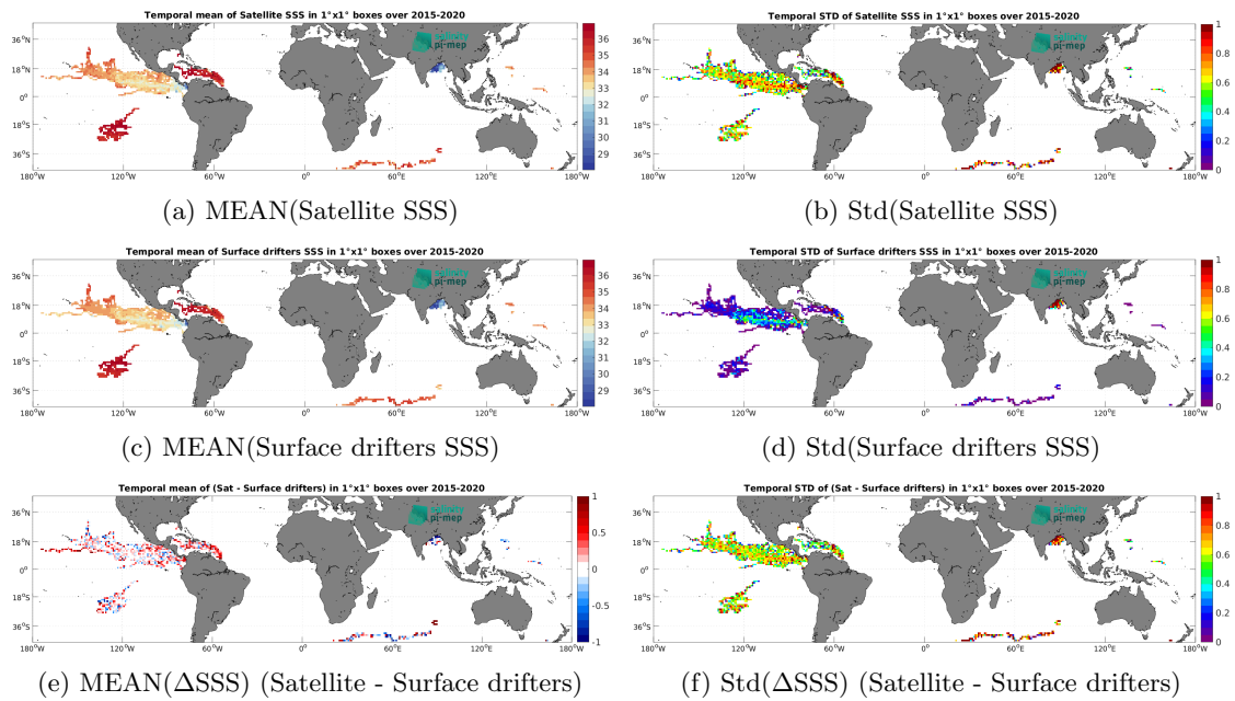
Figure 6: Temporal mean (left) and Std (right) of SSS from SMAP SSS L2 v6 - 40 km (RSS) (top), Surface drifters (middle), and of \Delta SSS (Satellite - Surface drifters). Only match-up pairs are used to generate these maps.
