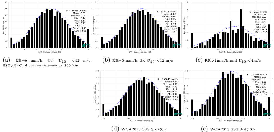
Figure 14: Normalized histogram of \Delta SSS (SMAP SSS L2 v6 - 40 km (RSS) - Surface drifters) for 5 different subdatasets corresponding to: RR=0 mm/h, 3 < U_{10} < 12 m/s, SST >5^\circ\text{C} , distance to coast > 800 km (a), RR=0 mm/h, 3 < U_{10} < 12 m/s (b), RR >1 mm/h and U_{10} < 4 m/s (c), WOA2013 SSS Std <0.2 (d), WOA2013 SSS Std >0.2 (e).
