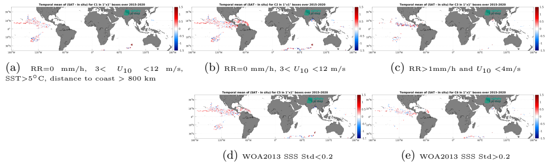
Figure 13: Temporal mean gridded over spatial boxes of size 1^\circ \times 1^\circ of \Delta SSS (SMAP SSS L2 v6 - 40 km (RSS) - Surface drifters) for 5 different subdatasets corresponding to:RR=0 mm/h, 3 < U_{10} < 12 m/s, SST >5^\circ\text{C} , distance to coast > 800 km (a), RR=0 mm/h, 3 < U_{10} < 12 m/s (b), RR >1 mm/h and U_{10} < 4 m/s (c), WOA2013 SSS Std <0.2 (d), WOA2013 SSS Std >0.2 (e).
