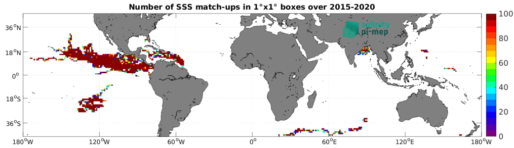
Figure 4: Number of SSS match-ups between Surface drifters SSS and the SMAP SSS L2 v6 - 40 km (RSS) SSS product for the Mid-Low Latitudes 45N-45S Pi-MEP region over 1^\circ \times 1^\circ boxes and for the full satellite product period.
