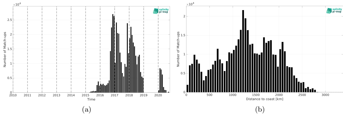
Figure 2: Number of match-ups between Surface drifters and SMAP SSS L2 v6 - 40 km (RSS) SSS as a function of time (a) and as function of the distance to coast (b) over the Mid-Low Latitudes 45N-45S Pi-MEP region and for the full satellite product period.
