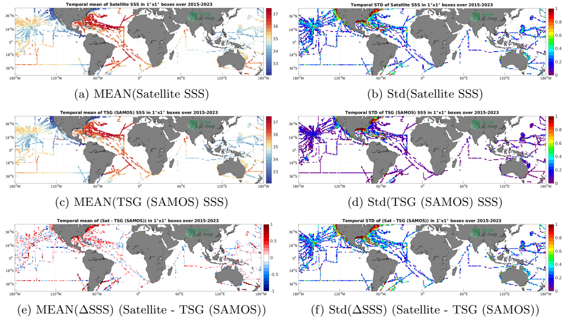
Figure 6: Temporal mean (left) and Std (right) of SSS from SMAP SSS L2 v5 (RSS) (top), TSG (SAMOS) (middle), and of \Delta SSS (Satellite - TSG (SAMOS)). Only match-up pairs are used to generate these maps.
