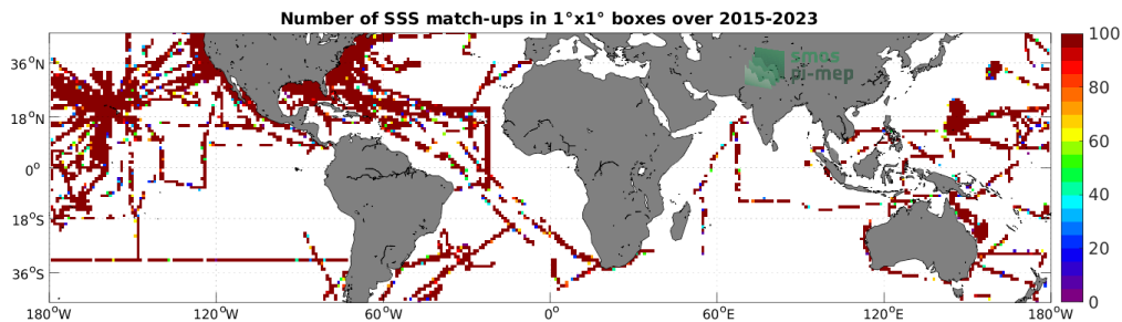
Figure 4: Number of SSS match-ups between TSG (SAMOS) SSS and the SMAP SSS L2 v5 (RSS) SSS product for the Mid-Low Latitudes 45N-45S Pi-MEP region over 1^\circ \times 1^\circ boxes and for the full satellite product period.
