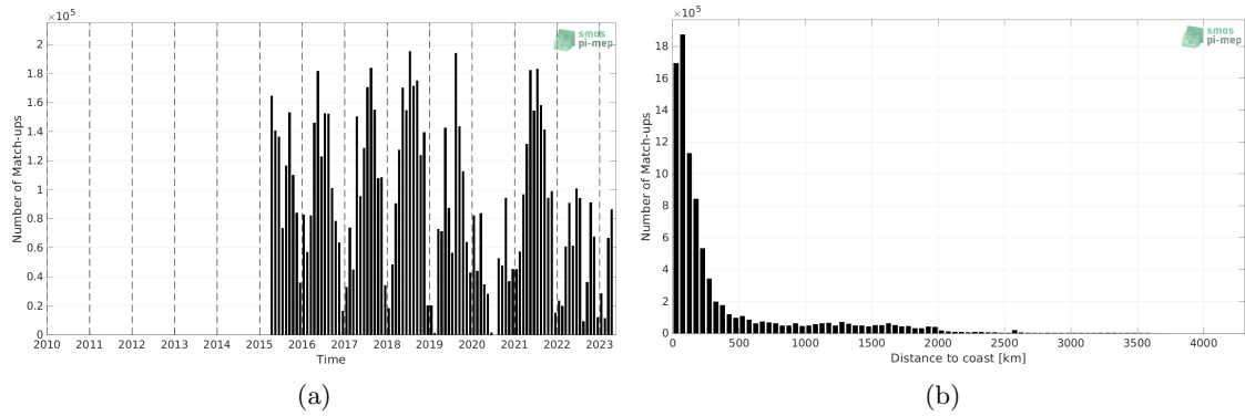
Figure 1: Number of match-ups between TSG (SAMOS) and SMAP SSS L2 v5 (RSS) SSS as a function of time (a) and as function of the distance to coast (b) over the Mid-Low Latitudes 45N-45S Pi-MEP region and for the full satellite product period.
