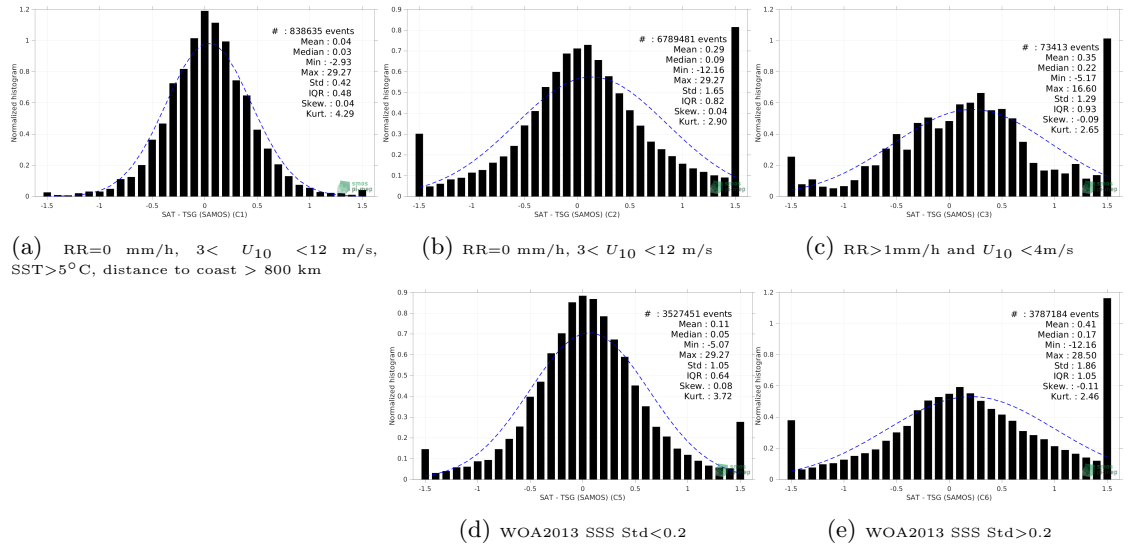
Figure 13: Normalized histogram of \Delta SSS (SMAP SSS L2 v5 (RSS) - TSG (SAMOS)) for 5 different subdatasets corresponding to: RR=0 mm/h, 3 < U_{10} < 12 m/s, SST >5^\circ\text{C} , distance to coast > 800 km (a), RR=0 mm/h, 3 < U_{10} < 12 m/s (b), RR >1 mm/h and U_{10} < 4 m/s (c), WOA2013 SSS Std <0.2 (d), WOA2013 SSS Std >0.2 (e).
