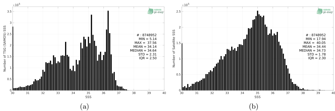
Figure 2: Histograms of SSS from TSG (SAMOS) (a) and SMAP SSS L2 v5 (RSS) (b) considering all match-up pairs per bins of 0.1 over the Mid-Low Latitudes 45N-45S Pi-MEP region and for the full satellite product period.
