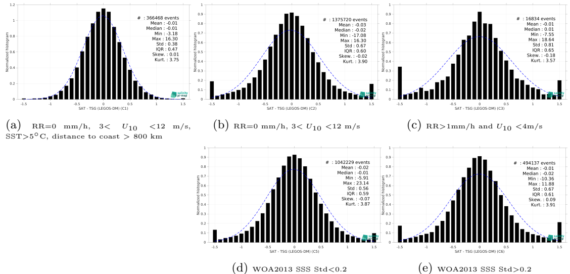
Figure 13: Normalized histogram of \Delta\text{SSS} (SMAP SSS L2 v5 (RSS) - TSG (LEGOS-DM)) for 5 different subdatasets corresponding to: RR=0 mm/h, 3 < U_{10} < 12 m/s, SST >5^\circ\text{C} , distance to coast > 800 km (a), RR=0 mm/h, 3 < U_{10} < 12 m/s (b), RR >1 mm/h and U_{10} < 4 m/s (c), WOA2013 SSS Std <0.2 (d), WOA2013 SSS Std >0.2 (e).
