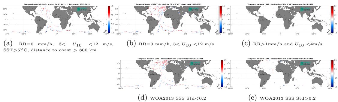
Figure 12: Temporal mean gridded over spatial boxes of size 1^\circ \times 1^\circ of \Delta\text{SSS} (SMAP SSS L2 v5 (RSS) - TSG (GOSUD-Sailing-ship)) for 5 different subdatasets corresponding to:RR=0 mm/h, 3 < U_{10} < 12 m/s, SST >5^\circ\text{C} , distance to coast > 800 km (a), RR=0 mm/h, 3 < U_{10} < 12 m/s (b), RR >1 mm/h and U_{10} < 4 m/s (c), WOA2013 SSS Std <0.2 (d), WOA2013 SSS Std >0.2 (e).
