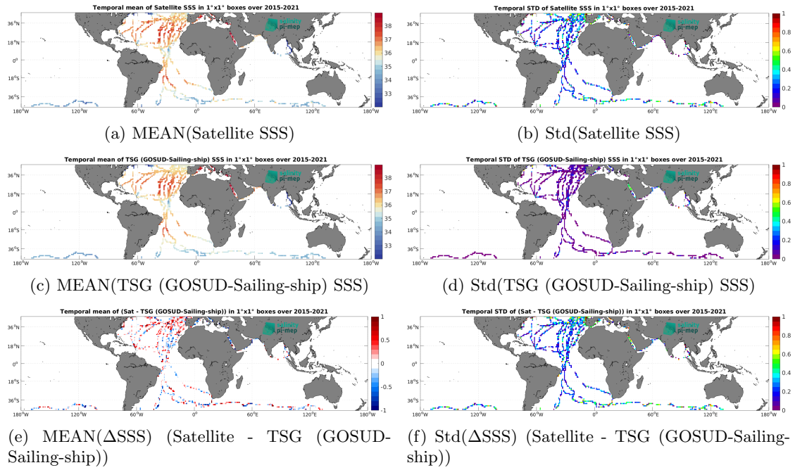
Figure 6: Temporal mean (left) and Std (right) of SSS from SMAP SSS L2 v5 (RSS) (top), TSG (GOSUD-Sailing-ship) (middle), and of \Delta SSS (Satellite - TSG (GOSUD-Sailing-ship)). Only match-up pairs are used to generate these maps.
