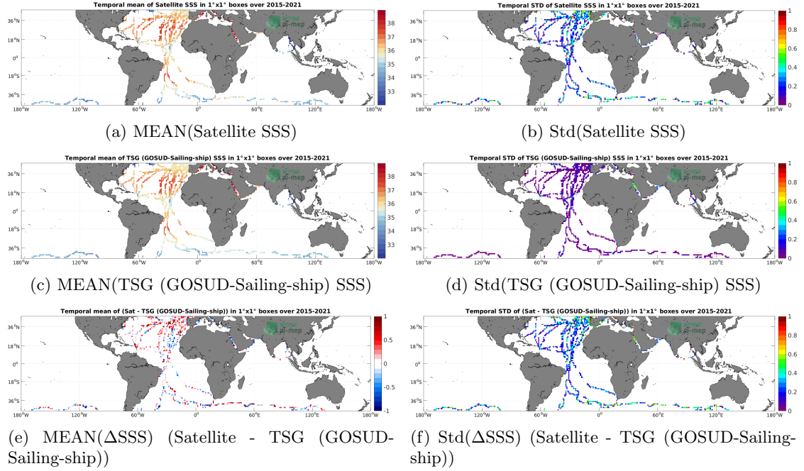
Figure 6: Temporal mean (left) and Std (right) of SSS from SMAP SSS L2 v5 (RSS) (top), TSG (GOSUD-Sailing-ship) (middle), and of \Delta SSS (Satellite - TSG (GOSUD-Sailing-ship)). Only match-up pairs are used to generate these maps.
