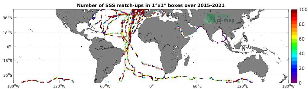
Figure 4: Number of SSS match-ups between TSG (GOSUD-Sailing-ship) SSS and the SMAP SSS L2 v5 (RSS) SSS product for the Mid-Low Latitudes 45N-45S Pi-MEP region over 1^\circ \times 1^\circ boxes and for the full satellite product period.
