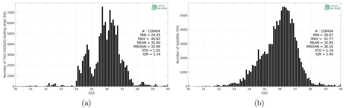
Figure 2: Histograms of SSS from TSG (GOSUD-Sailing-ship) (a) and SMAP SSS L2 v5 (RSS) (b) considering all match-up pairs per bins of 0.1 over the Mid-Low Latitudes 45N-45S Pi-MEP region and for the full satellite product period.
