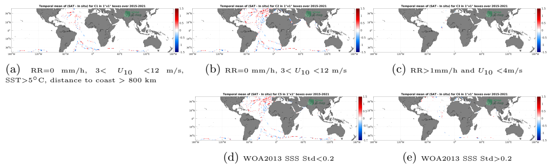
Figure 12: Temporal mean gridded over spatial boxes of size 1^\circ \times 1^\circ of \Delta SSS (SMAP SSS L2 v5 (RSS) - TSG (GOSUD-Sailing-ship)) for 5 different subdatasets corresponding to:RR=0 mm/h, 3 < U_{10} < 12 m/s, SST>5°C, distance to coast > 800 km (a), RR=0 mm/h, 3 < U_{10} < 12 m/s (b), RR>1mm/h and U_{10} < 4 m/s (c), WOA2013 SSS Std<0.2 (d), WOA2013 SSS Std>0.2 (e).
