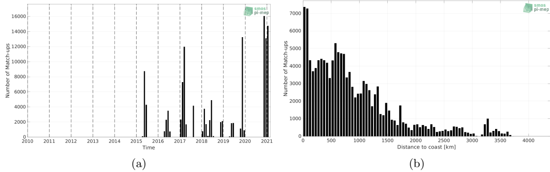
Figure 1: Number of match-ups between TSG (GOSUD-Sailing-ship) and SMAP SSS L2 v5 (RSS) SSS as a function of time (a) and as function of the distance to coast (b) over the Mid-Low Latitudes 45N-45S Pi-MEP region and for the full satellite product period.
