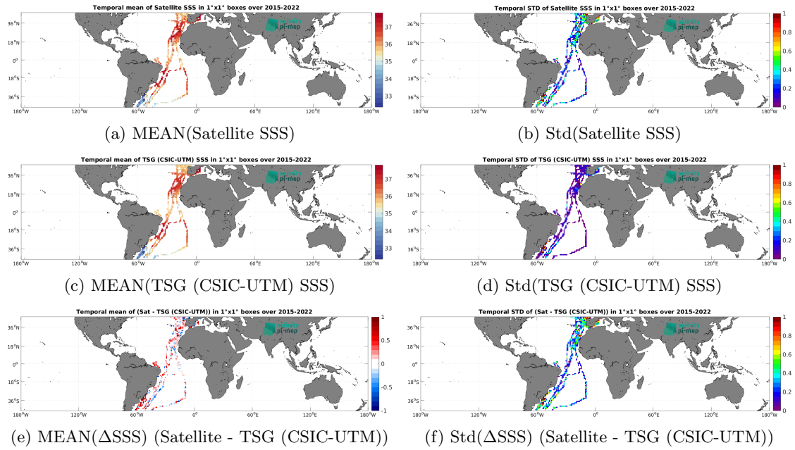
Figure 6: Temporal mean (left) and Std (right) of SSS from SMAP SSS L2 v5 (RSS) (top), TSG (CSIC-UTM) (middle), and of \Delta SSS (Satellite - TSG (CSIC-UTM)). Only match-up pairs are used to generate these maps.
