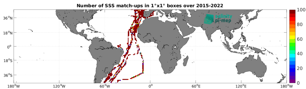
Figure 4: Number of SSS match-ups between TSG (CSIC-UTM) SSS and the SMAP SSS L2 v5 (RSS) SSS product for the Mid-Low Latitudes 45N-45S Pi-MEP region over 1^\circ \times 1^\circ boxes and for the full satellite product period.
