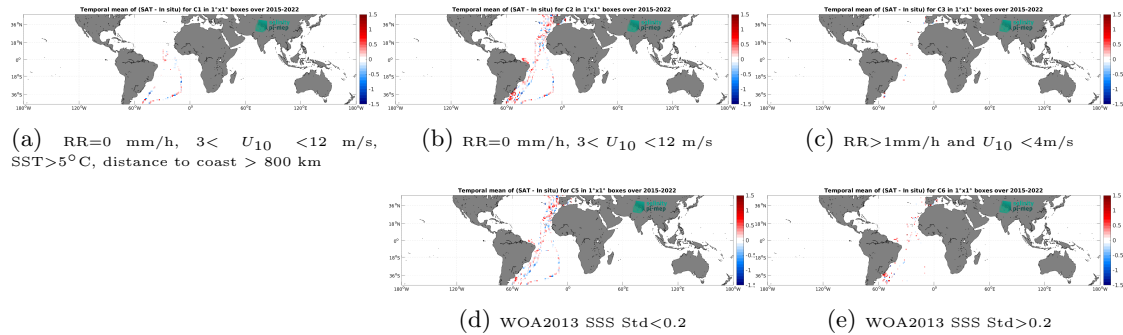
Figure 12: Temporal mean gridded over spatial boxes of size 1^\circ \times 1^\circ of \Delta SSS (SMAP SSS L2 v5 (RSS) - TSG (CSIC-UTM)) for 5 different subdatasets corresponding to:RR=0 mm/h, 3 < U_{10} < 12 m/s, SST >5^\circ C, distance to coast > 800 km (a), RR=0 mm/h, 3 < U_{10} < 12 m/s (b), RR >1 mm/h and U_{10} < 4 m/s (c), WOA2013 SSS Std <0.2 (d), WOA2013 SSS Std >0.2 (e).
