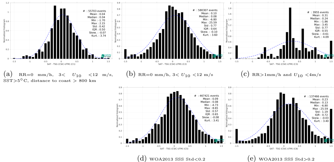
Figure 13: Normalized histogram of \Delta SSS (SMAP SSS L2 v5 (RSS) - TSG (CSIC-UTM)) for 5 different subdatasets corresponding to: RR=0 mm/h, 3 < U_{10} < 12 m/s, SST >5^\circ C, distance to coast > 800 km (a), RR=0 mm/h, 3 < U_{10} < 12 m/s (b), RR >1 mm/h and U_{10} < 4 m/s (c), WOA2013 SSS Std <0.2 (d), WOA2013 SSS Std >0.2 (e).
