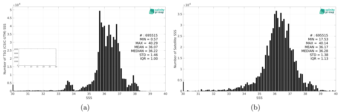
Figure 2: Histograms of SSS from TSG (CSIC-UTM) (a) and SMAP SSS L2 v5 (RSS) (b) considering all match-up pairs per bins of 0.1 over the Mid-Low Latitudes 45N-45S Pi-MEP region and for the full satellite product period.
