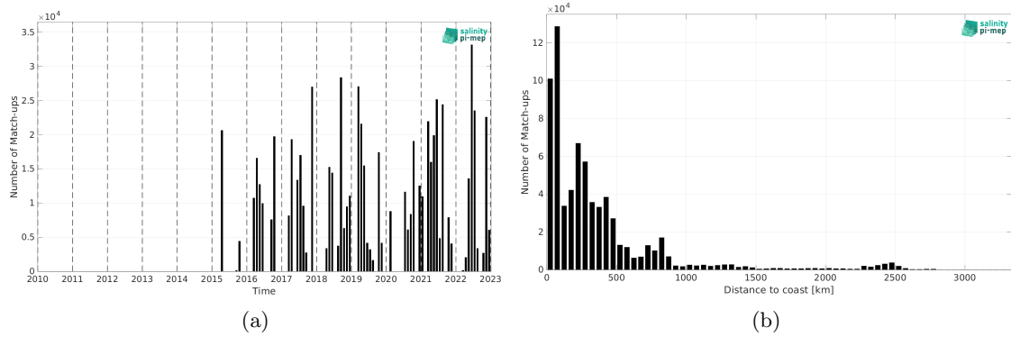
Figure 1: Number of match-ups between TSG (CSIC-UTM) and SMAP SSS L2 v5 (RSS) SSS as a function of time (a) and as function of the distance to coast (b) over the Mid-Low Latitudes 45N-45S Pi-MEP region and for the full satellite product period.
