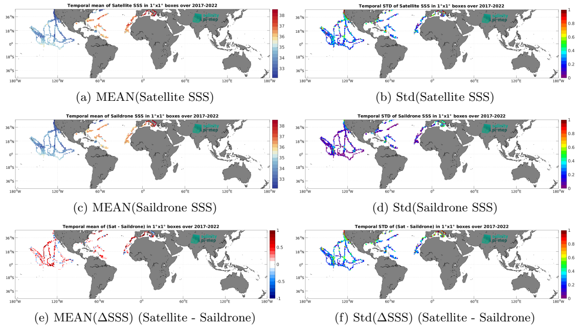
Figure 6: Temporal mean (left) and Std (right) of SSS from SMAP SSS L2 v5 (RSS) (top), Saildrone (middle), and of \Delta SSS (Satellite - Saildrone). Only match-up pairs are used to generate these maps.
