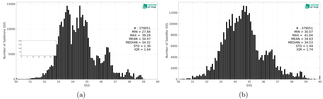
Figure 2: Histograms of SSS from Sairdrone (a) and SMAP SSS L2 v5 (RSS) (b) considering all match-up pairs per bins of 0.1 over the Mid-Low Latitudes 45N-45S Pi-MEP region and for the full satellite product period.
