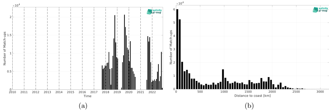
Figure 1: Number of match-ups between Sairdrone and SMAP SSS L2 v5 (RSS) SSS as a function of time (a) and as function of the distance to coast (b) over the Mid-Low Latitudes 45N-45S Pi-MEP region and for the full satellite product period.
