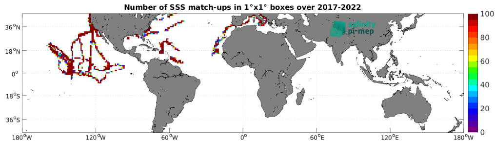
Figure 4: Number of SSS match-ups between Saildrone SSS and the SMAP SSS L2 v5 (RSS) SSS product for the Mid-Low Latitudes 45N-45S Pi-MEP region over 1^\circ \times 1^\circ boxes and for the full satellite product period.
