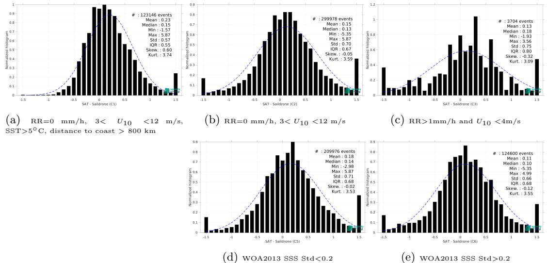
Figure 13: Normalized histogram of \Delta SSS (SMAP SSS L2 v5 (RSS) - Saildrone) for 5 different subdatasets corresponding to: RR=0 mm/h, 3 < U_{10} < 12 m/s, SST >5^\circ\text{C} , distance to coast > 800 km (a), RR=0 mm/h, 3 < U_{10} < 12 m/s (b), RR >1 mm/h and U_{10} < 4 m/s (c), WOA2013 SSS Std <0.2 (d), WOA2013 SSS Std >0.2 (e).
