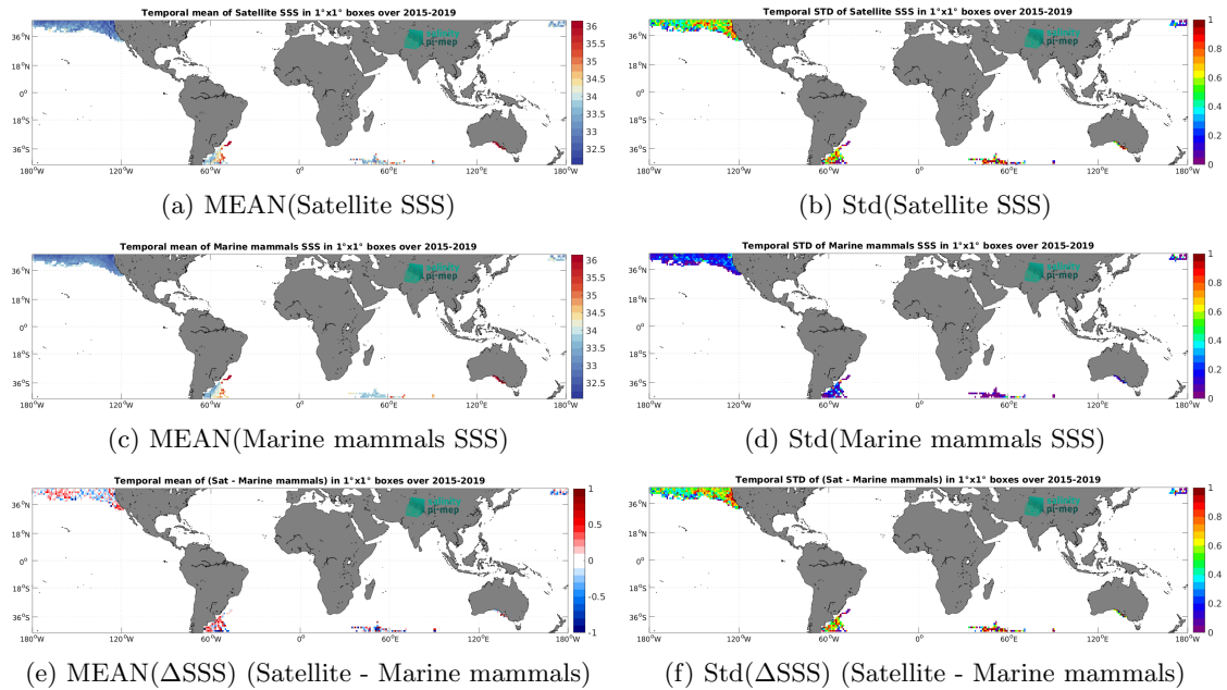
Figure 6: Temporal mean (left) and Std (right) of SSS from SMAP SSS L2 v5 (RSS) (top), Marine mammals (middle), and of \Delta SSS (Satellite - Marine mammals). Only match-up pairs are used to generate these maps.
