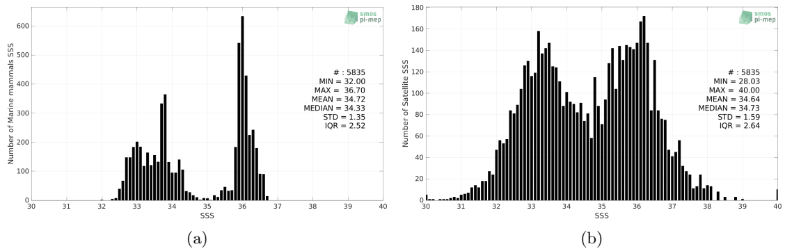
Figure 2: Histograms of SSS from Marine mammals (a) and SMAP SSS L2 v5 (RSS) (b) considering all match-up pairs per bins of 0.1 over the Mid-Low Latitudes 45N-45S Pi-MEP region and for the full satellite product period.
