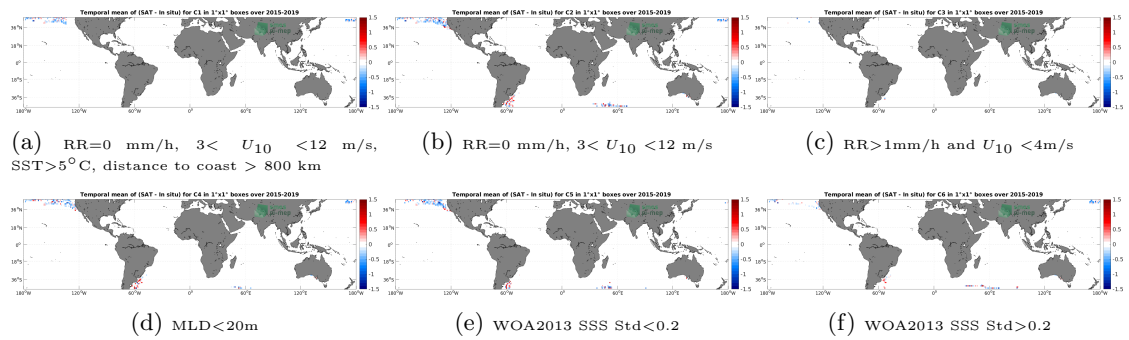
Figure 12: Temporal mean gridded over spatial boxes of size 1^\circ \times 1^\circ of \Delta SSS (SMAP SSS L2 v5 (RSS) - Marine mammals) for 6 different subdatasets corresponding to:RR=0 mm/h, 3 < U_{10} < 12 m/s, SST>5°C, distance to coast > 800 km (a), RR=0 mm/h, 3 < U_{10} < 12 m/s (b), RR>1mm/h and U_{10} < 4 m/s (c),MLD<20m (d),WOA2013 SSS Std<0.2 (e),WOA2013 SSS Std>0.2 (f).
