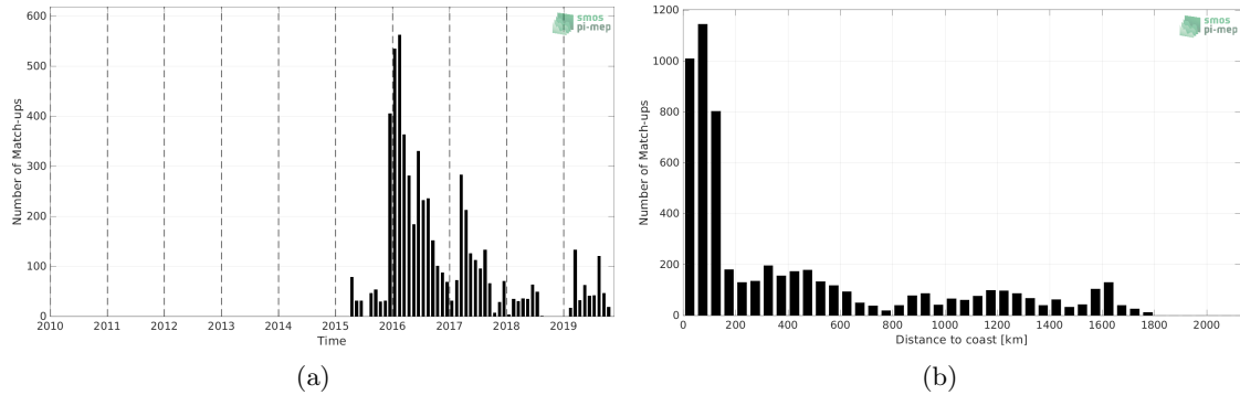
Figure 1: Number of match-ups between Marine mammals and SMAP SSS L2 v5 (RSS) SSS as a function of time (a) and as function of the distance to coast (b) over the Mid-Low Latitudes 45N-45S Pi-MEP region and for the full satellite product period.
