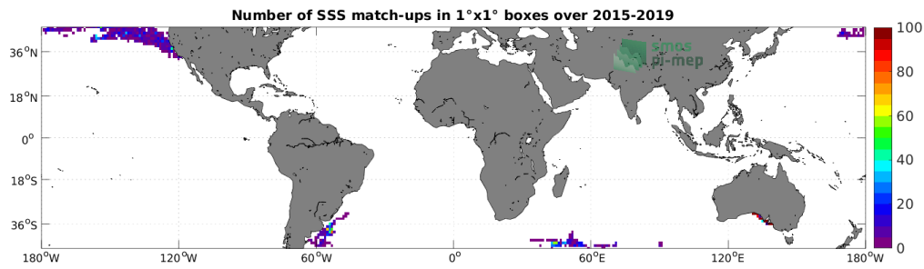
Figure 4: Number of SSS match-ups between Marine mammals SSS and the SMAP SSS L2 v5 (RSS) SSS product for the Mid-Low Latitudes 45N-45S Pi-MEP region over 1^\circ \times 1^\circ boxes and for the full satellite product period.
