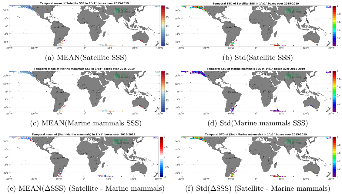
Figure 6: Temporal mean (left) and Std (right) of SSS from SMAP SSS L2 v5 (RSS) (top), Marine mammals (middle), and of \Delta SSS (Satellite - Marine mammals). Only match-up pairs are used to generate these maps.
