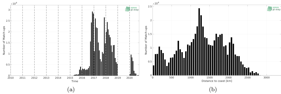
Figure 1: Number of match-ups between Surface drifters and SMAP SSS L2 v5 (RSS) SSS as a function of time (a) and as function of the distance to coast (b) over the Mid-Low Latitudes 45N-45S Pi-MEP region and for the full satellite product period.
