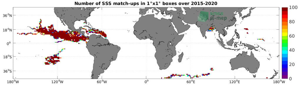
Figure 3: Number of SSS match-ups between Surface drifters SSS and the SMAP SSS L2 v5 (RSS) SSS product for the Mid-Low Latitudes 45N-45S Pi-MEP region over 1^\circ \times 1^\circ boxes and for the full satellite product period.
