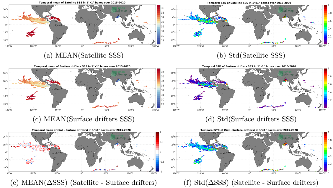
Figure 5: Temporal mean (left) and Std (right) of SSS from SMAP SSS L2 v5 (RSS) (top), Surface drifters (middle), and of \Delta SSS (Satellite - Surface drifters). Only match-up pairs are used to generate these maps.
