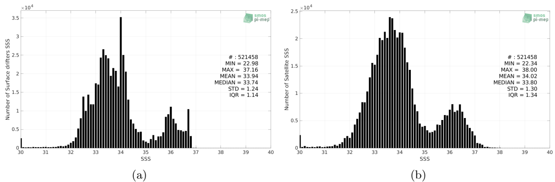
Figure 2: Histograms of SSS from Surface drifters (a) and SMAP SSS L2 v5 (RSS) (b) considering all match-up pairs per bins of 0.1 over the Mid-Low Latitudes 45N-45S Pi-MEP region and for the full satellite product period.
