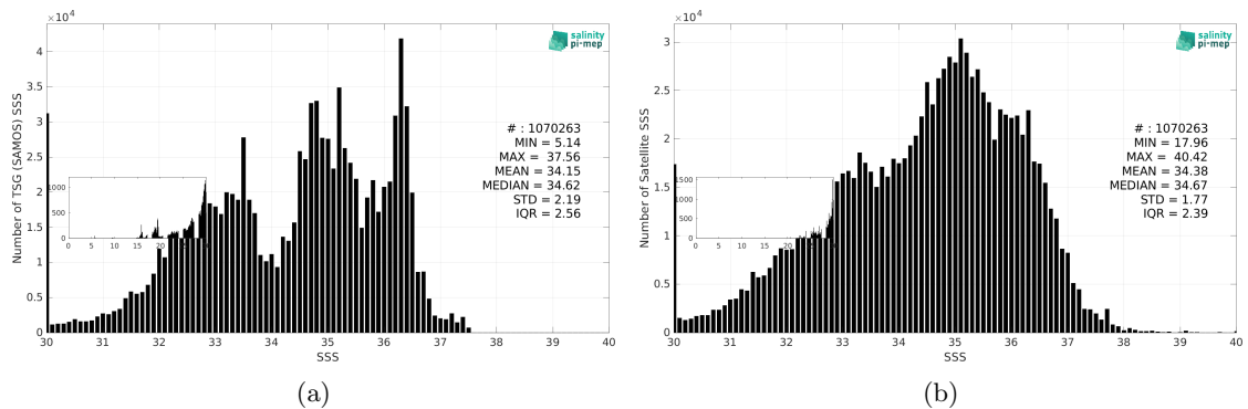
Figure 3: Histograms of SSS from TSG (SAMOS) (a) and SMAP SSS L2 v5.3 (RSS) (b) considering all match-up pairs per bins of 0.1 over the Mid-Low Latitudes 45N-45S Pi-MEP region and for the full satellite product period.
