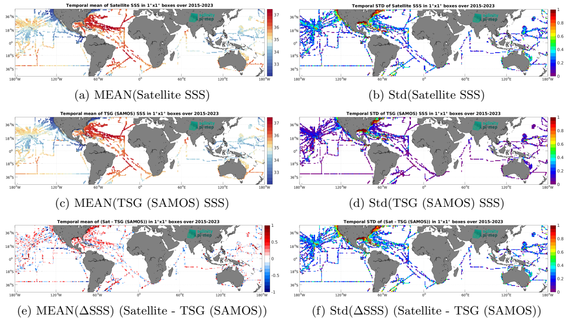
Figure 7: Temporal mean (left) and Std (right) of SSS from SMAP SSS L2 v5.3 (RSS) (top), TSG (SAMOS) (middle), and of \Delta SSS (Satellite - TSG (SAMOS)). Only match-up pairs are used to generate these maps.
