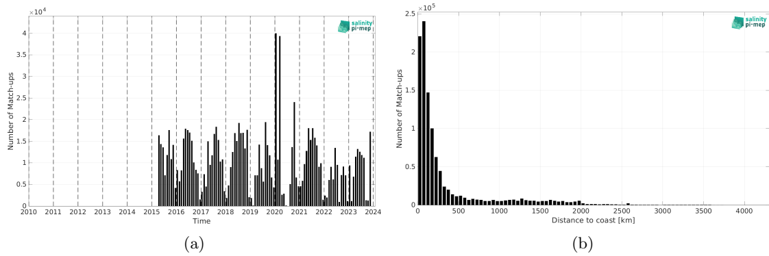
Figure 2: Number of match-ups between TSG (SAMOS) and SMAP SSS L2 v5.3 (RSS) SSS as a function of time (a) and as function of the distance to coast (b) over the Mid-Low Latitudes 45N-45S Pi-MEP region and for the full satellite product period.
