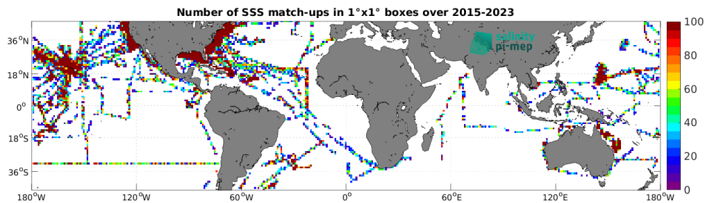
Figure 5: Number of SSS match-ups between TSG (SAMOS) SSS and the SMAP SSS L2 v5.3 (RSS) SSS product for the Mid-Low Latitudes 45N-45S Pi-MEP region over 1^\circ \times 1^\circ boxes and for the full satellite product period.
