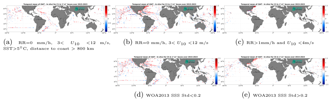
Figure 14: Temporal mean gridded over spatial boxes of size 1^\circ \times 1^\circ of \Delta SSS (SMAP SSS L2 v5.3 (RSS) - TSG (SAMOS)) for 5 different subdatasets corresponding to: RR=0 mm/h, 3 < U_{10} < 12 m/s, SST > 5°C, distance to coast > 800 km (a), RR=0 mm/h, 3 < U_{10} < 12 m/s (b), RR > 1mm/h and U_{10} < 4 m/s (c), WOA2013 SSS Std < 0.2 (d), WOA2013 SSS Std > 0.2 (e).
