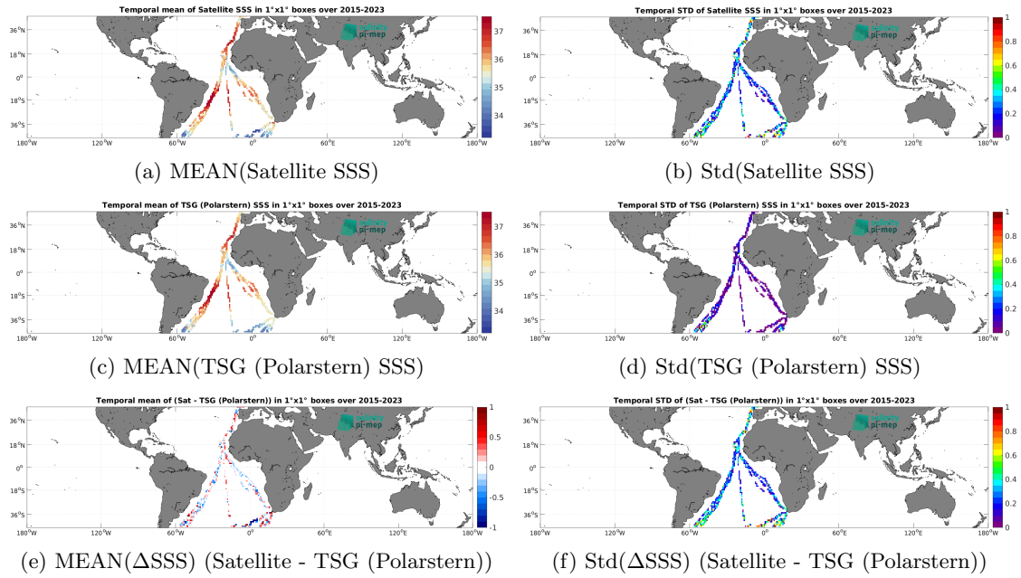
Figure 7: Temporal mean (left) and Std (right) of SSS from SMAP SSS L2 v5.3 (RSS) (top), TSG (Polarstern) (middle), and of \Delta SSS (Satellite - TSG (Polarstern)). Only match-up pairs are used to generate these maps.
