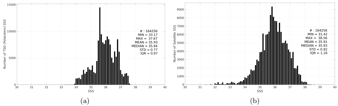
Figure 3: Histograms of SSS from TSG (Polarstern) (a) and SMAP SSS L2 v5.3 (RSS) (b) considering all match-up pairs per bins of 0.1 over the Mid-Low Latitudes 45N-45S Pi-MEP region and for the full satellite product period.
