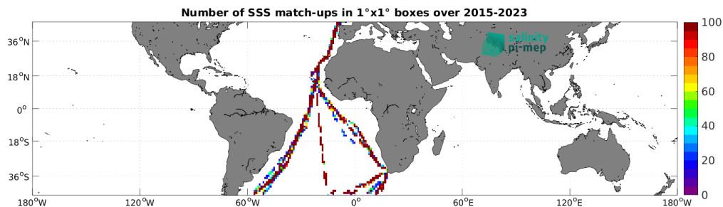
Figure 5: Number of SSS match-ups between TSG (Polarstern) SSS and the SMAP SSS L2 v5.3 (RSS) SSS product for the Mid-Low Latitudes 45N-45S Pi-MEP region over 1^\circ \times 1^\circ boxes and for the full satellite product period.
