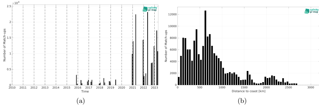
Figure 2: Number of match-ups between TSG (Polarstern) and SMAP SSS L2 v5.3 (RSS) SSS as a function of time (a) and as function of the distance to coast (b) over the Mid-Low Latitudes 45N-45S Pi-MEP region and for the full satellite product period.
