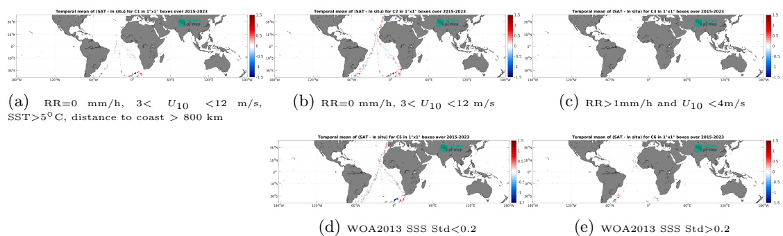
Figure 14: Temporal mean gridded over spatial boxes of size 1^\circ \times 1^\circ of \Delta\text{SSS} (SMAP SSS L2 v5.3 (RSS) - TSG (Polarstern)) for 5 different subdatasets corresponding to: RR=0 mm/h, 3 < U_{10} < 12 m/s, SST > 5°C, distance to coast > 800 km (a), RR=0 mm/h, 3 < U_{10} < 12 m/s (b), RR > 1mm/h and U_{10} < 4 m/s (c), WOA2013 SSS Std < 0.2 (d), WOA2013 SSS Std > 0.2 (e).
