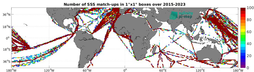
Figure 5: Number of SSS match-ups between TSG (LEGOS-DM) SSS and the SMAP SSS L2 v5.3 (RSS) SSS product for the Mid-Low Latitudes 45N-45S Pi-MEP region over 1^\circ \times 1^\circ boxes and for the full satellite product period.
