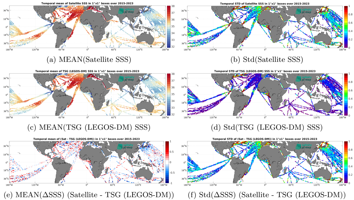
Figure 7: Temporal mean (left) and Std (right) of SSS from SMAP SSS L2 v5.3 (RSS) (top), TSG (LEGOS-DM) (middle), and of \Delta SSS (Satellite - TSG (LEGOS-DM)). Only match-up pairs are used to generate these maps.
