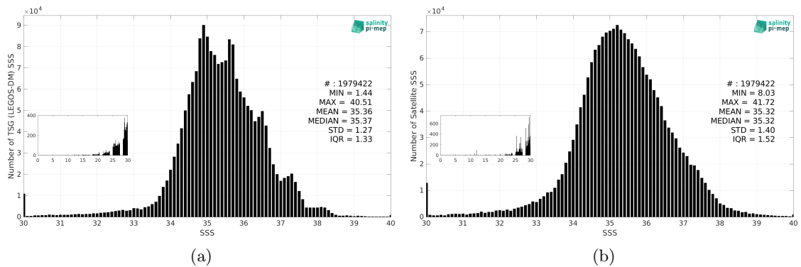
Figure 3: Histograms of SSS from TSG (LEGOS-DM) (a) and SMAP SSS L2 v5.3 (RSS) (b) considering all match-up pairs per bins of 0.1 over the Mid-Low Latitudes 45N-45S Pi-MEP region and for the full satellite product period.
