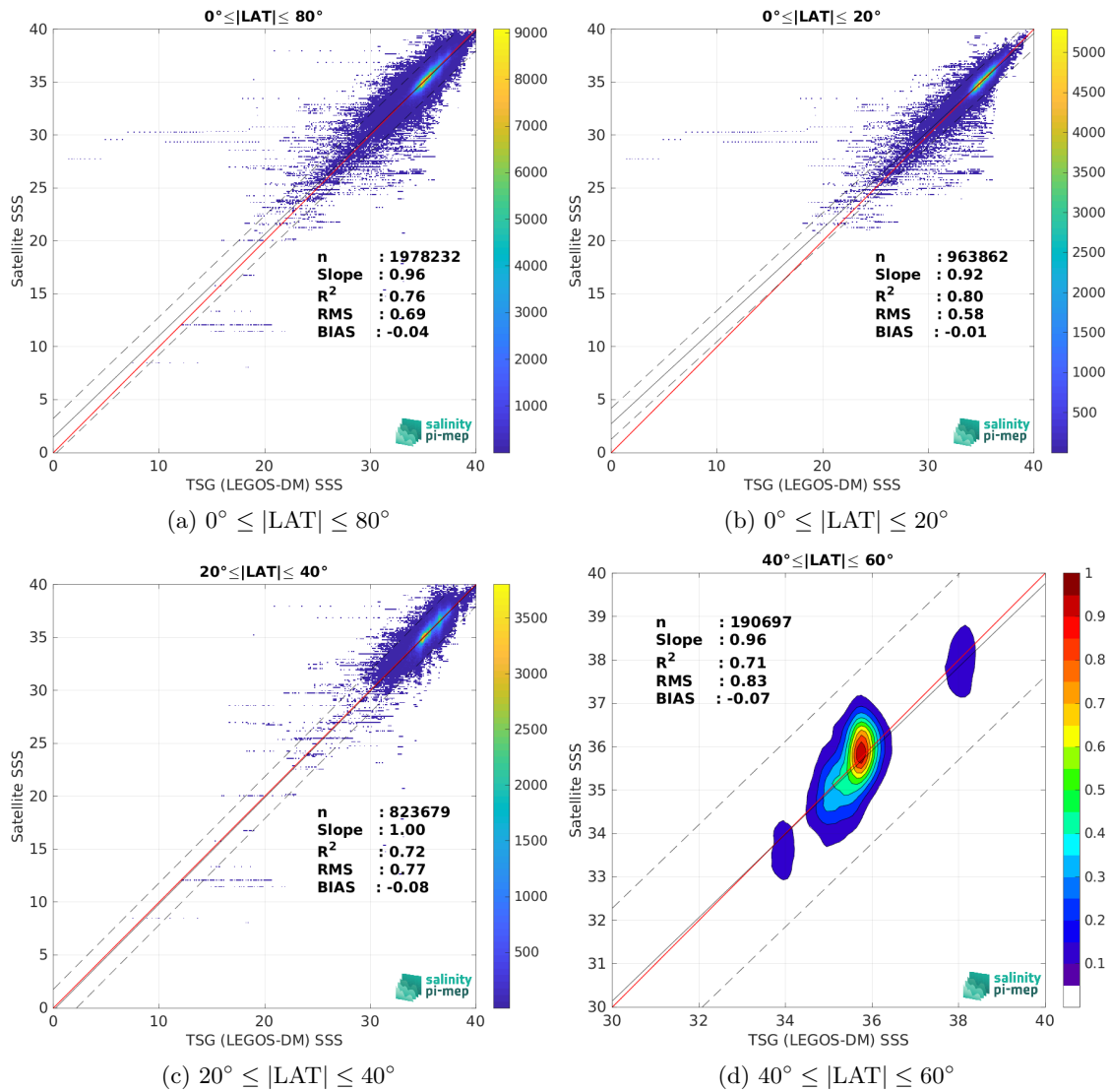
Figure 10: Contour maps of the concentration of SMAP SSS L2 v5.3 (RSS) SSS (y-axis) versus TSG (LEGOS-DM) SSS (x-axis) at match-up pairs for different latitude bands. For each plot, the red line shows x=y . The black thin and dashed lines indicate a linear fit through the data cloud and the \pm 95\% confidence levels, respectively. The number match-up pairs n , the slope and R^2 coefficient of the linear fit, the root mean square (RMS) and the mean bias between satellite and in situ data are indicated for each latitude band in each plots.
