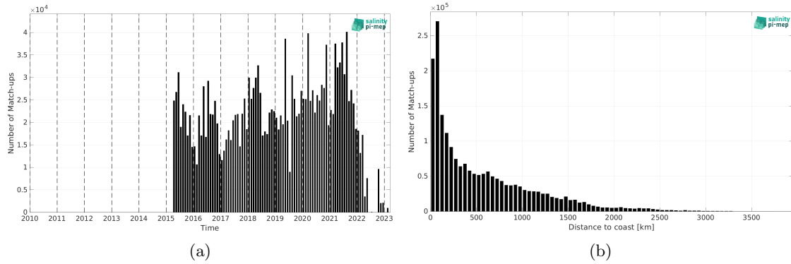
Figure 2: Number of match-ups between TSG (LEGOS-DM) and SMAP SSS L2 v5.3 (RSS) SSS as a function of time (a) and as function of the distance to coast (b) over the Mid-Low Latitudes 45N-45S Pi-MEP region and for the full satellite product period.
