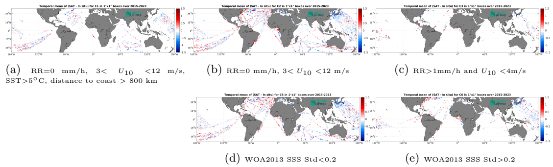
Figure 14: Temporal mean gridded over spatial boxes of size 1^\circ \times 1^\circ of \Delta SSS (SMAP SSS L2 v5.3 (RSS) - TSG (LEGOS-DM)) for 5 different subdatasets corresponding to: RR=0 mm/h, 3 < U_{10} < 12 m/s, SST > 5°C, distance to coast > 800 km (a), RR=0 mm/h, 3 < U_{10} < 12 m/s (b), RR > 1mm/h and U_{10} < 4 m/s (c), WOA2013 SSS Std < 0.2 (d), WOA2013 SSS Std > 0.2 (e).
