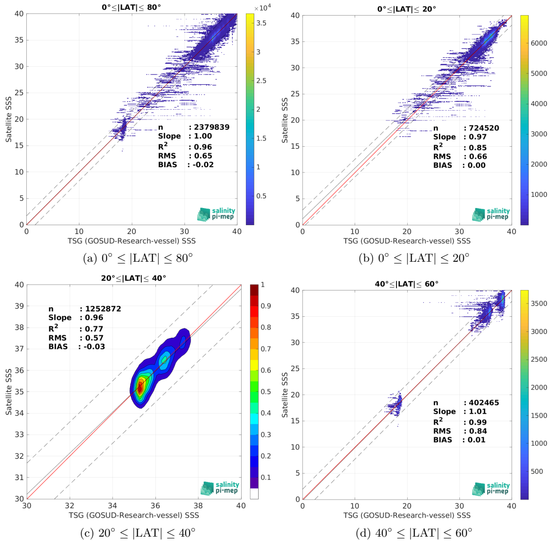
Figure 10: Contour maps of the concentration of SMAP SSS L2 v5.3 (RSS) SSS (y-axis) versus TSG (GOSUD-Research-vessel) SSS (x-axis) at match-up pairs for different latitude bands. For each plot, the red line shows x=y . The black thin and dashed lines indicate a linear fit through the data cloud and the \pm 95\% confidence levels, respectively. The number match-up pairs n , the slope and R^2 coefficient of the linear fit, the root mean square (RMS) and the mean bias between satellite and in situ data are indicated for each latitude band in each plots.
