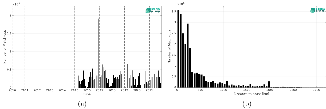
Figure 2: Number of match-ups between TSG (GOSUD-Research-vessel) and SMAP SSS L2 v5.3 (RSS) SSS as a function of time (a) and as function of the distance to coast (b) over the Mid-Low Latitudes 45N-45S Pi-MEP region and for the full satellite product period.
