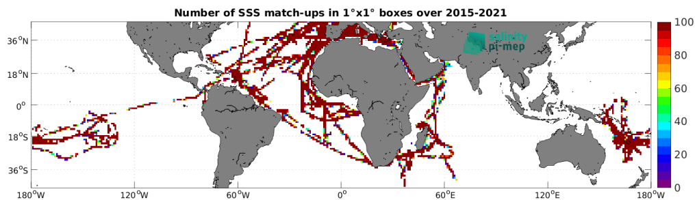
Figure 5: Number of SSS match-ups between TSG (GOSUD-Research-vessel) SSS and the SMAP SSS L2 v5.3 (RSS) SSS product for the Mid-Low Latitudes 45N-45S Pi-MEP region over 1^\circ \times 1^\circ boxes and for the full satellite product period.
