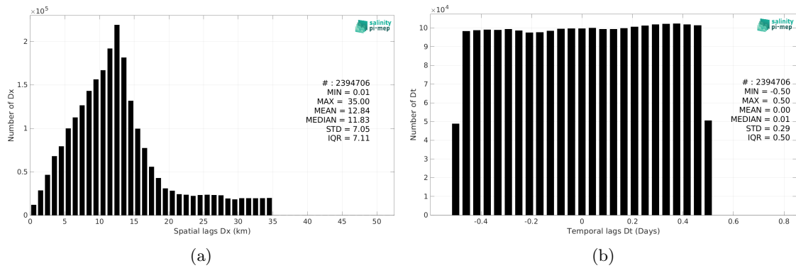
Figure 6: Histograms of the spatial (a) and temporal (b) lags between the location/time of the TSG (GOSUD-Research-vessel) measurement and the date of the corresponding SMAP SSS L2 v5.3 (RSS) SSS pixel.
