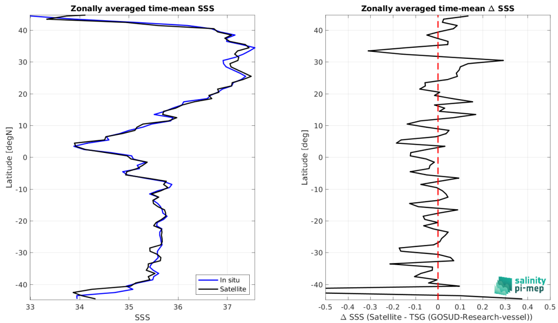
Figure 9: Left panel: Zonal mean SSS from SMAP SSS L2 v5.3 (RSS) satellite product (black) and from TSG (GOSUD-Research-vessel) (blue). Right panel: Zonal mean of \Delta SSS (Satellite - TSG (GOSUD-Research-vessel)) for all the collected Pi-MEP match-up pairs estimated over the full satellite product period.
