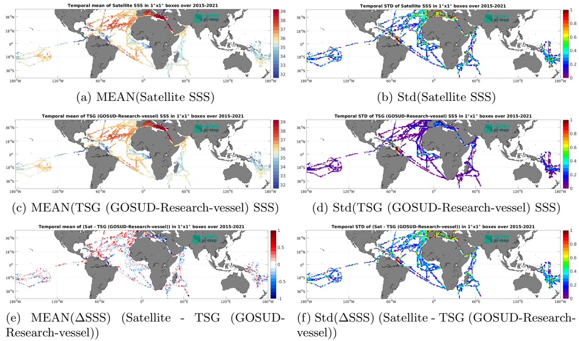
Figure 7: Temporal mean (left) and Std (right) of SSS from SMAP SSS L2 v5.3 (RSS) (top), TSG (GOSUD-Research-vessel) (middle), and of \Delta SSS (Satellite - TSG (GOSUD-Research-vessel)). Only match-up pairs are used to generate these maps.
