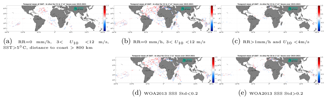
Figure 14: Temporal mean gridded over spatial boxes of size 1^\circ \times 1^\circ of \Delta SSS (SMAP SSS L2 v5.3 (RSS) - TSG (GOSUD-Research-vessel)) for 5 different subdatasets corresponding to: RR=0 mm/h, 3 < U_{10} < 12 m/s, SST > 5^\circ\text{C} , distance to coast > 800 km (a), RR=0 mm/h, 3 < U_{10} < 12 m/s (b), RR > 1\text{mm/h} and U_{10} < 4\text{m/s} (c), WOA2013 SSS Std < 0.2 (d), WOA2013 SSS Std > 0.2 (e).
