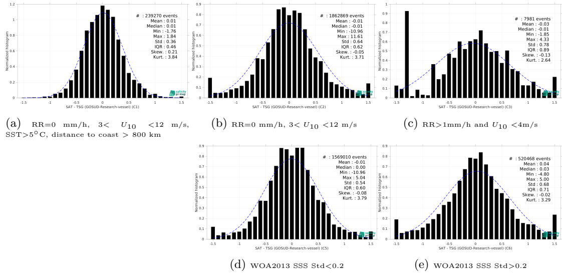
Figure 15: Normalized histogram of \Delta SSS (SMAP SSS L2 v5.3 (RSS) - TSG (GOSUD-Research-vessel)) for 5 different subdatasets corresponding to: RR=0 mm/h, 3 < U_{10} < 12 m/s, SST > 5°C, distance to coast > 800 km (a), RR=0 mm/h, 3 < U_{10} < 12 m/s (b), RR > 1mm/h and U_{10} < 4 m/s (c), WOA2013 SSS Std < 0.2 (d), WOA2013 SSS Std > 0.2 (e).
