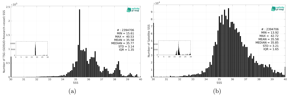
Figure 3: Histograms of SSS from TSG (GOSUD-Research-vessel) (a) and SMAP SSS L2 v5.3 (RSS) (b) considering all match-up pairs per bins of 0.1 over the Mid-Low Latitudes 45N-45S Pi-MEP region and for the full satellite product period.
