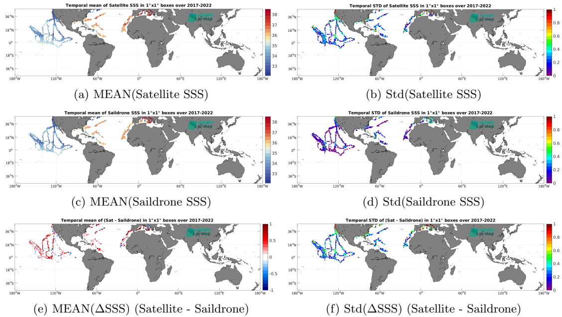
Figure 7: Temporal mean (left) and Std (right) of SSS from SMAP SSS L2 v5.3 (RSS) (top), Saildrone (middle), and of \Delta SSS (Satellite - Saildrone). Only match-up pairs are used to generate these maps.
