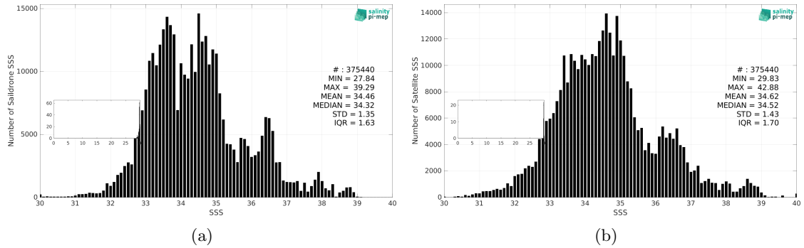
Figure 3: Histograms of SSS from Saildrone (a) and SMAP SSS L2 v5.3 (RSS) (b) considering all match-up pairs per bins of 0.1 over the Mid-Low Latitudes 45N-45S Pi-MEP region and for the full satellite product period.
