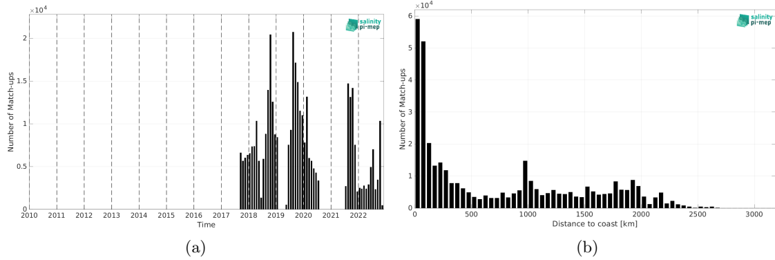
Figure 2: Number of match-ups between Saildrone and SMAP SSS L2 v5.3 (RSS) SSS as a function of time (a) and as function of the distance to coast (b) over the Mid-Low Latitudes 45N-45S Pi-MEP region and for the full satellite product period.
