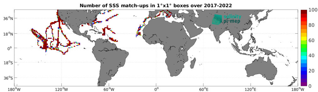
Figure 5: Number of SSS match-ups between Saildrone SSS and the SMAP SSS L2 v5.3 (RSS) SSS product for the Mid-Low Latitudes 45N-45S Pi-MEP region over 1^\circ \times 1^\circ boxes and for the full satellite product period.
