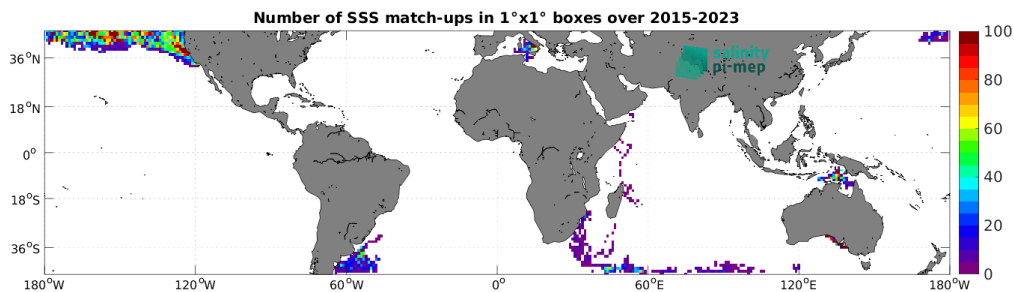
Figure 5: Number of SSS match-ups between Marine mammals SSS and the SMAP SSS L2 v5.3 (RSS) SSS product for the Mid-Low Latitudes 45N-45S Pi-MEP region over 1^\circ \times 1^\circ boxes and for the full satellite product period.
