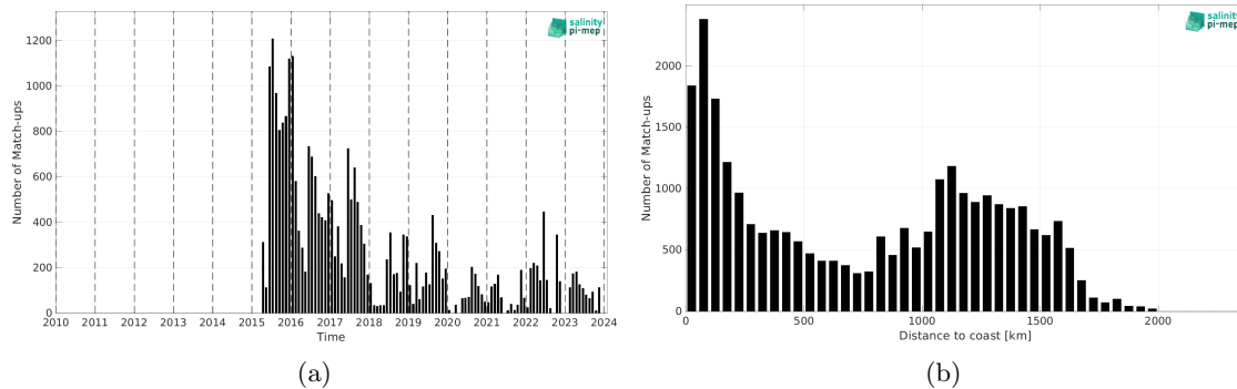
Figure 2: Number of match-ups between Marine mammals and SMAP SSS L2 v5.3 (RSS) SSS as a function of time (a) and as function of the distance to coast (b) over the Mid-Low Latitudes 45N-45S Pi-MEP region and for the full satellite product period.
