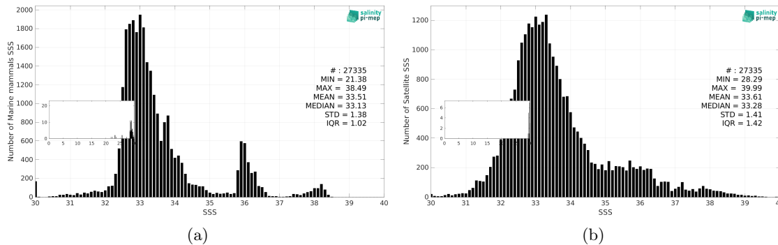
Figure 3: Histograms of SSS from Marine mammals (a) and SMAP SSS L2 v5.3 (RSS) (b) considering all match-up pairs per bins of 0.1 over the Mid-Low Latitudes 45N-45S Pi-MEP region and for the full satellite product period.
