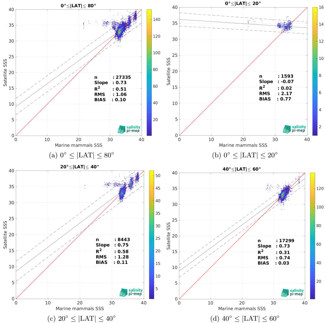
Figure 10: Contour maps of the concentration of SMAP SSS L2 v5.3 (RSS) SSS (y-axis) versus Marine mammals SSS (x-axis) at match-up pairs for different latitude bands. For each plot, the red line shows x=y . The black thin and dashed lines indicate a linear fit through the data cloud and the \pm 95\% confidence levels, respectively. The number match-up pairs n , the slope and R^2 coefficient of the linear fit, the root mean square (RMS) and the mean bias between satellite and in situ data are indicated for each latitude band in each plots.
