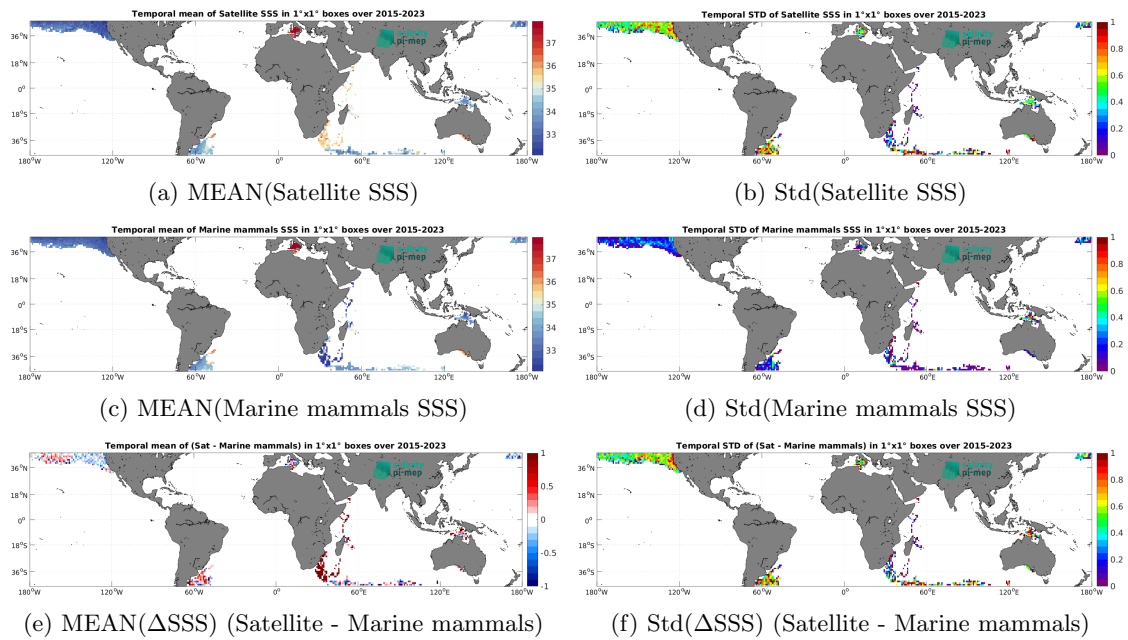
Figure 7: Temporal mean (left) and Std (right) of SSS from SMAP SSS L2 v5.3 (RSS) (top), Marine mammals (middle), and of \Delta SSS (Satellite - Marine mammals). Only match-up pairs are used to generate these maps.
